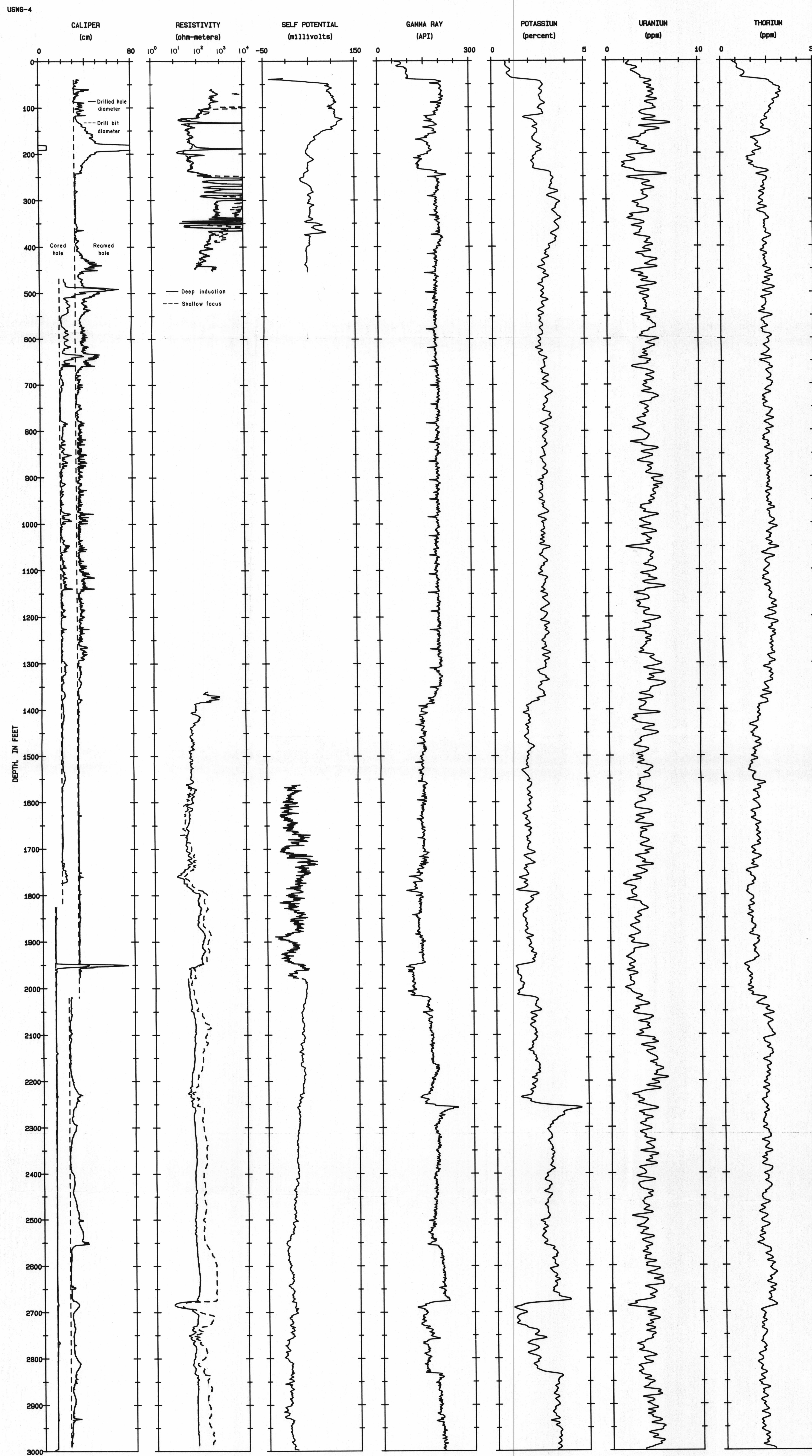
Graphic log showing lithologic, structural, and geophysical features of USW G-4--continued
