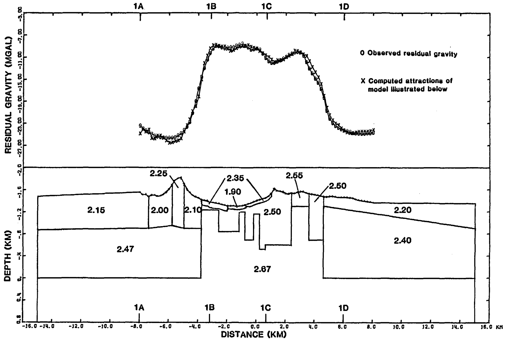
Figure 18.--South-north residual gravity interpretive model line 1. Densities (g/cm 3 ) are based on rock sampling. The profile is located on plate 1. A schematic of the geology is shown in figure 19.
