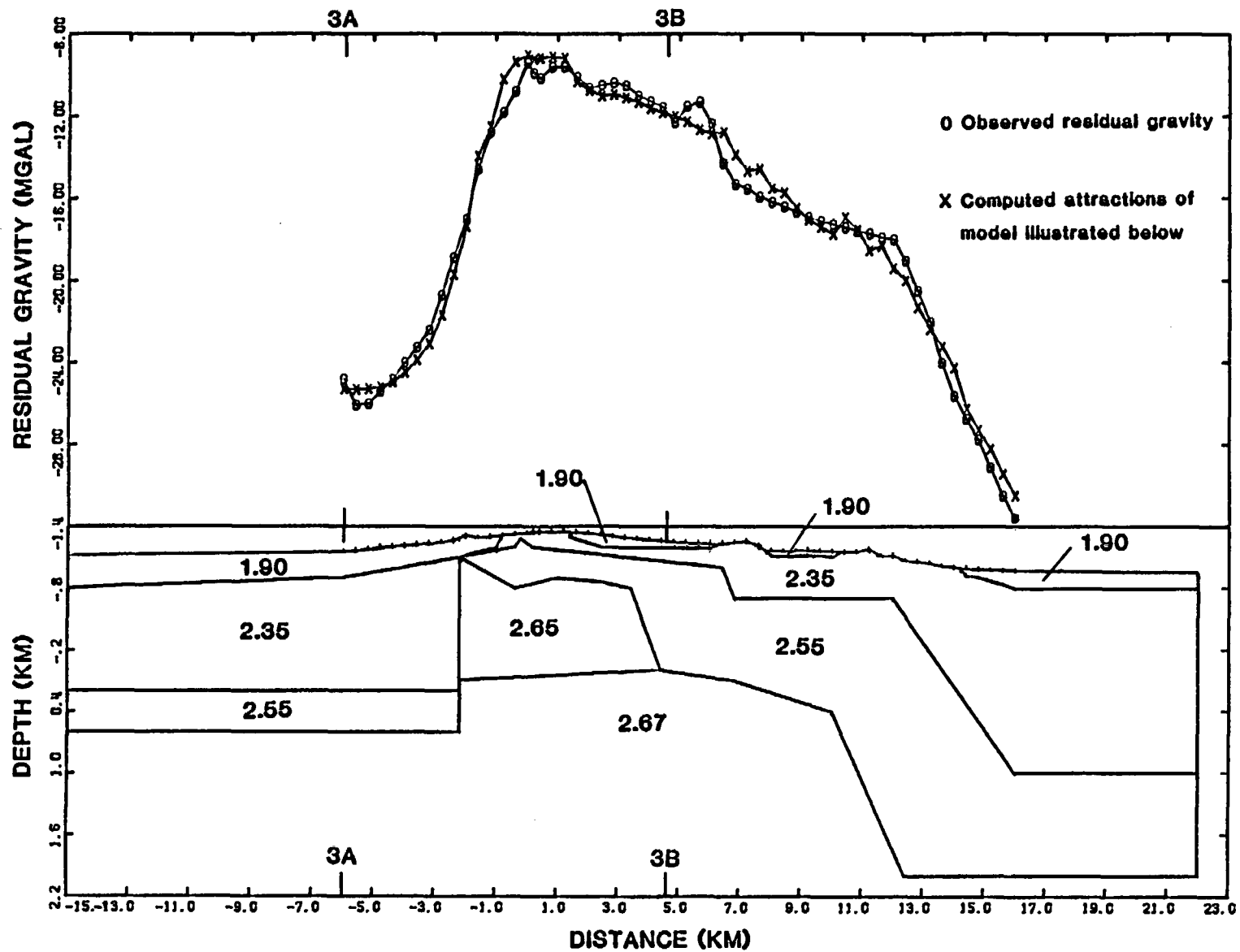
Figure 22.--West-east residual gravity anomaly interpretive model line 3. Densities are in g/cm^3 . The profile is located on plate 1. A schematic of the geology is shown in figure 23.
