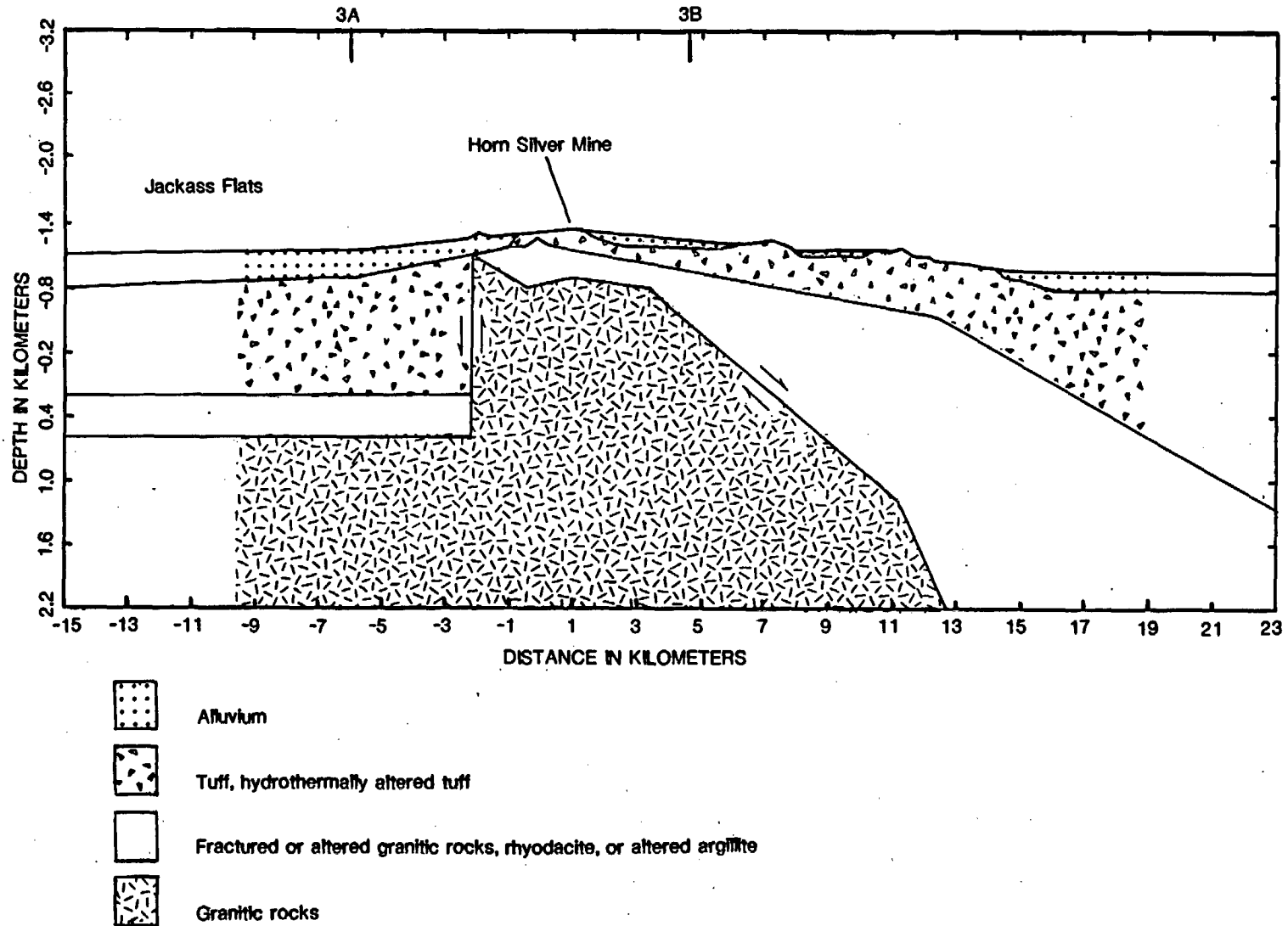
Figure 23.--Schematic of the geology represented in model line 3, figure 22.
