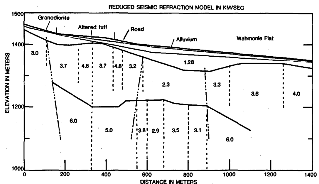
Figure 17.--Seismic refraction model along profile line 4 by L. W. Pankratz (written commun., 1981) and residual gravity anomaly for a density of 2.67 \text{ g/cm}^3 . The profile is located on plate 1.
