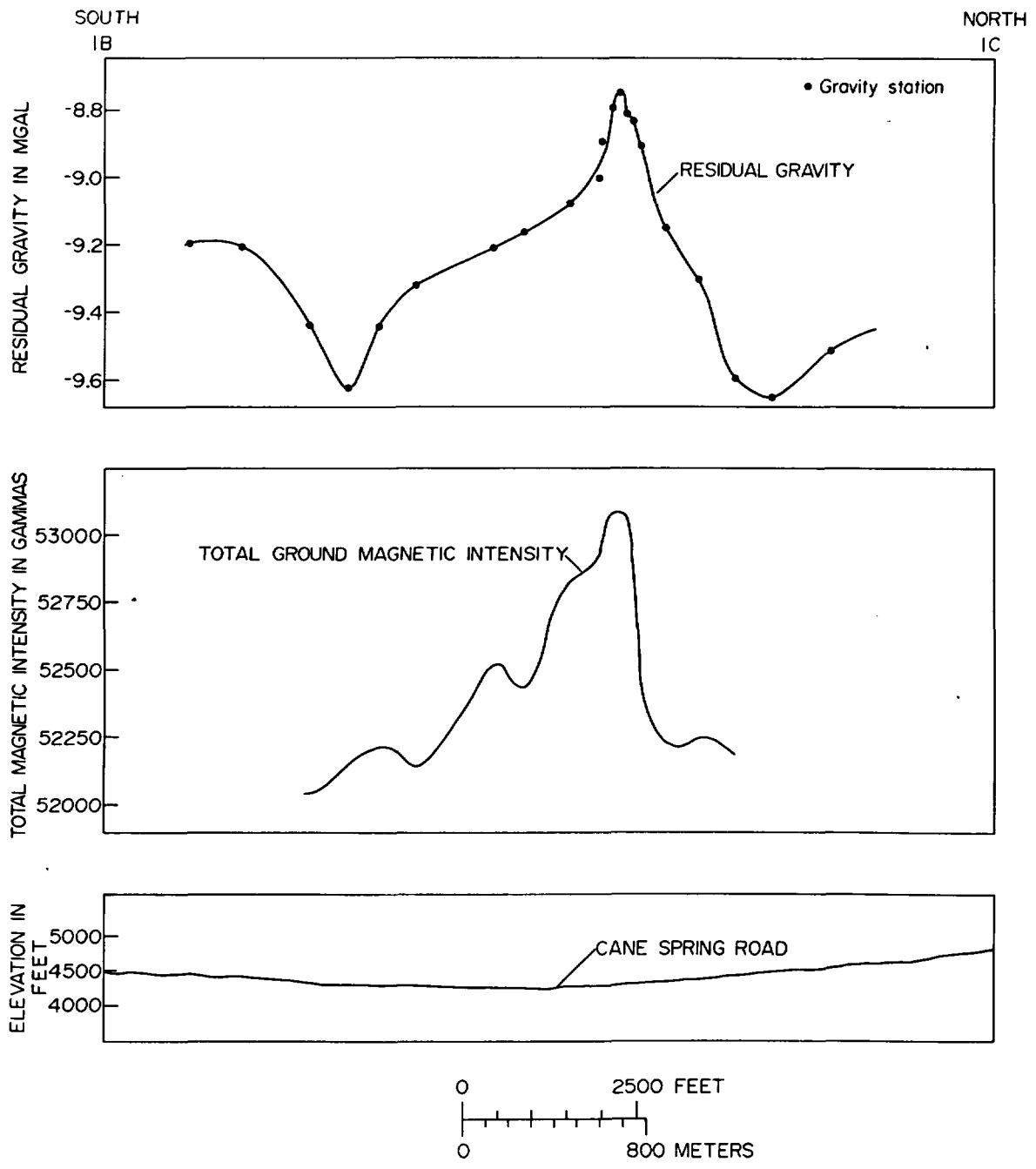
Figure 13.--Detailed south-north residual gravity profile line 1 coincident with a ground magnetic traverse. The profile is located on plate 1.
