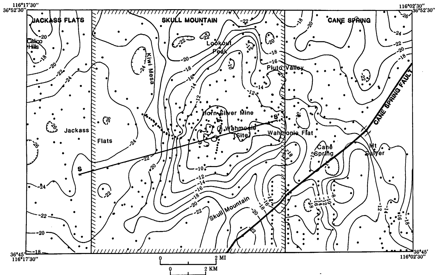
Figure 8.--Residual gravity anomaly contour map of the Skull Mountain and part of the Jackass Flats and Cane Spring 7\frac{1}{2} quadrangles reduced for a density of 2.67 \text{ g/cm}^3 . The contour interval is 2 mGal. Hachures indicate closed gravity lows. Ruled border area is shown in plate 1.
