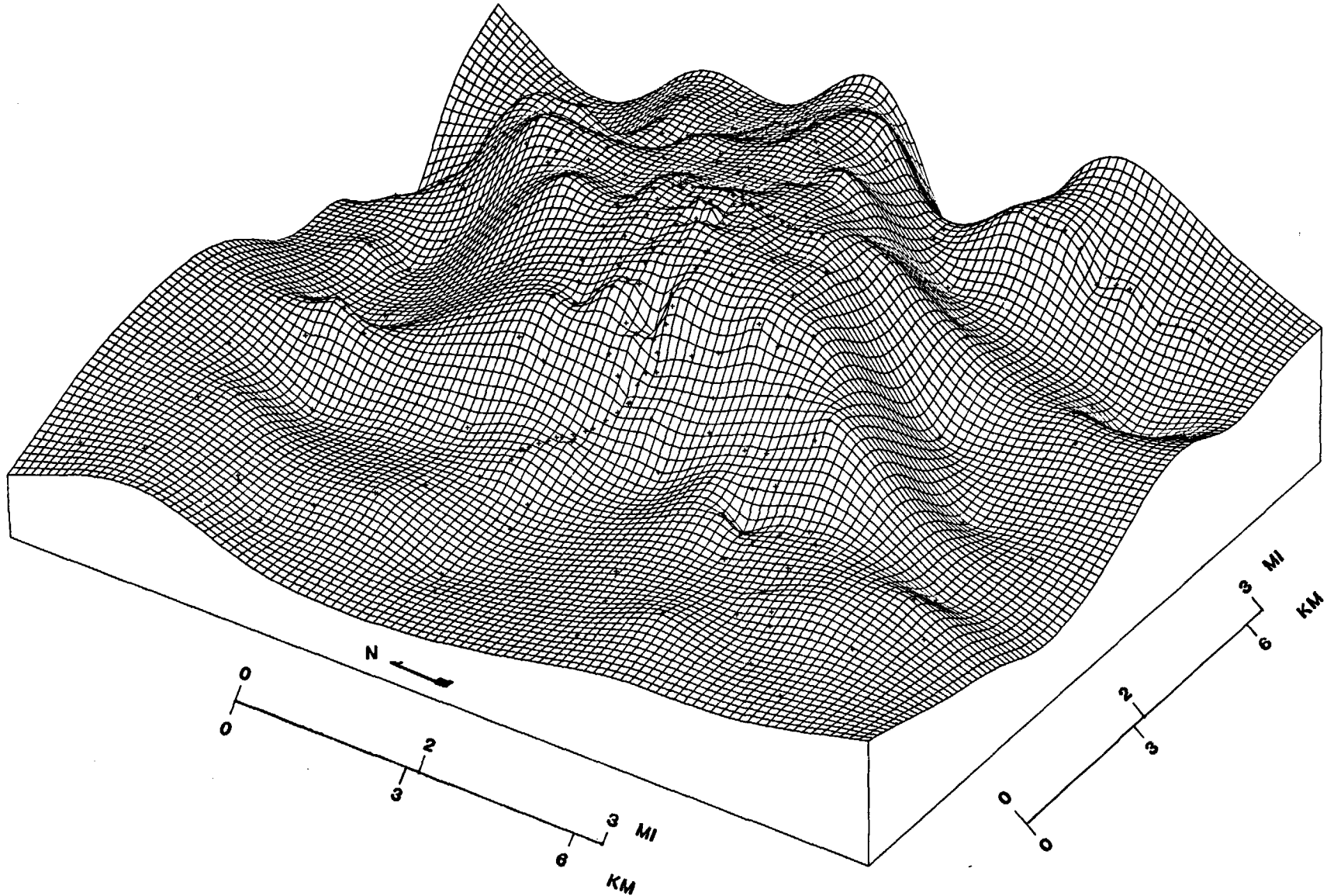
Figure 11.--Three-dimensional mesh perspective view of the residual gravity anomaly field of the Skull Mountain 7\frac{1}{2} quadrangle reduced for a density of 2.67 \text{ g/cm}^3 . The view angle is from the SW. corner of plate 1. Gravity stations are plotted at their correct spatial positions.
