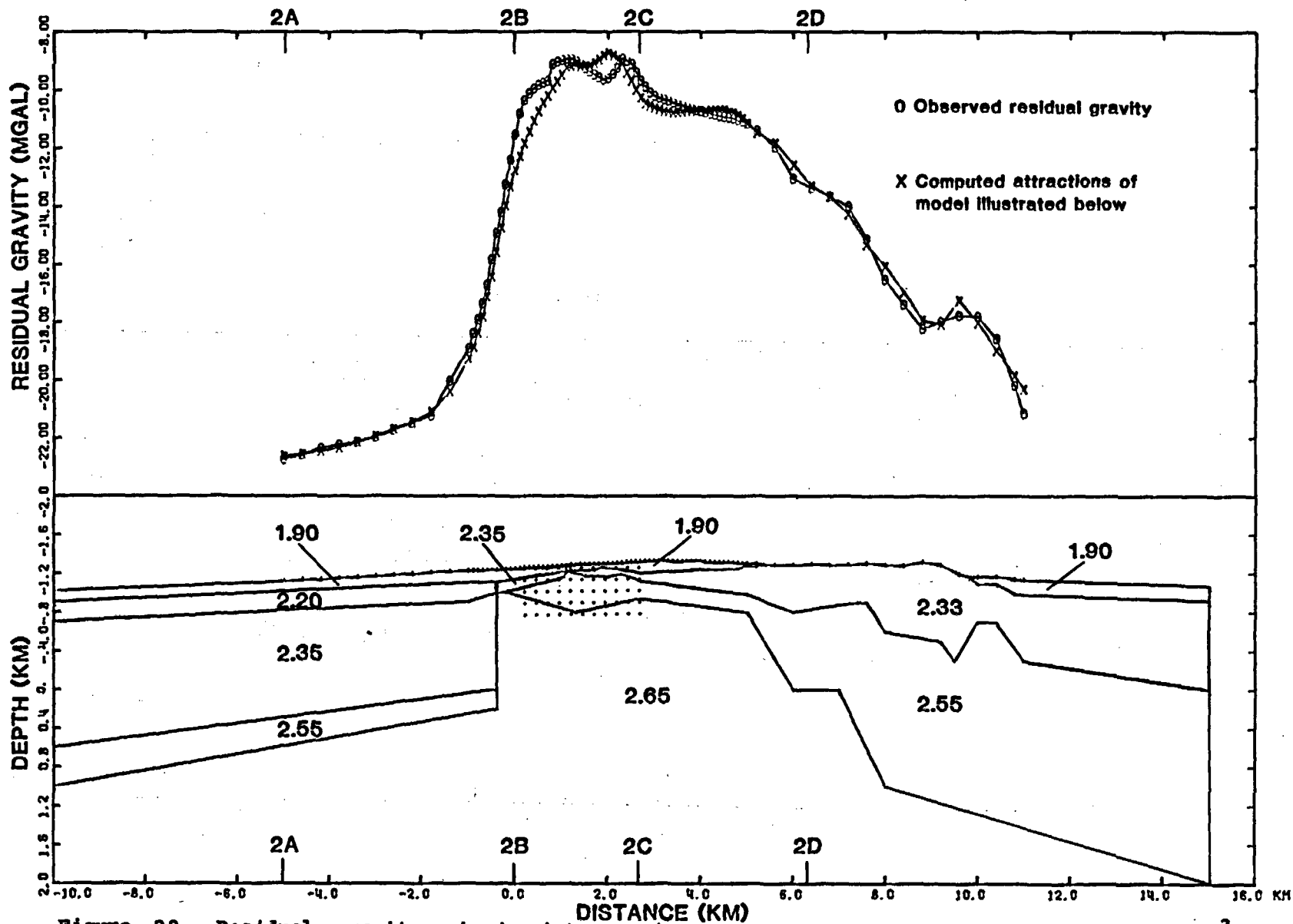
Figure 20.--Residual gravity-seismic interpretive model line 2. Densities are in \text{g/cm}^3 . Stippled area denotes seismic refraction control. The profile is located on plate 1. A schematic of the geology is shown in figure 21.
