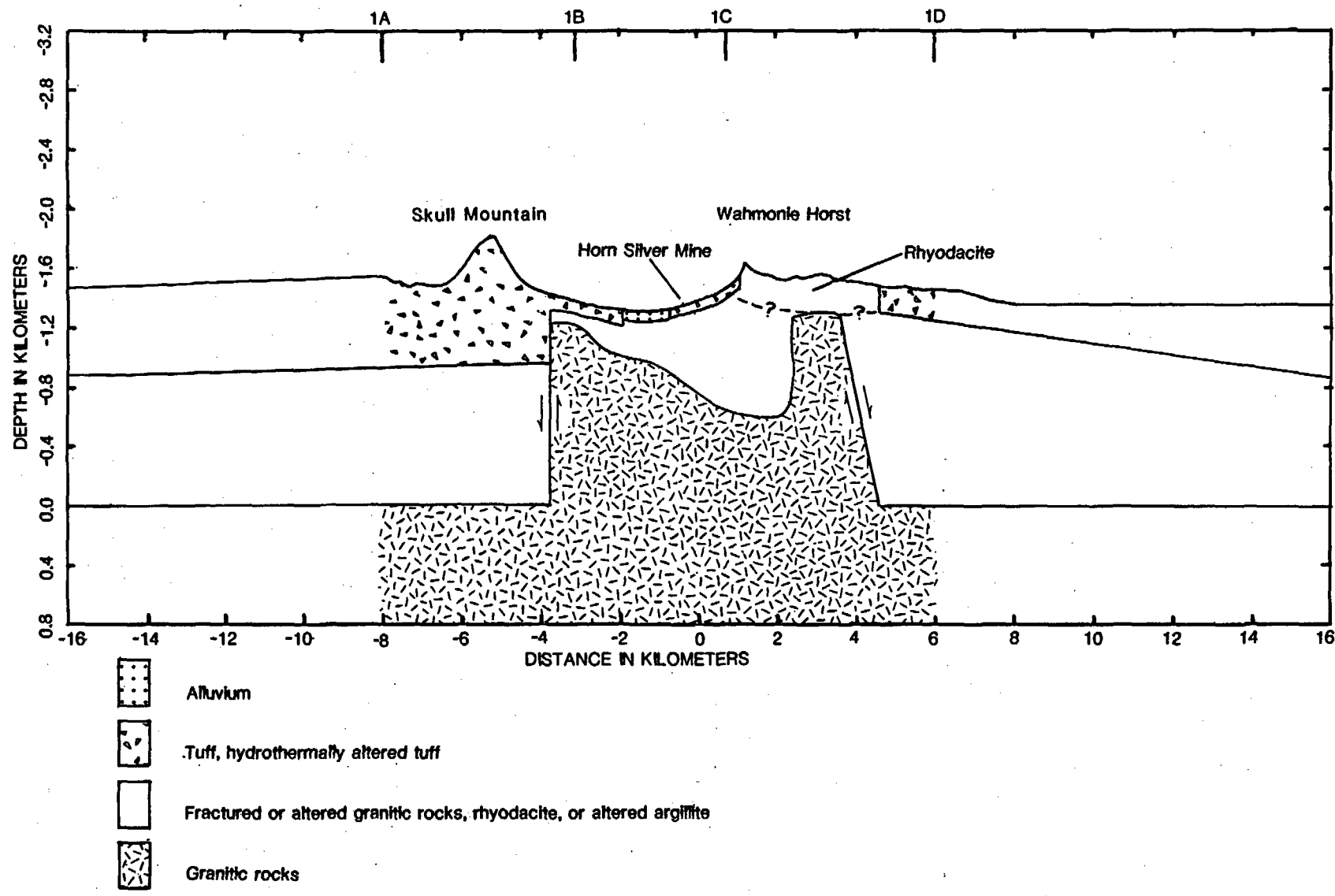
Figure 19.--Schematic of the geology represented in model line 1, figure 18.
