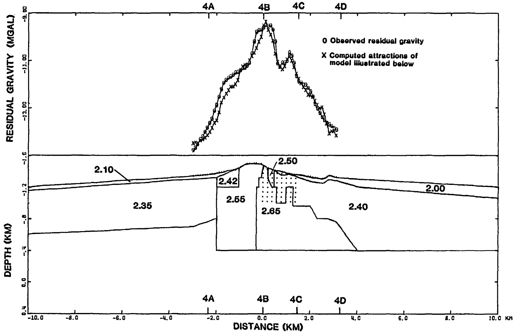
Figure 24.--Residual gravity-seismic interpretive model line 4. Densities are in \text{g/cm}^3 . Stippled area denotes area of seismic refraction control. The profile is located on plate 1. A schematic of the geology is shown in figure 25.
