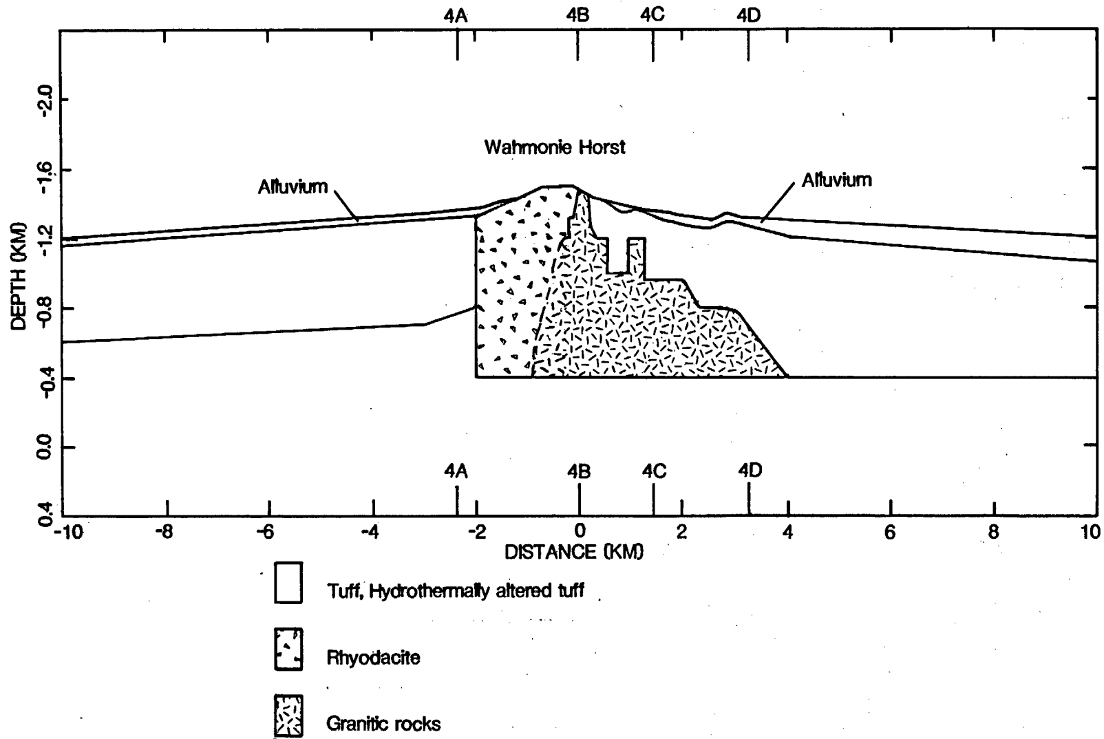
Figure 25.--Schematic of the geology represented in model line 4, figure 24.
