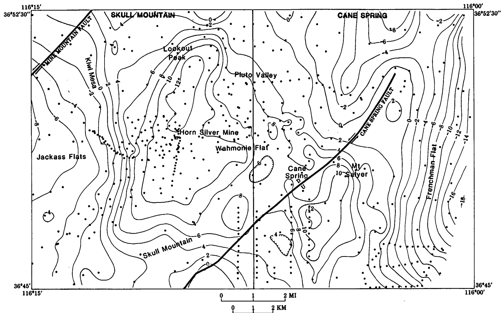
Figure 10.--Residual gravity anomaly map of the Skull Mountain and Cane Spring 7\frac{1}{2}' quadrangles reduced for a density of 2.30 \text{ g/cm}^3 . The contour interval is 2 mGal. Hachures indicate closed gravity lows.
