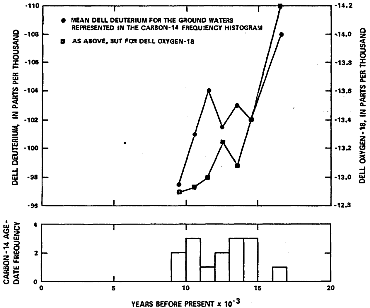
Figure 15.--Carbon-, hydrogen-, and oxygen-isotope data for water in tuff and tuffaceous valley fill and their relationship to climate change.
