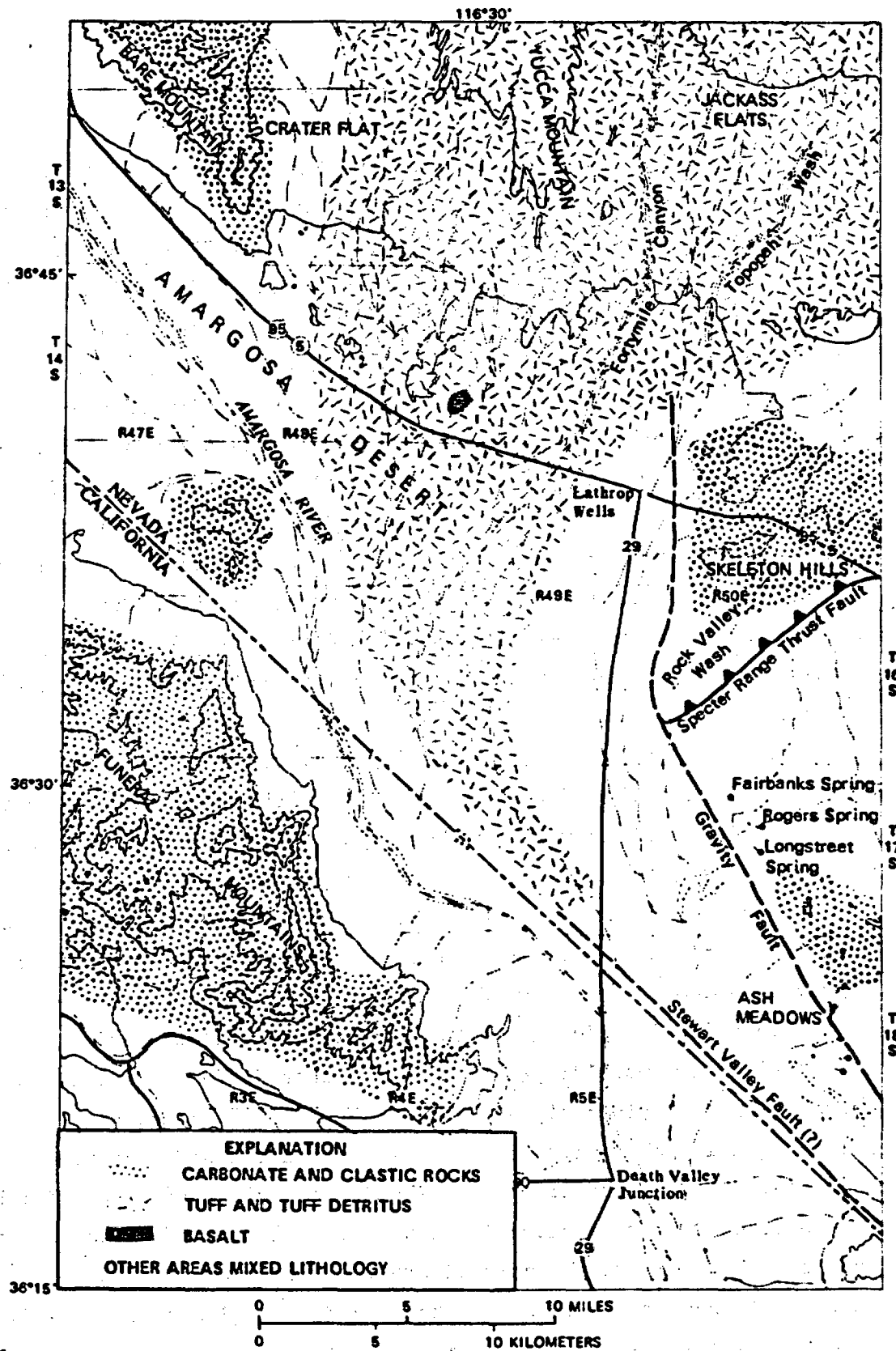
Figure 1.--West-central Amargosa Desert and vicinity.
