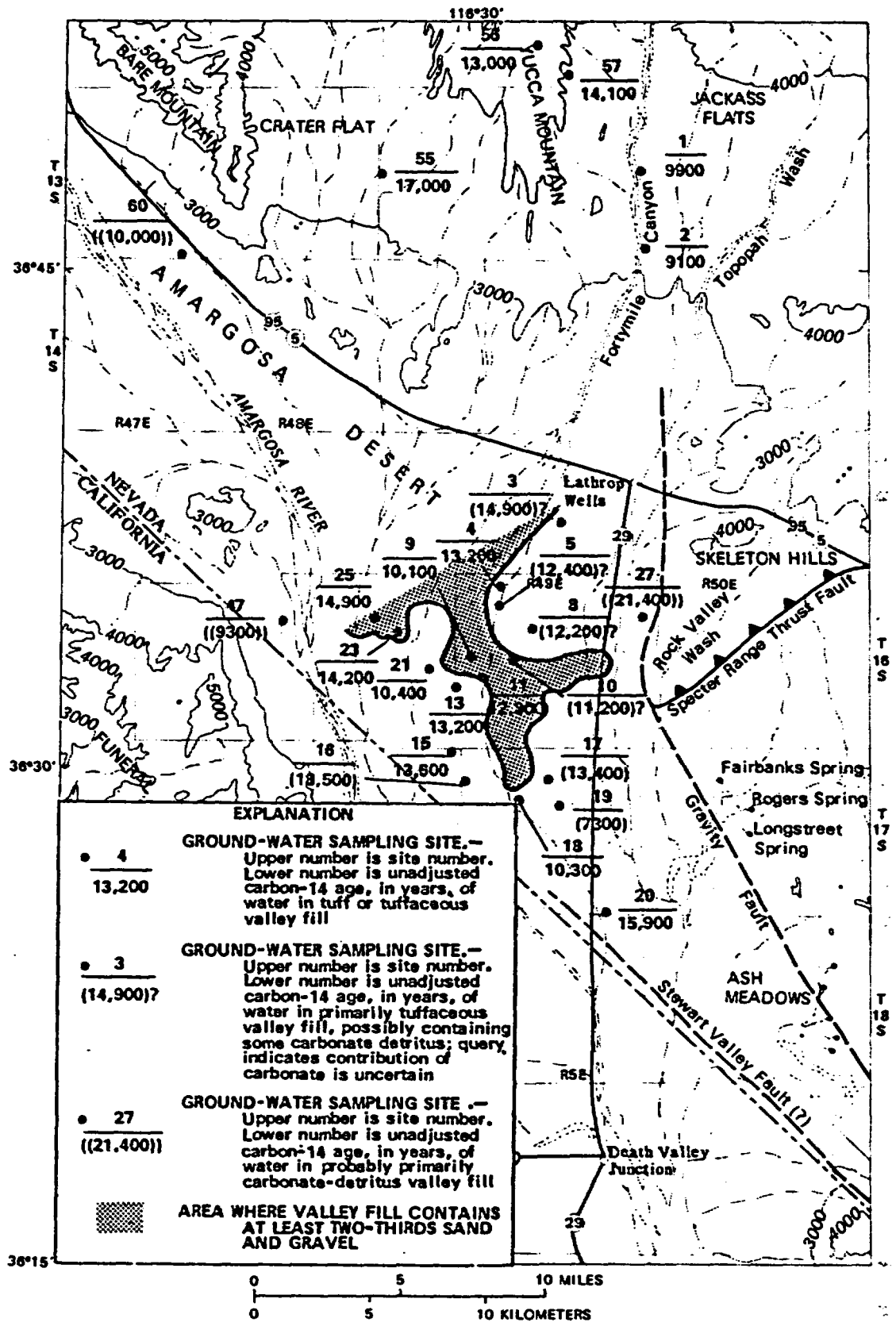
Figure 14.--Unadjusted carbon-14 age of ground water in relation to major surface drainageways and relative permeability.
