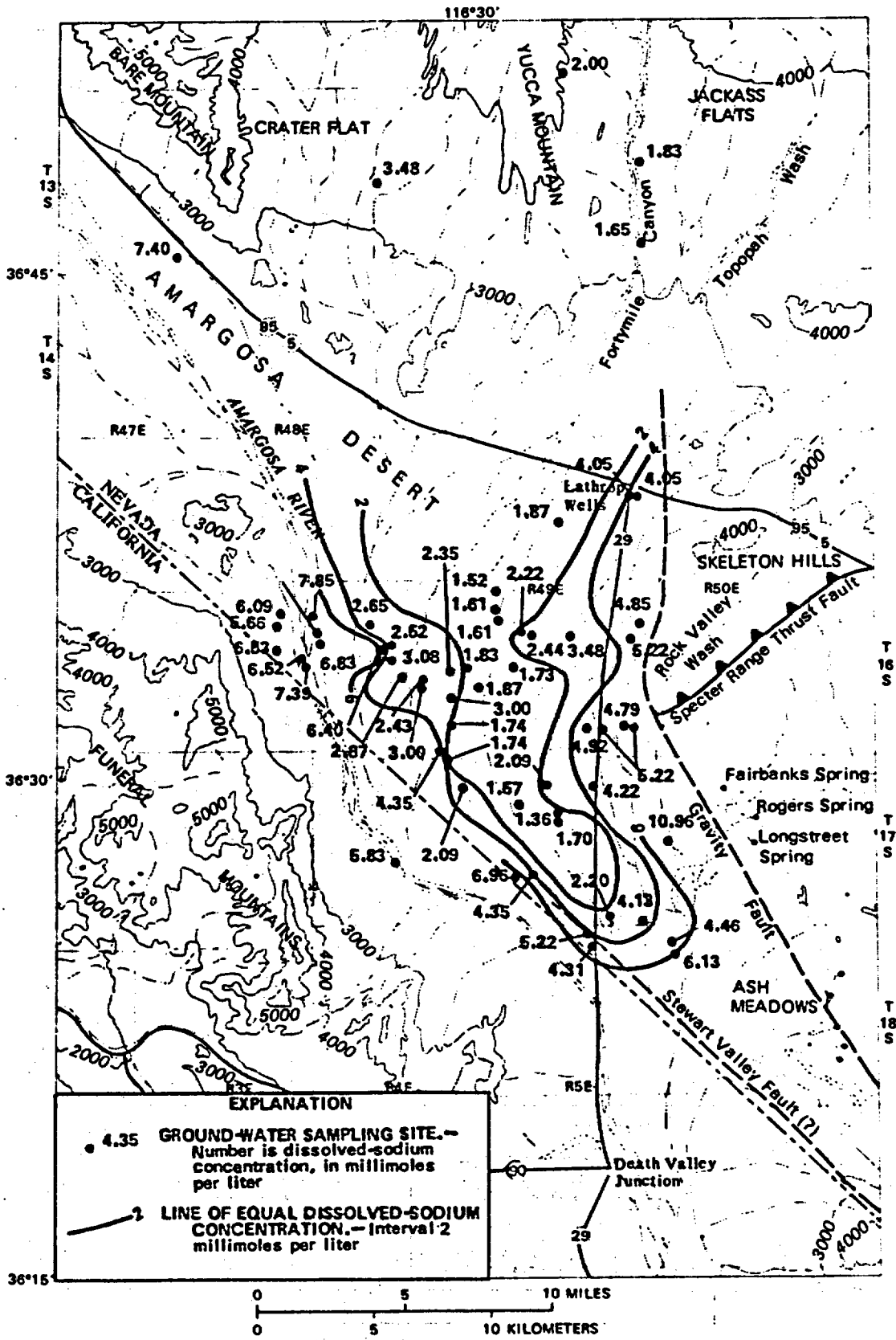
Figure 4.--Dissolved sodium ( \text{Na}^+ ) in ground water.
