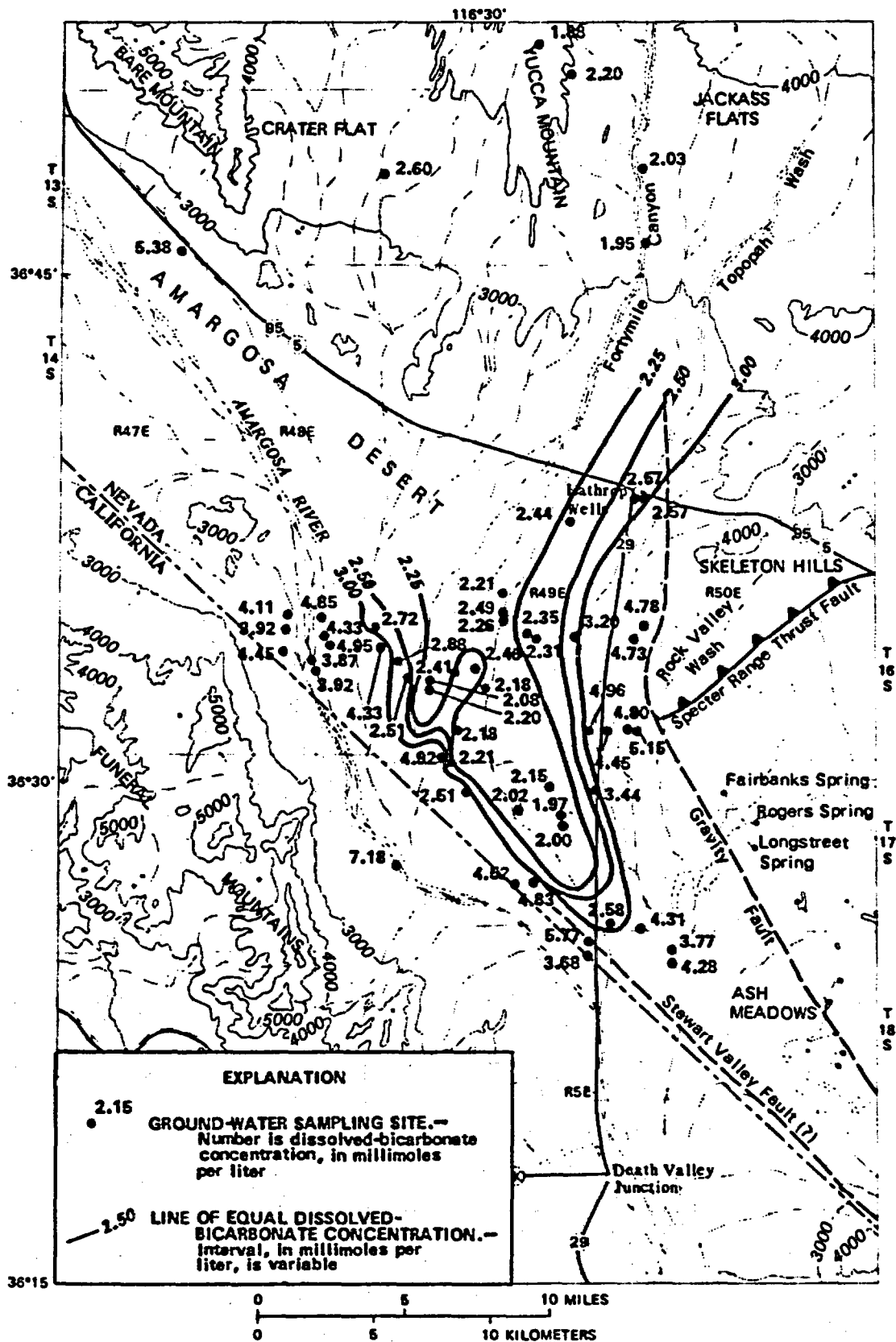
Figure 6.--Dissolved bicarbonate ( \text{HCO}_3^- ) in ground water.
