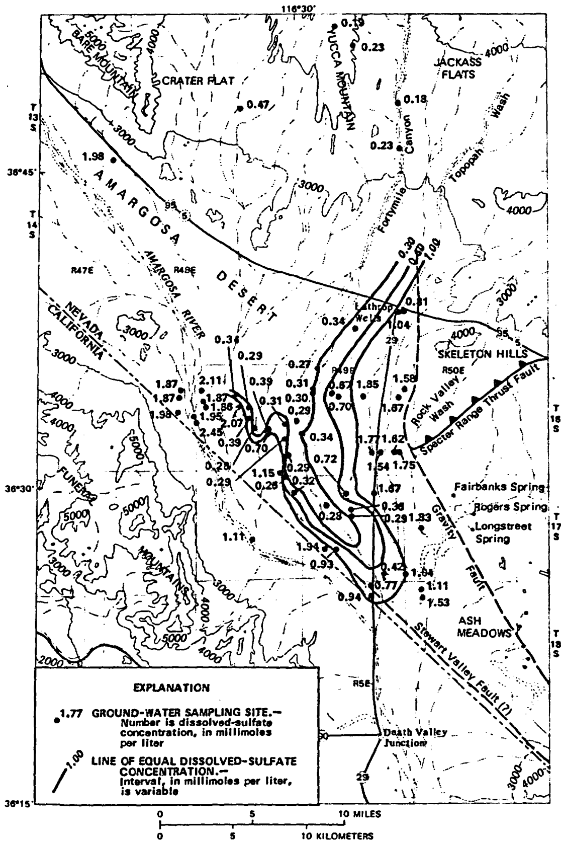
Figure 7.--Dissolved sulfate ( \text{SO}_4^{2-} ) in ground water.
