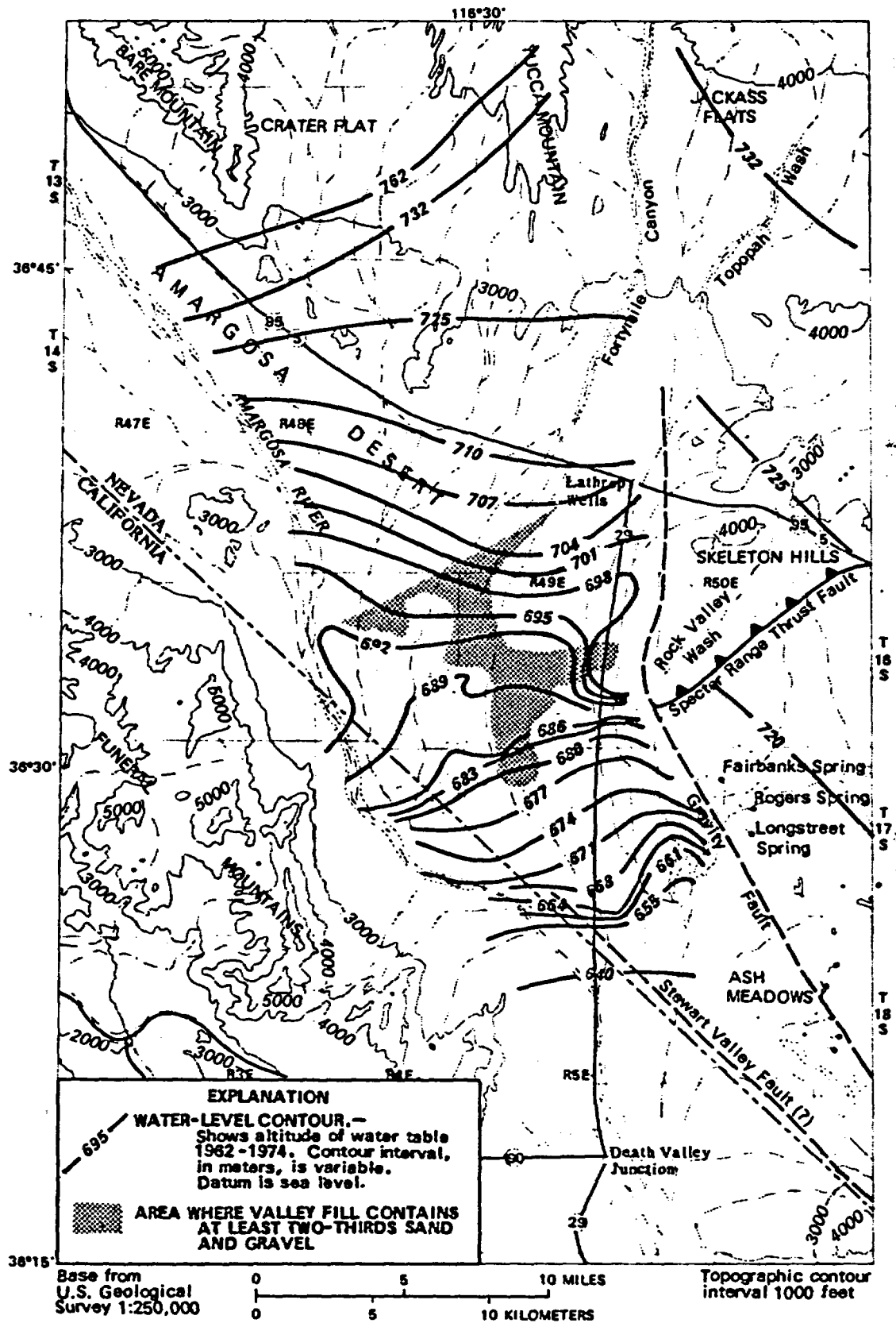
Figure 2.--Water-level altitudes (modified from Walker and Eakin, 1963).
