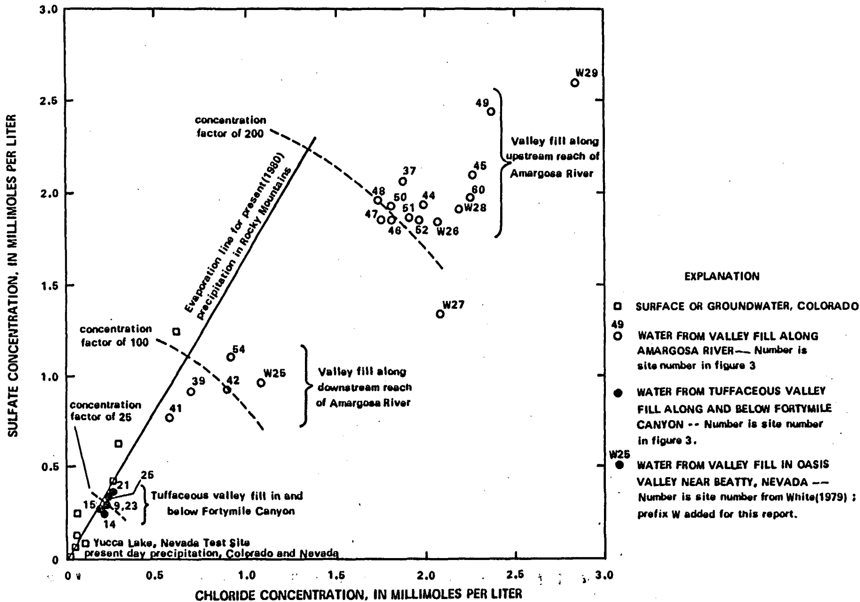
Figure 12.--Chloride and sulfate in precipitation and selected ground and surface waters, Colorado and Nevada.
