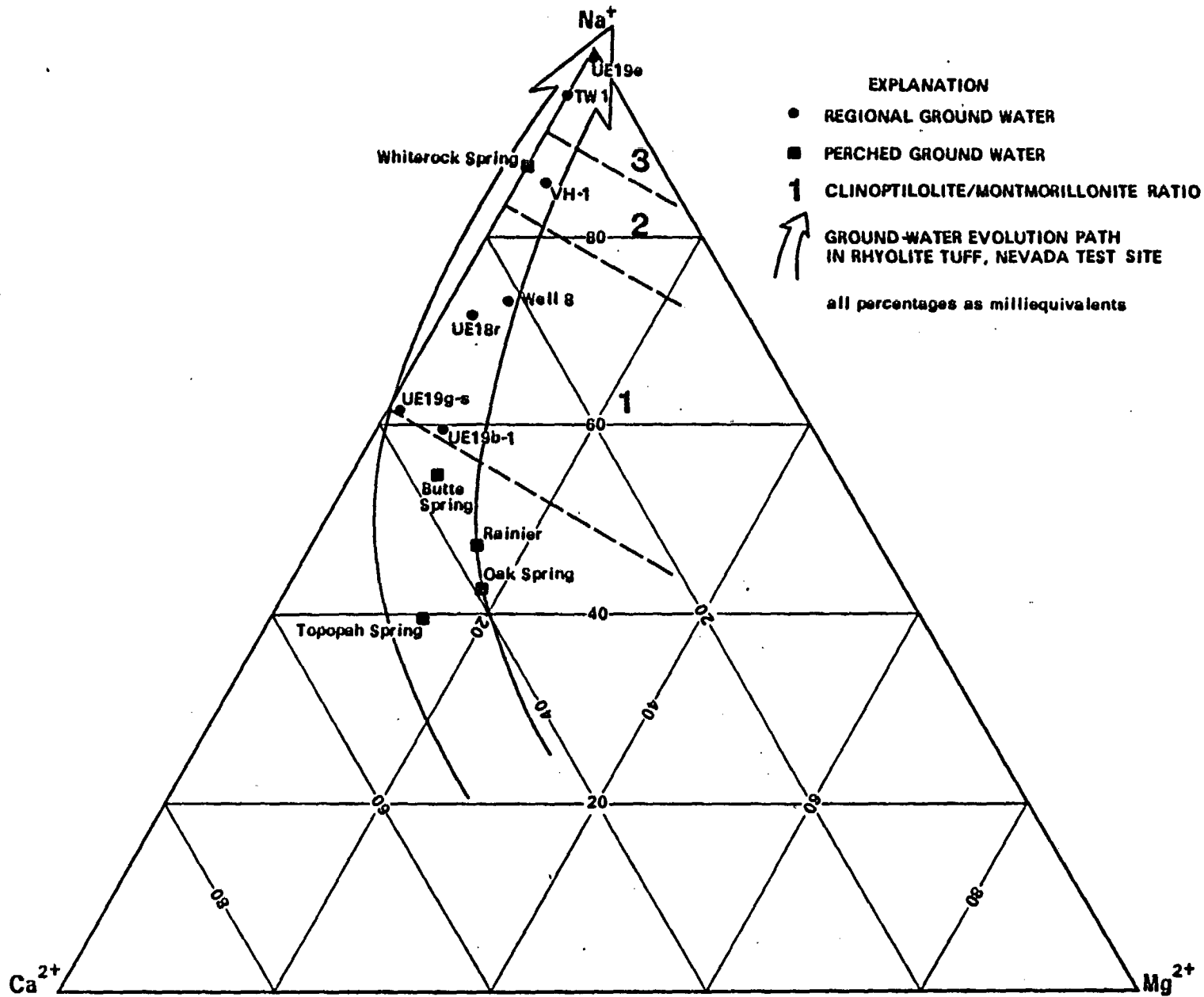
Figure 8.--Evolution of water in tuff, Nevada Test Site.
