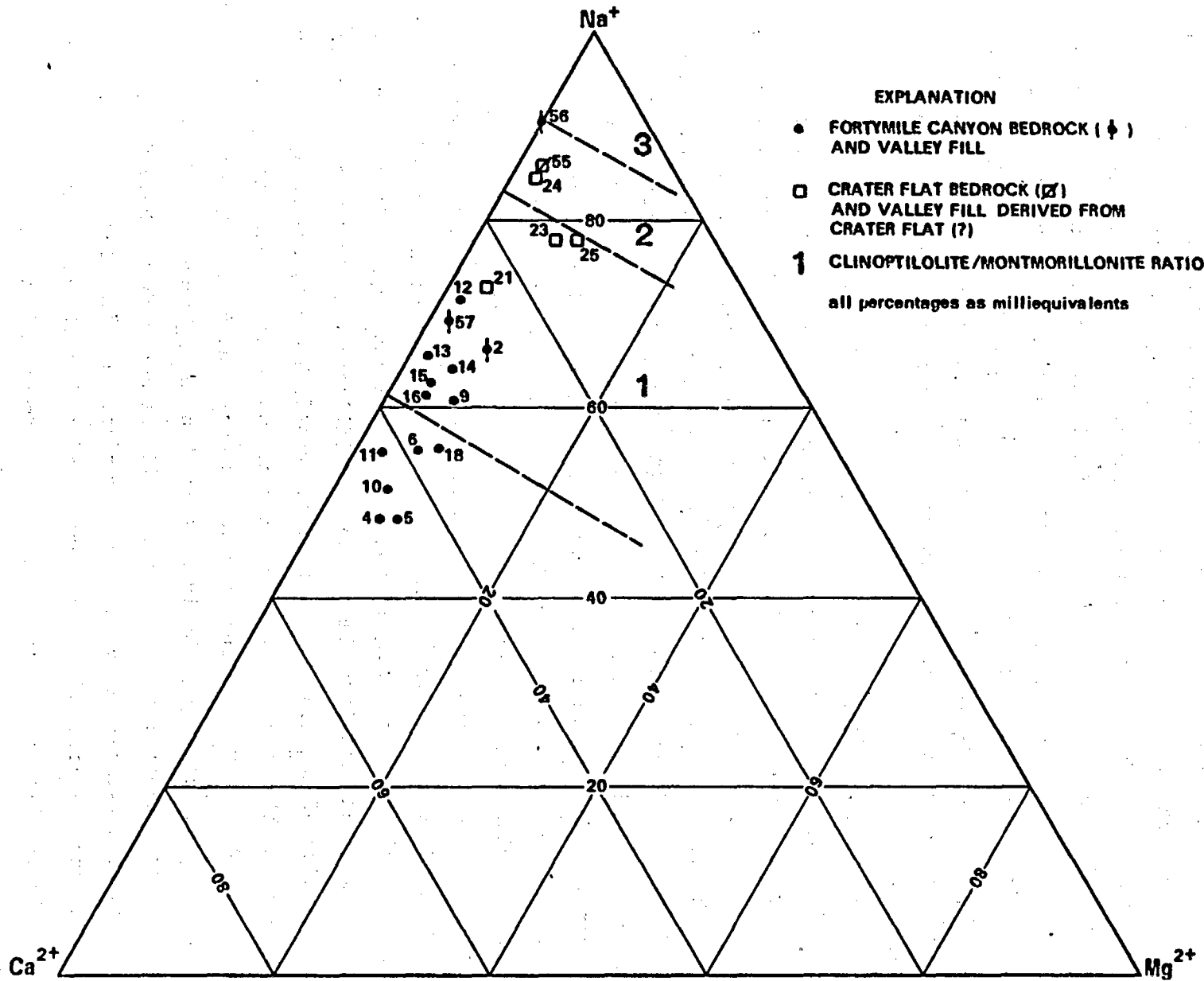
Figure 9.--Composition of water in tuffaceous valley fill.
