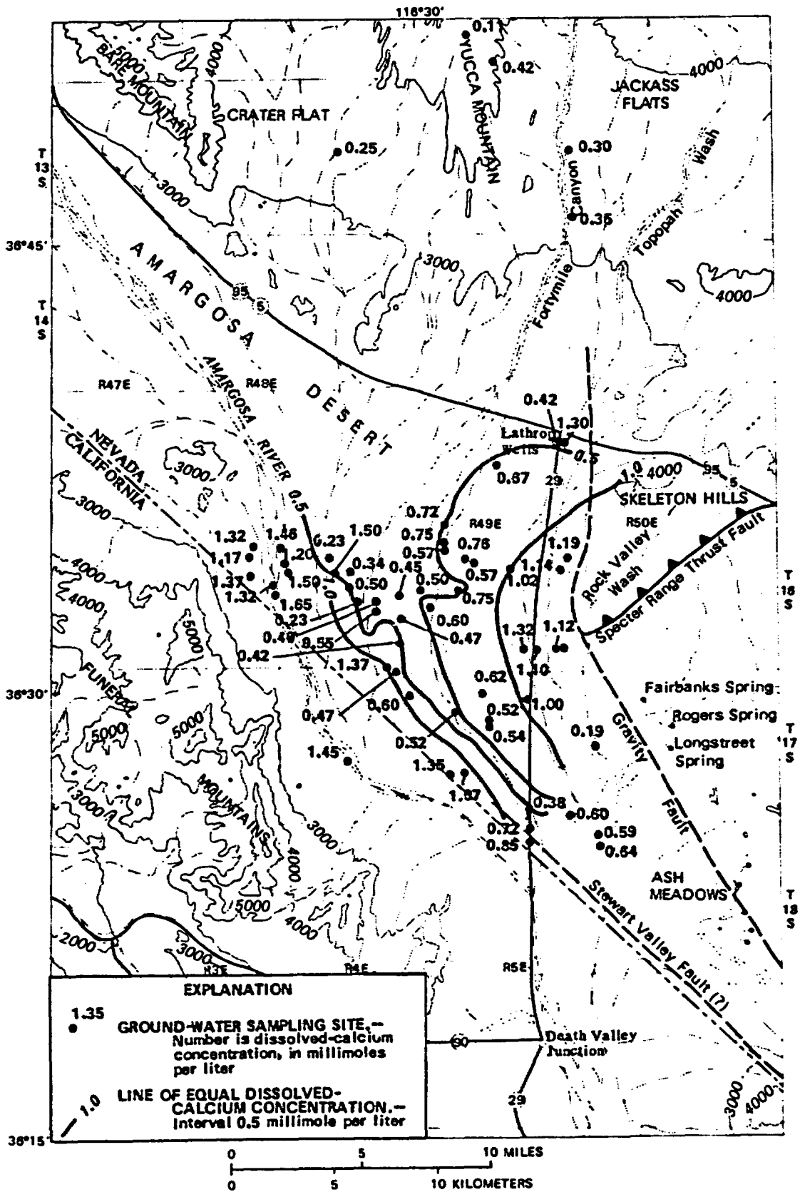
Figure 5.--Dissolved calcium ( \text{Ca}^{2+} ) in ground water.
