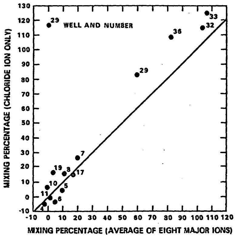
Figure 11.--Comparison of mixing percentage calculated by two methods.
