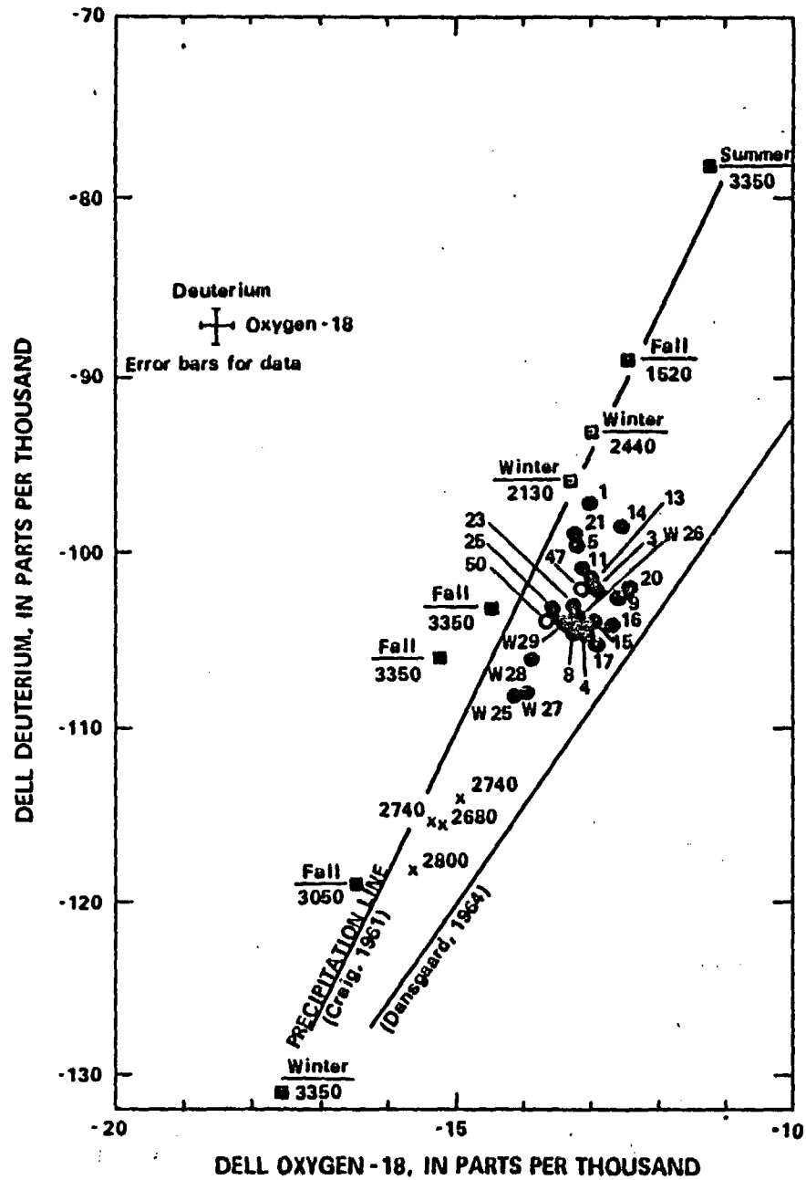
Figure 13.—Hydrogen and oxygen isotopes in precipitation and selected ground and surface waters, Colorado and Nevada.
