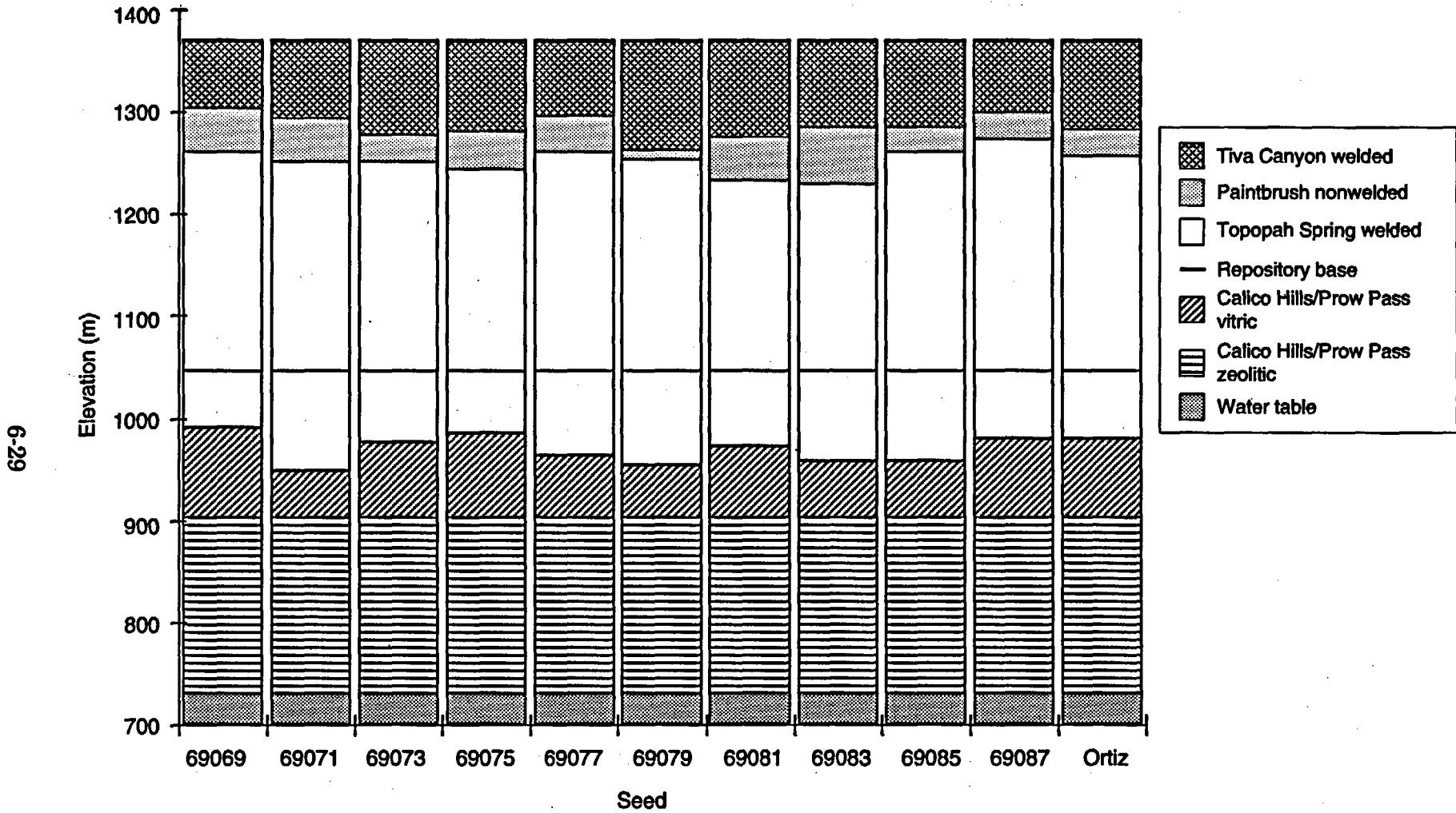
Figure 6-15. Ten simplified stochastic realizations of stratigraphic column 6 extracted from the three-dimensional indicator simulations. Note the absence of the Topopah Spring basal vitrophyre, the Prow Pass welded, and the Bullfrog units from this column. The thermal/mechanical stratigraphy for column 6 of Ortiz et al. (1985) is at the right.
