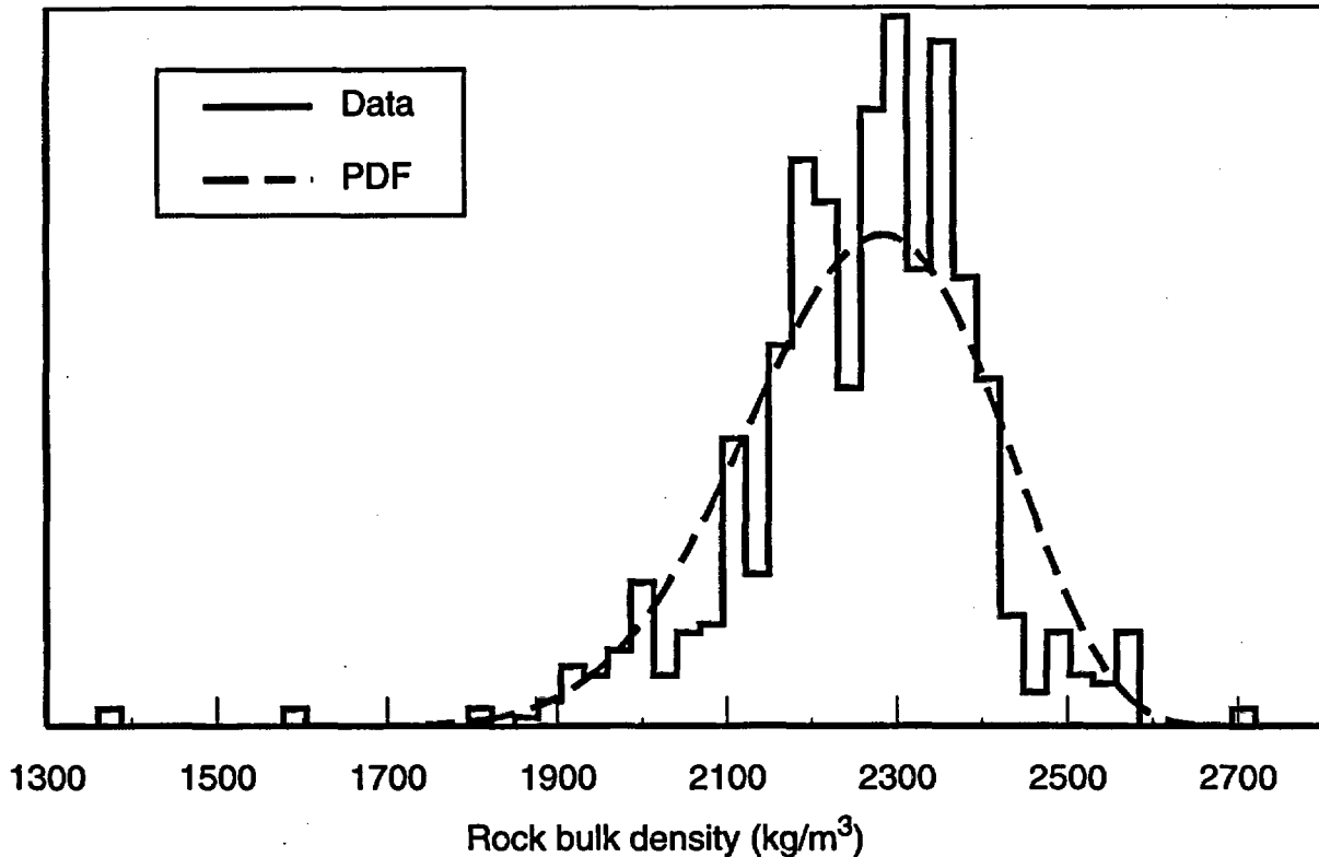
Figure 7-4. PDF fit to the rock bulk density data for unit 3 (Topopah Spring welded).
