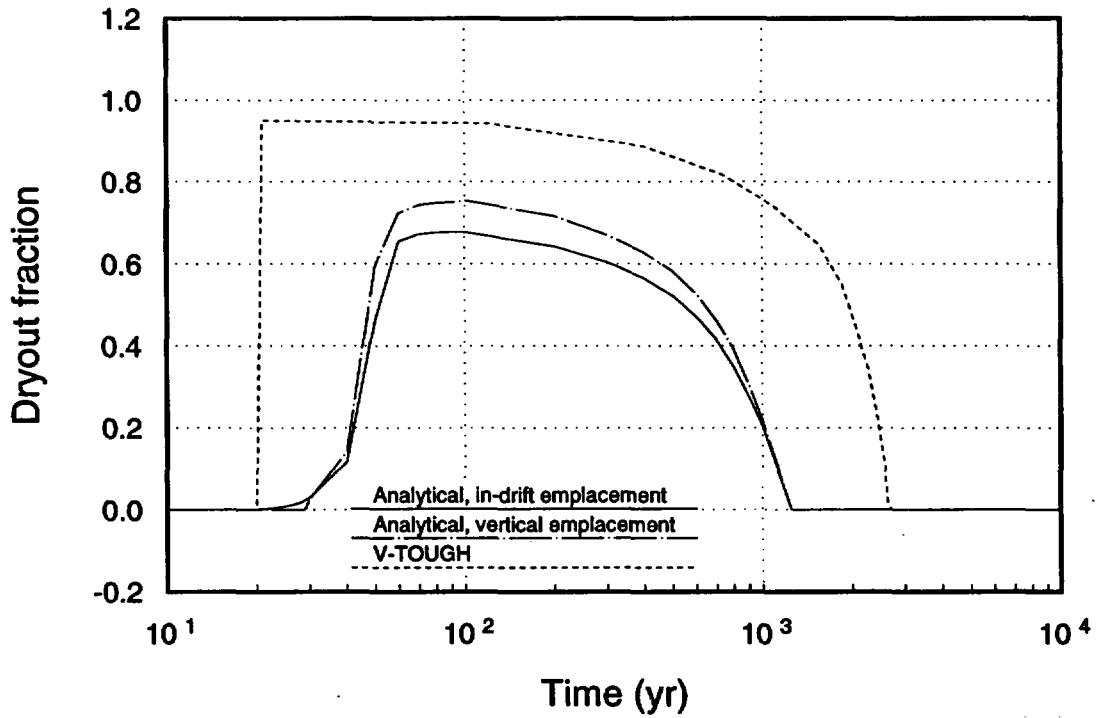
Figure 10-11. Fraction dry for 57-kW/acre cases.
