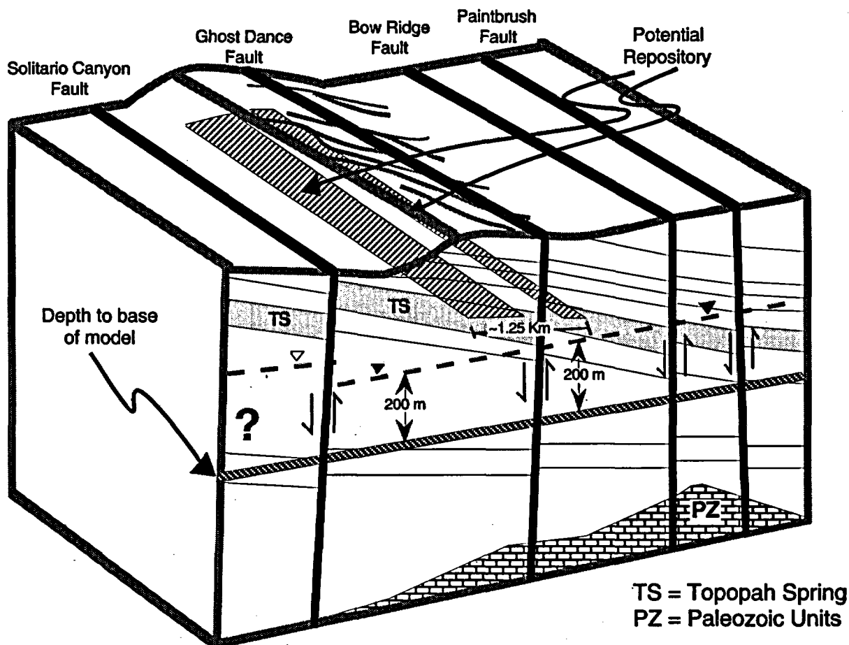
Figure 11-3. A schematic diagram showing the three-dimensional relationship among the potential repository, the stratigraphic units, and the major faults. Also shown is the depth of the base of the saturated-zone model developed for TSPA-93.
