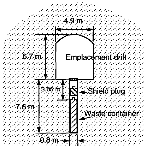
Figure 4-3. Borehole-emplacment configuration.
