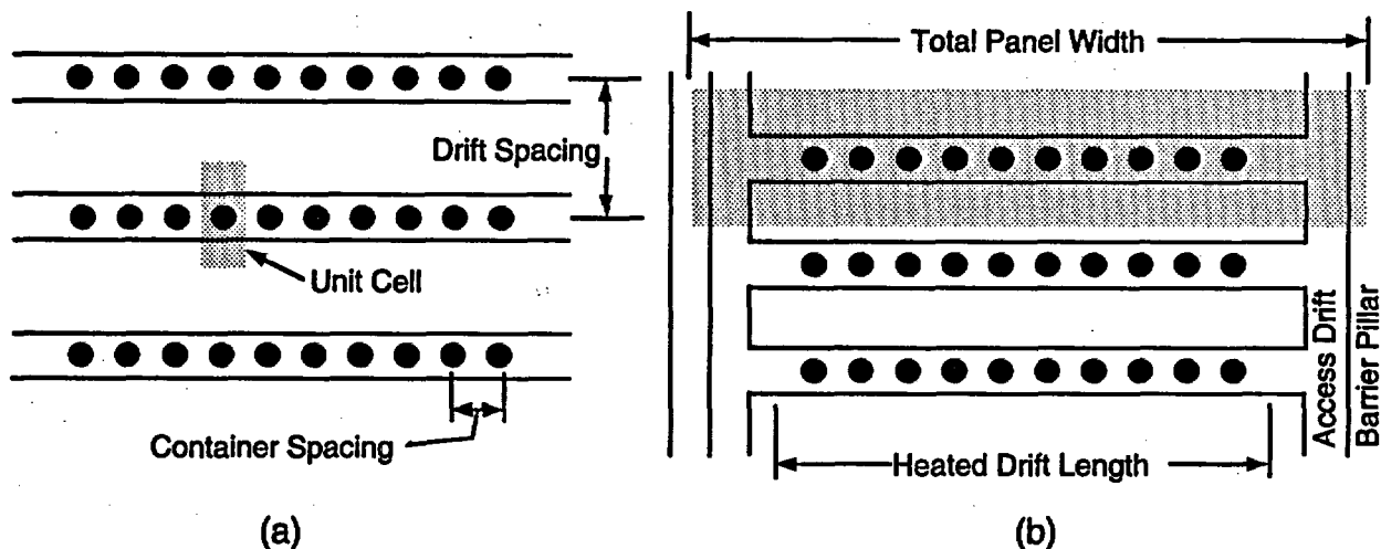
Figure 10-5. (a) Representation of unit cell used to calculate LAPD; (b) Heated drift length used to calculate design-basis areal power density.
