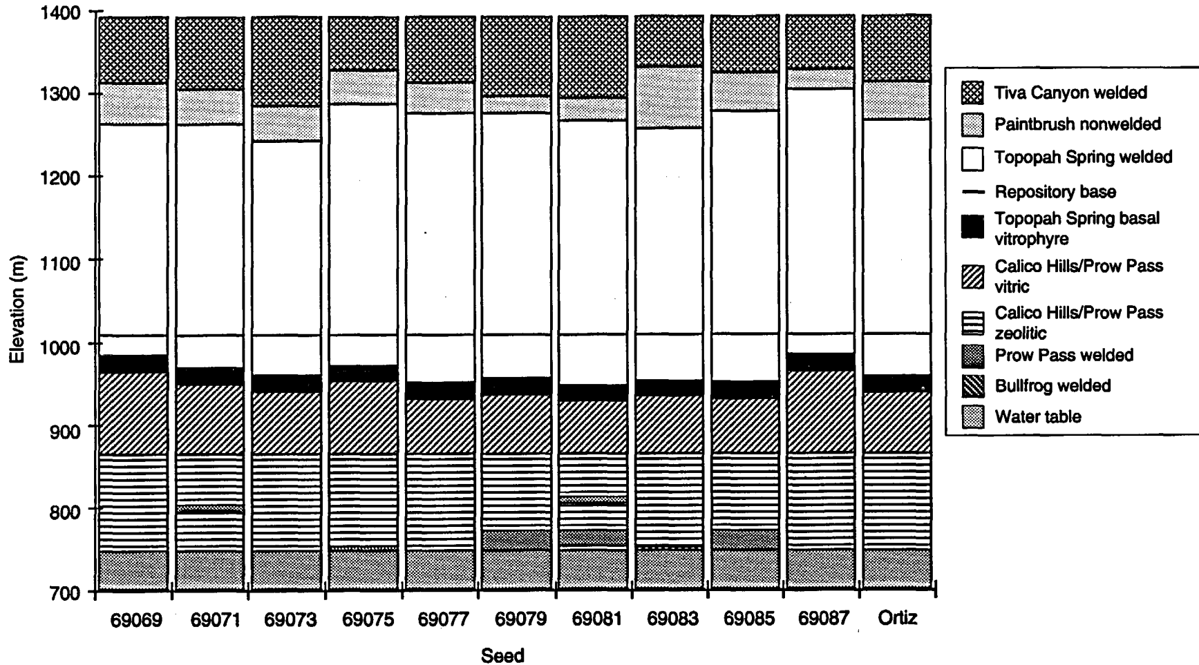
Figure 6-12. Ten simplified stochastic realizations of stratigraphic column 3 extracted from the three-dimensional indicator simulations. Note the appearance of the Prow Pass welded unit twice in simulation 69081, and the presence of the Bullfrog welded only in simulation 69083. The approximately equivalent thermal/mechanical stratigraphy for column 3 of Ortiz et al. (1985) is at the right.
