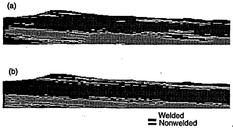
Figure 6-6. Representative west-to-east cross-section of Yucca Mountain illustrating the tendency of simulated welded and nonwelded lithologies to pinch and swell and to interfinger in a more complex fashion than is believed reasonable based on field observations. (a) Profile simulated directly using the anisotropy ratios from Table 6-1. (b) The same profile simulated by adjusting anisotropy ratio 2 to 0.025 (40:1).
