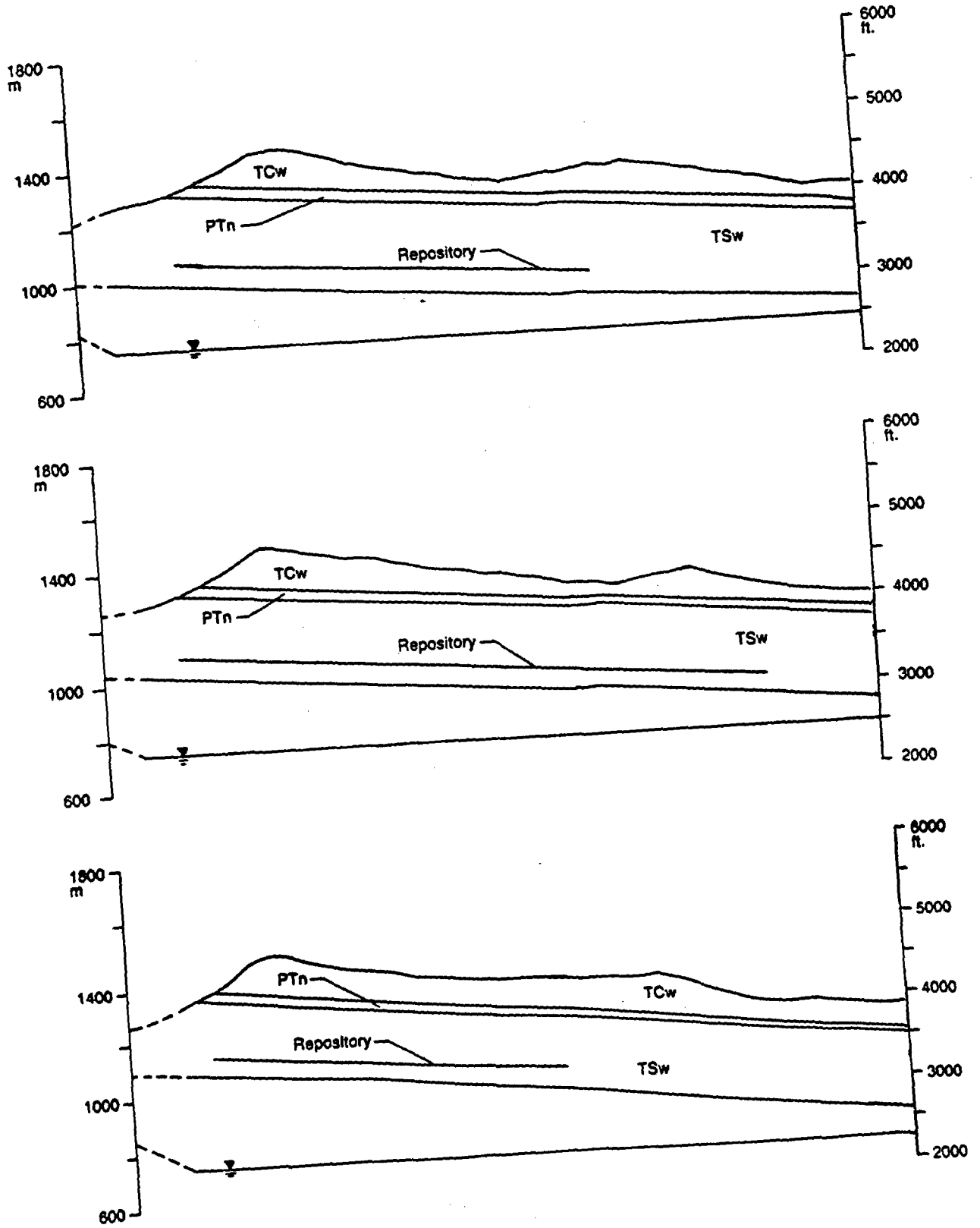
Figure 12-3. Geometry of the three modeled cross sections. Top: N765000; middle: N762500; Bottom: N760000.
