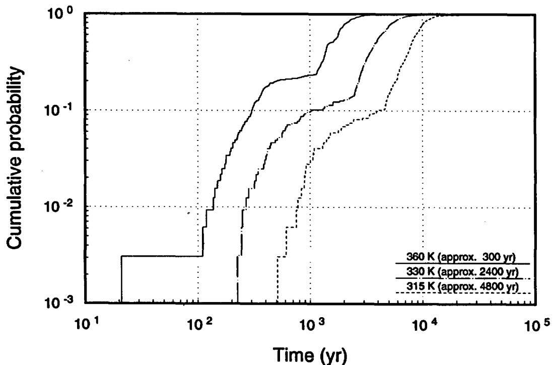
Figure 12-11. ^{14}\text{C} travel-time distributions for TSPA-91.
