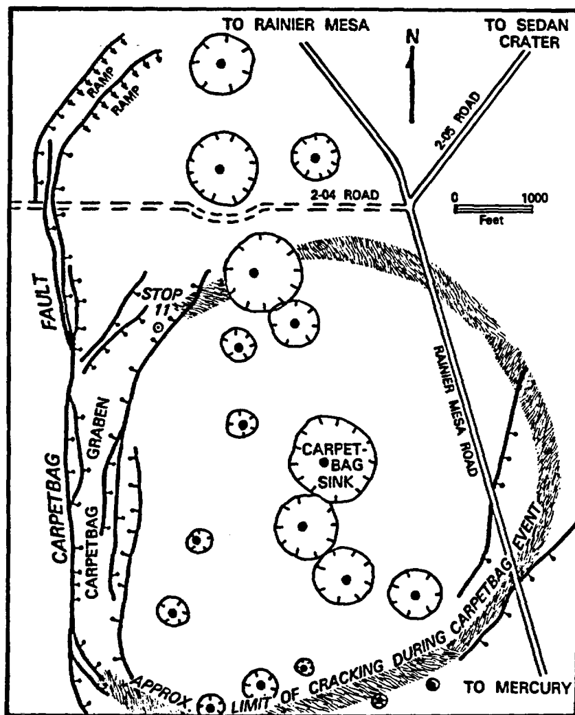
Fig. 17. Carpetbag fault system (Stop 11).
