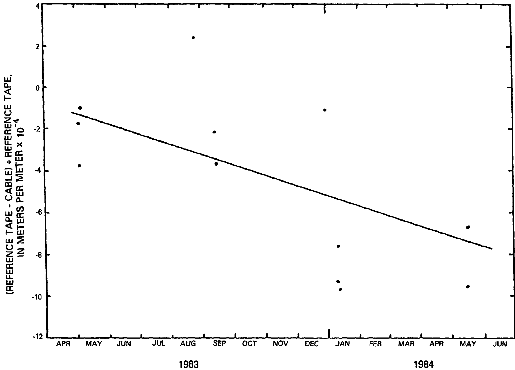
Figure 3.--Correction factor versus time for multiconductor cable.
