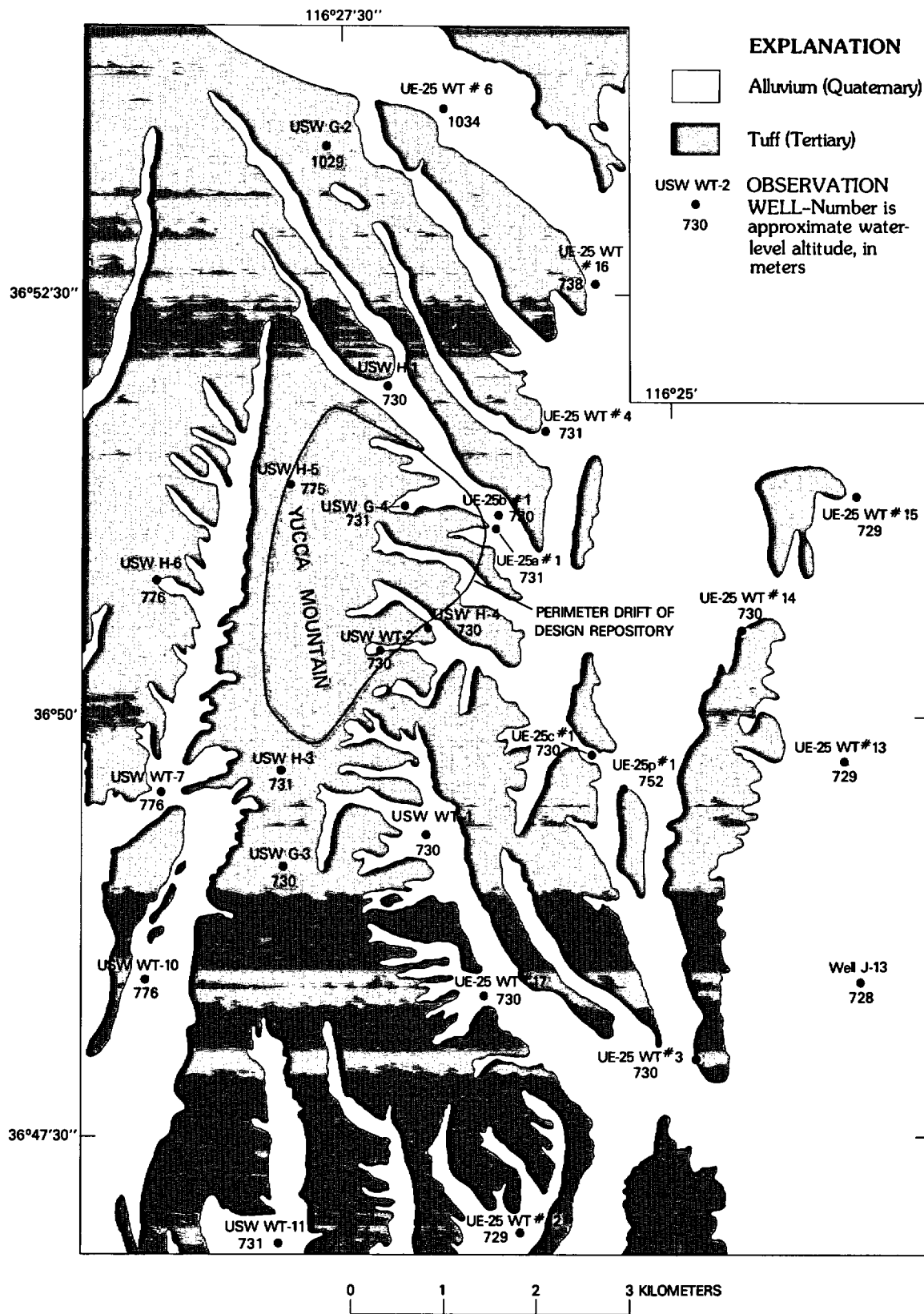
Figure 2.--Locations of wells and water-level altitudes in the vicinity of Yucca Mountain (modified from Robison, 1984, 1986).
