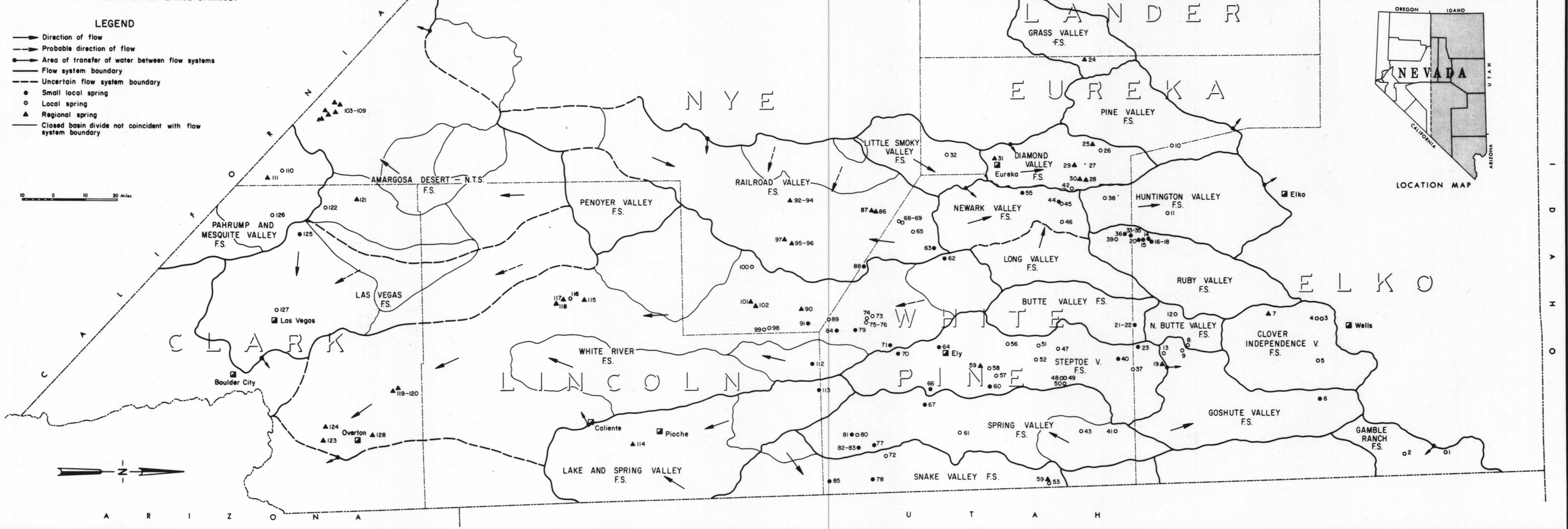
PLATE II. MAP OF FLOW SYSTEMS IN THE CARBONATE ROCK PROVINCE AND THE LOCATION OF LARGE SPRINGS.
