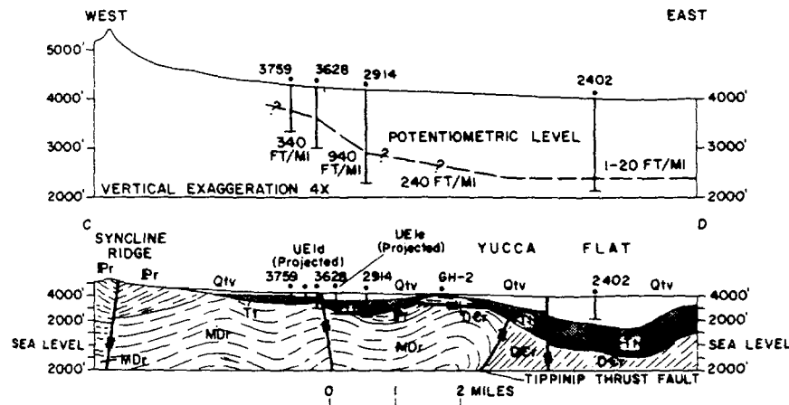
Figure 5. Geologic and hydrologic cross section, west-central Yucca Flat. Line of section shown on Figure 4. QIV, Quaternary and Tertiary valley fill; Tt, Tertiary tuff; Pr, Pennsylvanian carbonate rocks; MDr, Mississippian and Devonian clastic rocks (Eleana Formation); DCr, Devonian to Cambrian carbonate rocks.
