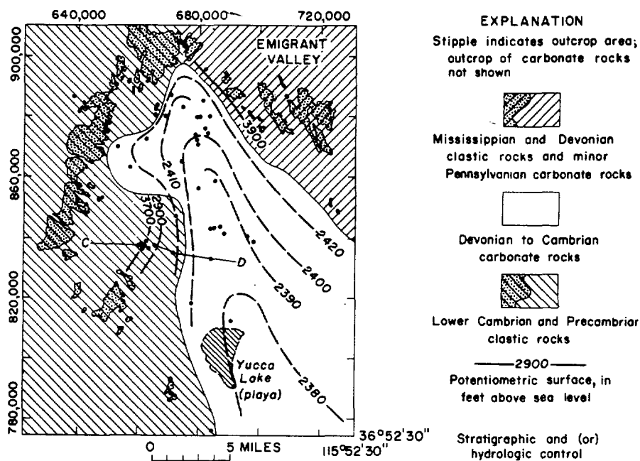
Figure 4. Approximate distribution of pre-Tertiary rocks at 2400-ft altitude and their potentiometric surface, Yucca Flat. Tertiary and Quaternary rocks, which extend below 2400 ft altitude in the central part of the valley, are not shown. The Cambrian through Devonian carbonate aquifers are saturated only below 2420 ft altitude, whereas the Precambrian and Lower Cambrian and Devonian and Mississippian clastic rocks are saturated to altitudes up to and above 3900 ft. The centrally located carbonate wedge thus serves as an hydraulic sink for ground water in the clastic strata. C-D, line of section of Figure 5. 40,000-ft grid based on Nevada State Co-ordinate System (Central Zone).
