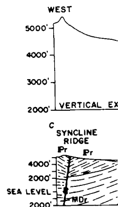
Figure 5. Geologic section shown on Figure 4. Pr, Pennsylvanian carbonate rocks (Eleana Formation);
