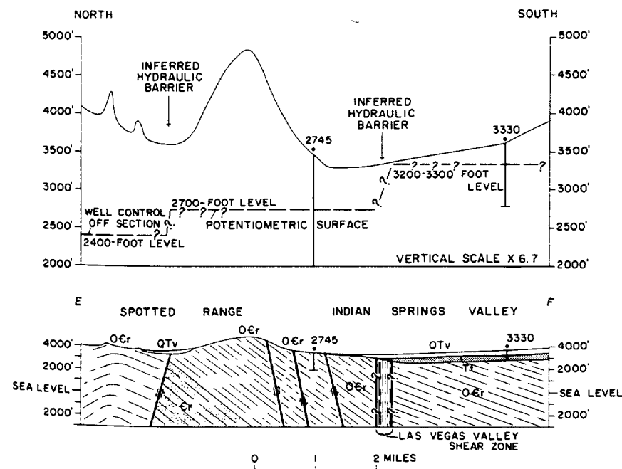
Figure 7. Geologic and hydrologic cross section, southern Indian Springs Valley. Line of section shown on Figure 6. QTv, Quaternary and Tertiary valley fill; Tt, Tertiary tuff; OCr, Ordovician and Cambrian carbonate rocks; Cr, Lower Cambrian clastic rocks.
