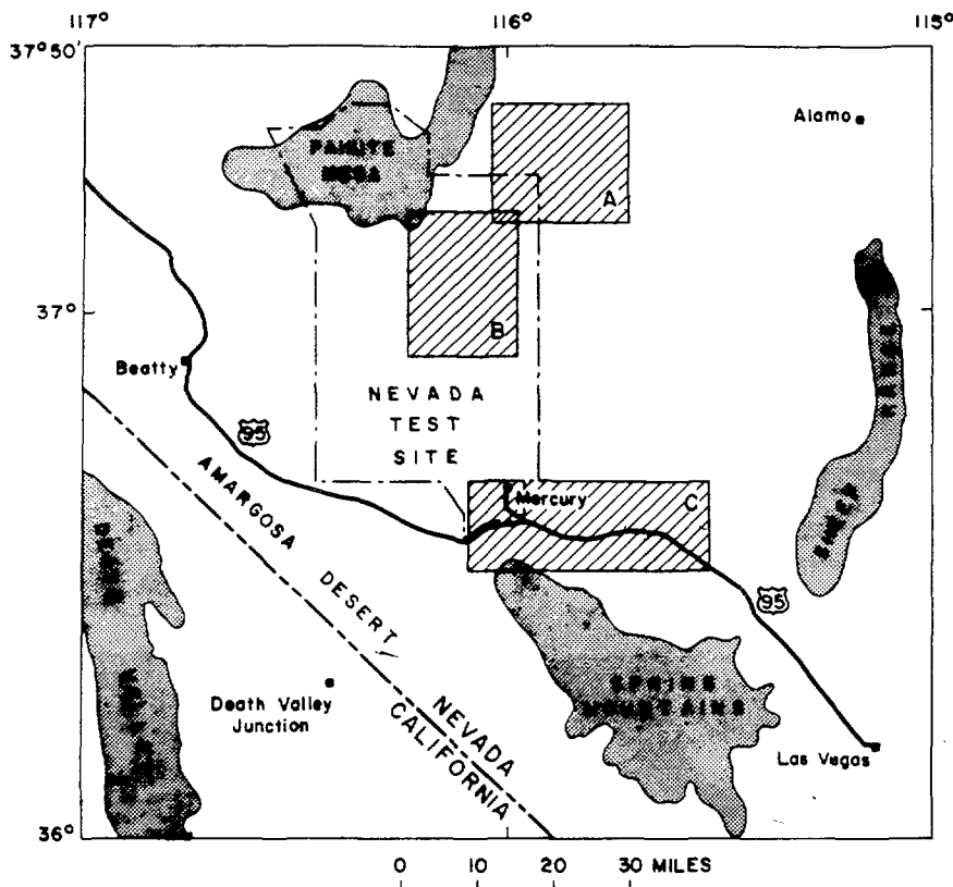
Figure 1. Index map of south-central Nevada, showing areas discussed in the text. (A) Emigrant Valley, area of Figure 2; (B) Yucca Flat, area of Figure 4; (C) southern Indian Springs Valley, area of Figure 6.
