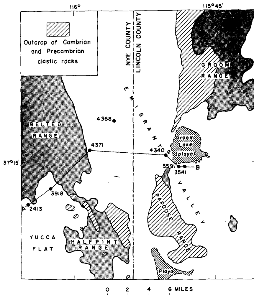
Figure 2. Areas of Precambrian and Lower Cambrian outcrops and subsurface control points, Emigrant Valley. A-B, line of section shown on Figure 3; numbers adjacent to wells represent altitude, in feet above sea level, of water level in well.
