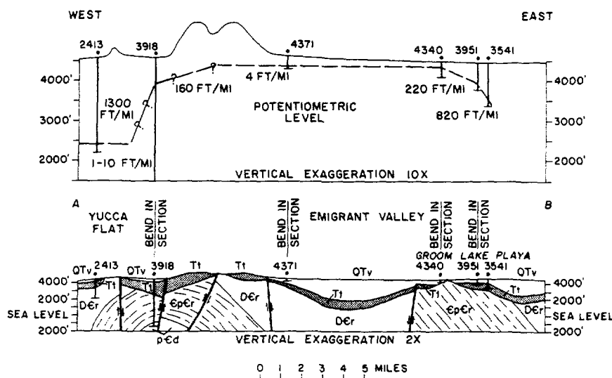
Figure 3. Geologic and hydrologic cross section, Yucca Flat to Groom Lake playa. Line of section shown on Figure 2; well numbers represent altitude, in feet above sea level, of water level in well. QTv, Quaternary and Tertiary valley fill; Tt, Tertiary tuff; D-Cr, Devonian to Cambrian carbonate rocks; Ep-Cr, Lower Cambrian to Precambrian clastic rocks; p-Cd, Precambrian dolomite.)
