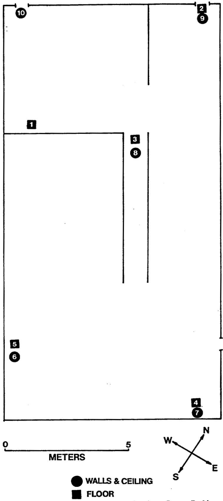
FIGURE 15: Floor Plan of the Locker Room Indicating Locations of Measurements and Smears
