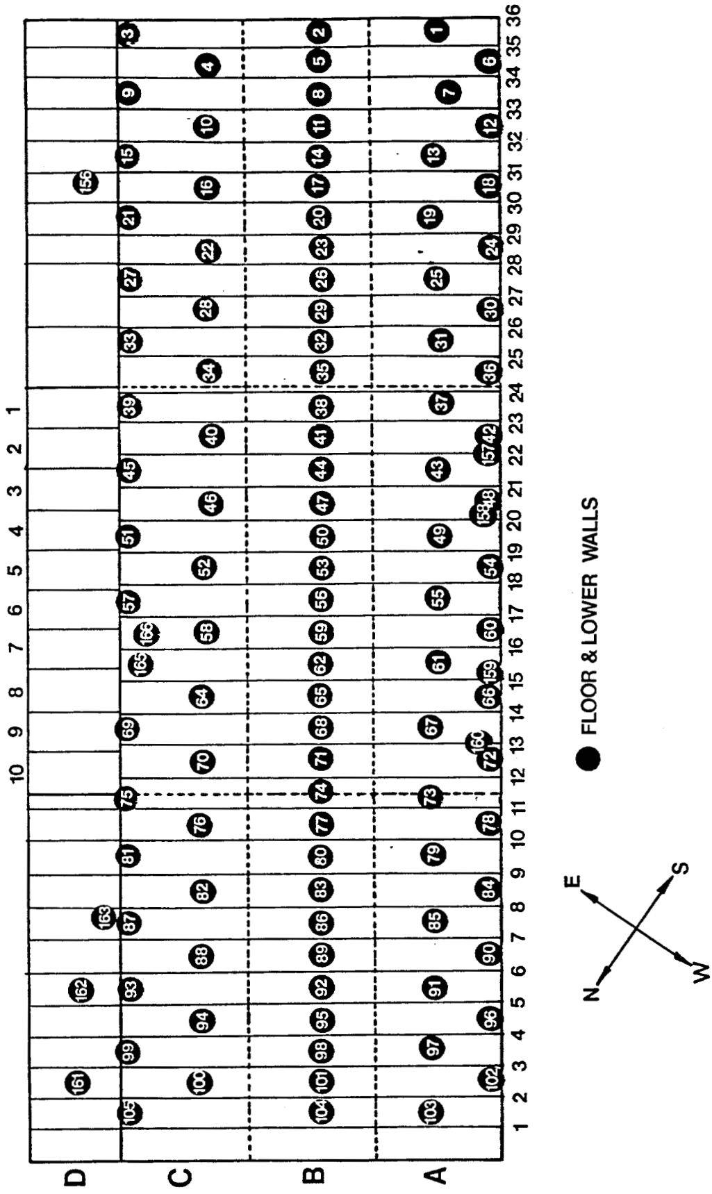
FIGURE 8A: Floor Plan of the Alloy Building Indicating Locations of Measurements and Smears (Floor and Lower Walls)
