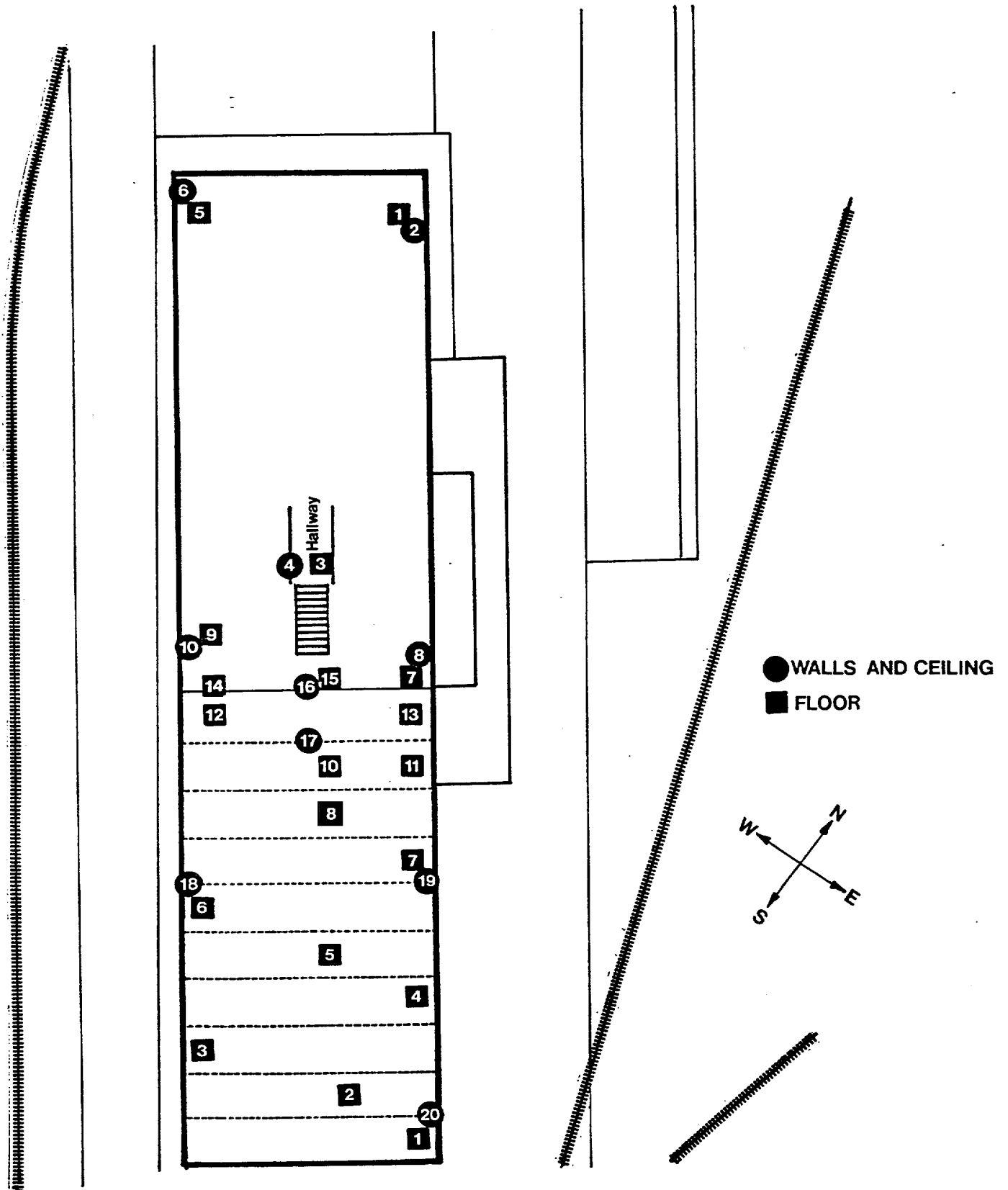
FIGURE 11: Floor Plan of Building No. 2 Indicating Locations of Measurements and Smears
