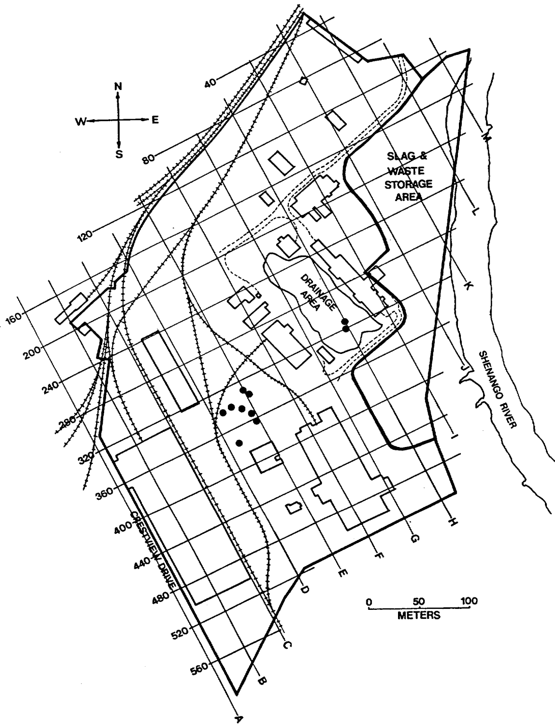
FIGURE 6: Locations of Areas of Elevated Direct Radiation After Decontamination.
