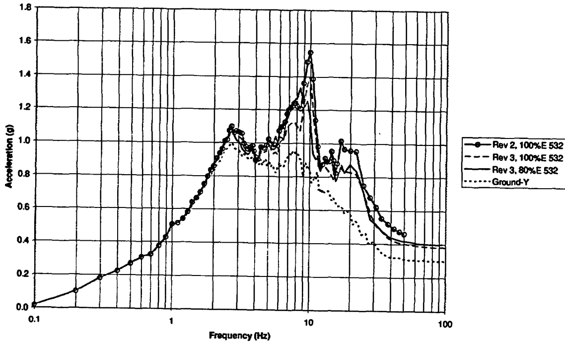
Figure 3.7.2.9-1-1: Node 532 – FRS comparison - Y Direction
