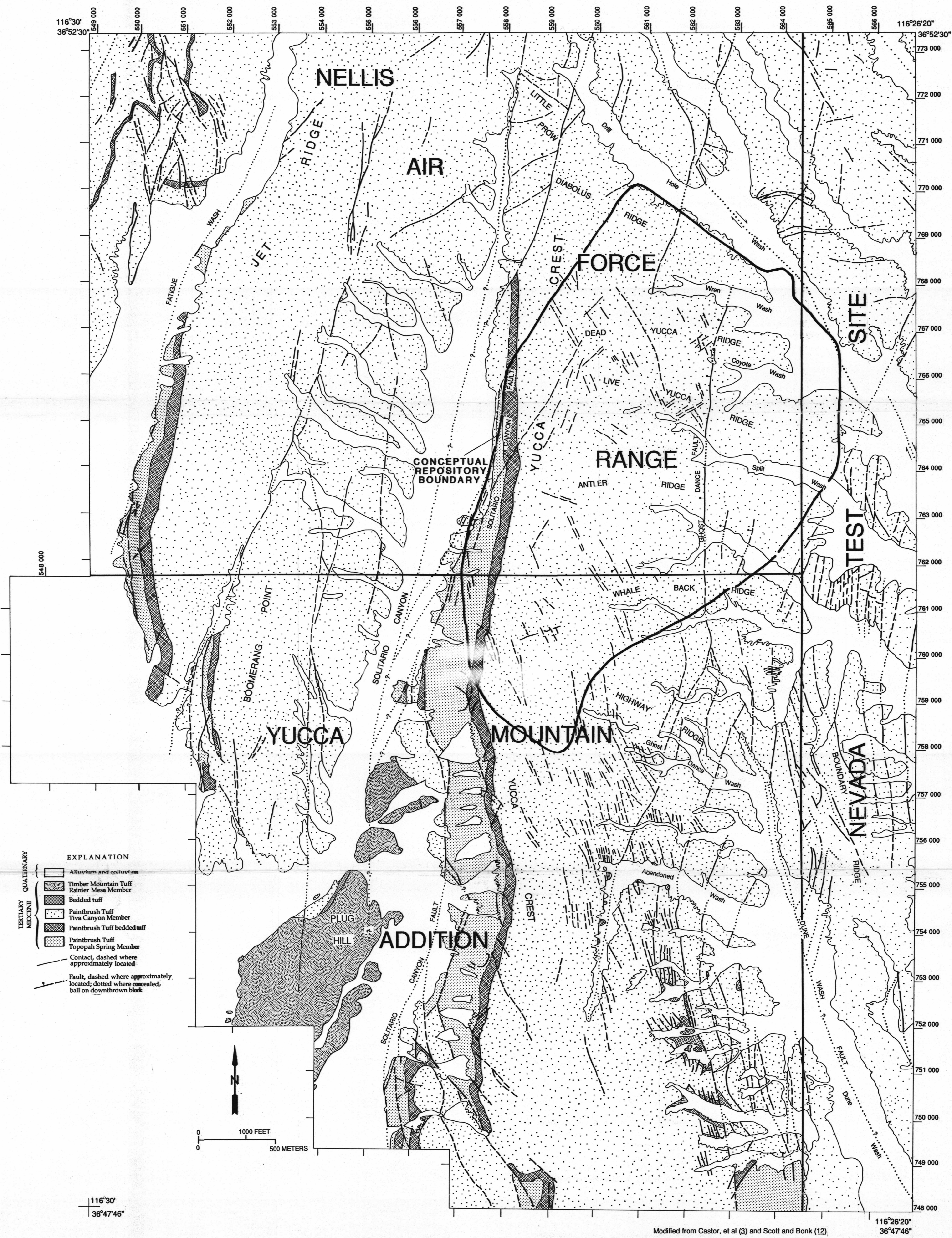
PLATE 1.- Simplified geologic map of Yucca Mountain in the vicinity of the perimeter drift
