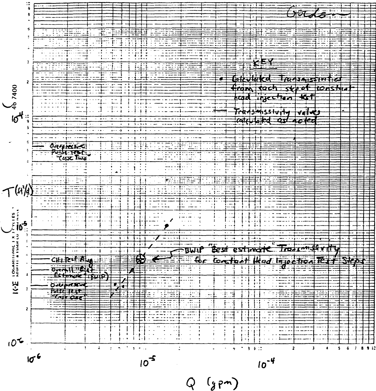
Figure 1. Flowrate vs. transmissivity for each step. T1-109 Cohasset Interior 4 Step Injection Test
