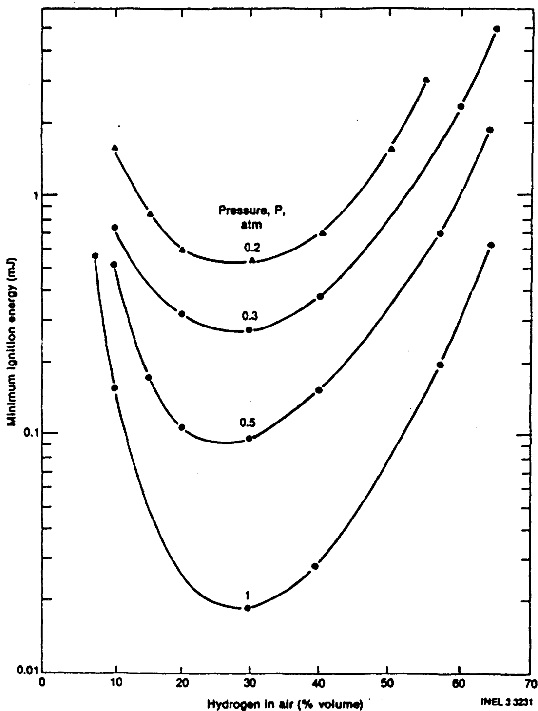
Figure 3.2 Spark Ignition Energies for Hydrogen/Air Mixtures (From Randolph et al., 1985)
