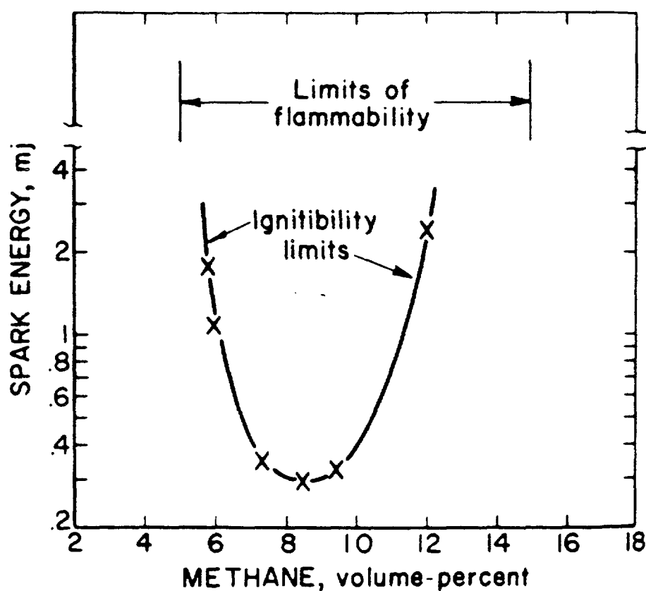
Figure 3.1 Spark Ignition Energies, Ignitibility Curve, and Limits of Flammability for Methane-Air Mixtures at Atmospheric Pressure and 26°C. (From Zabetakis, 1965)
