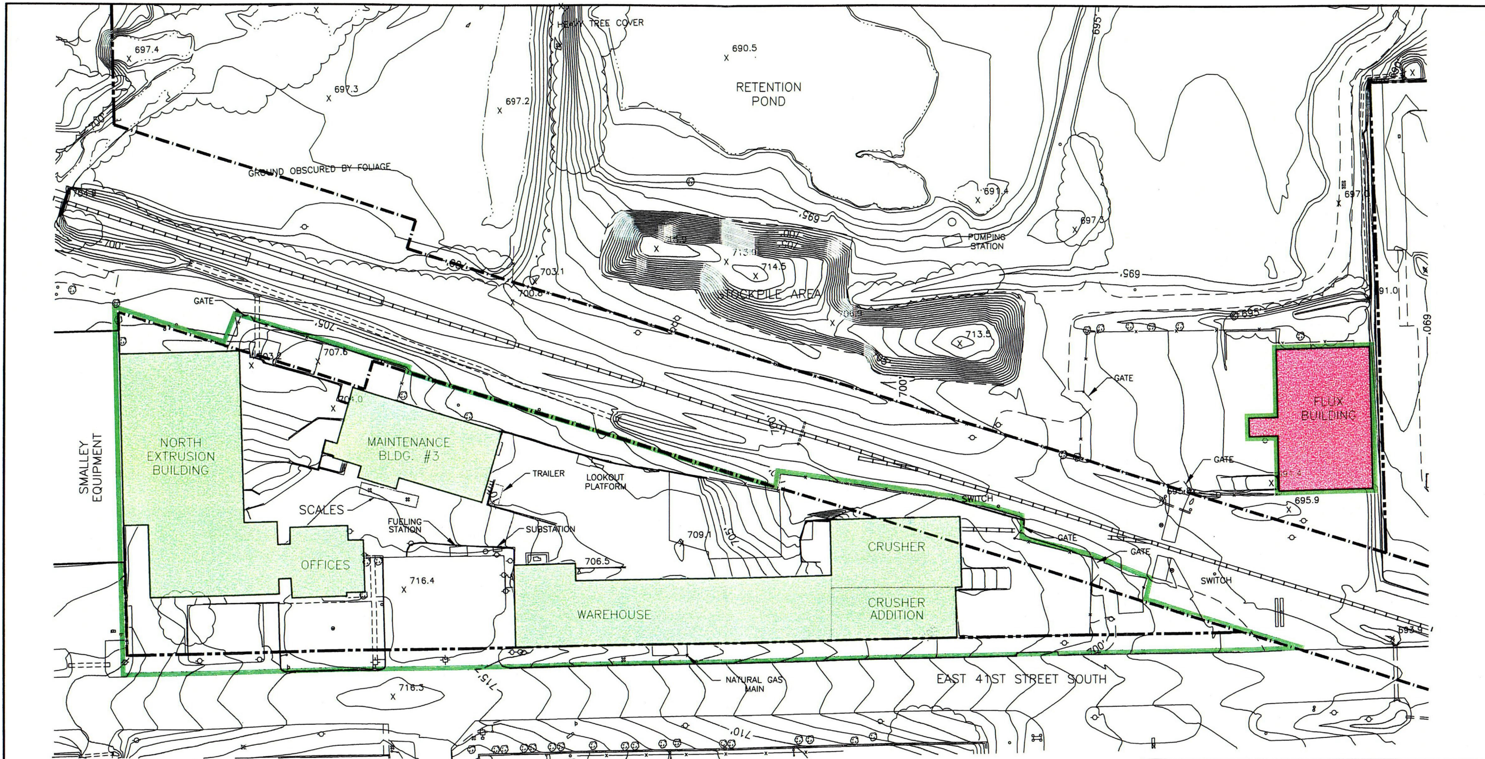
FIGURE 9 CONCEPTUAL MODEL OF STRUCTURES FORMER KAISER ALUMINUM SPECIALTY PRODUCTS FACILITY TULSA, OKLAHOMA
