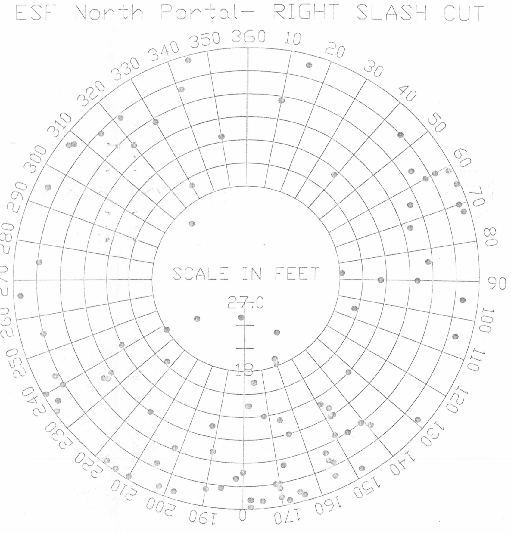
Continuity Plot
