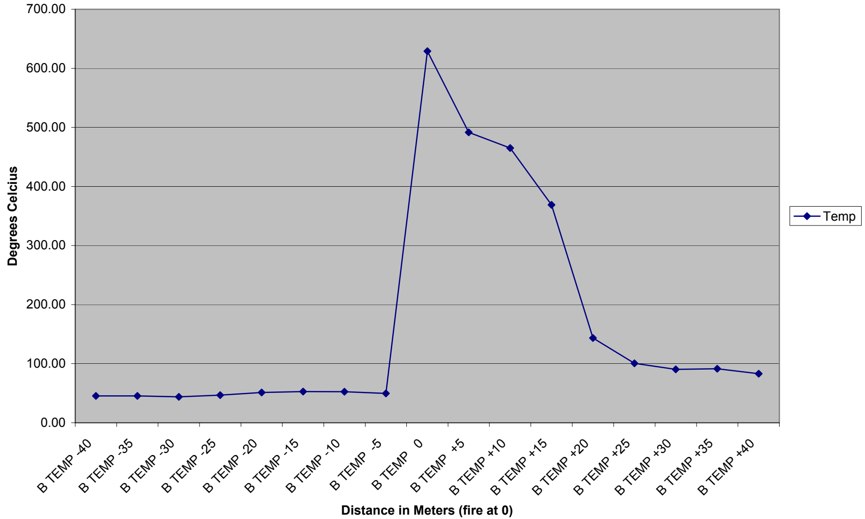
Temperature at Bottom of Railcars
