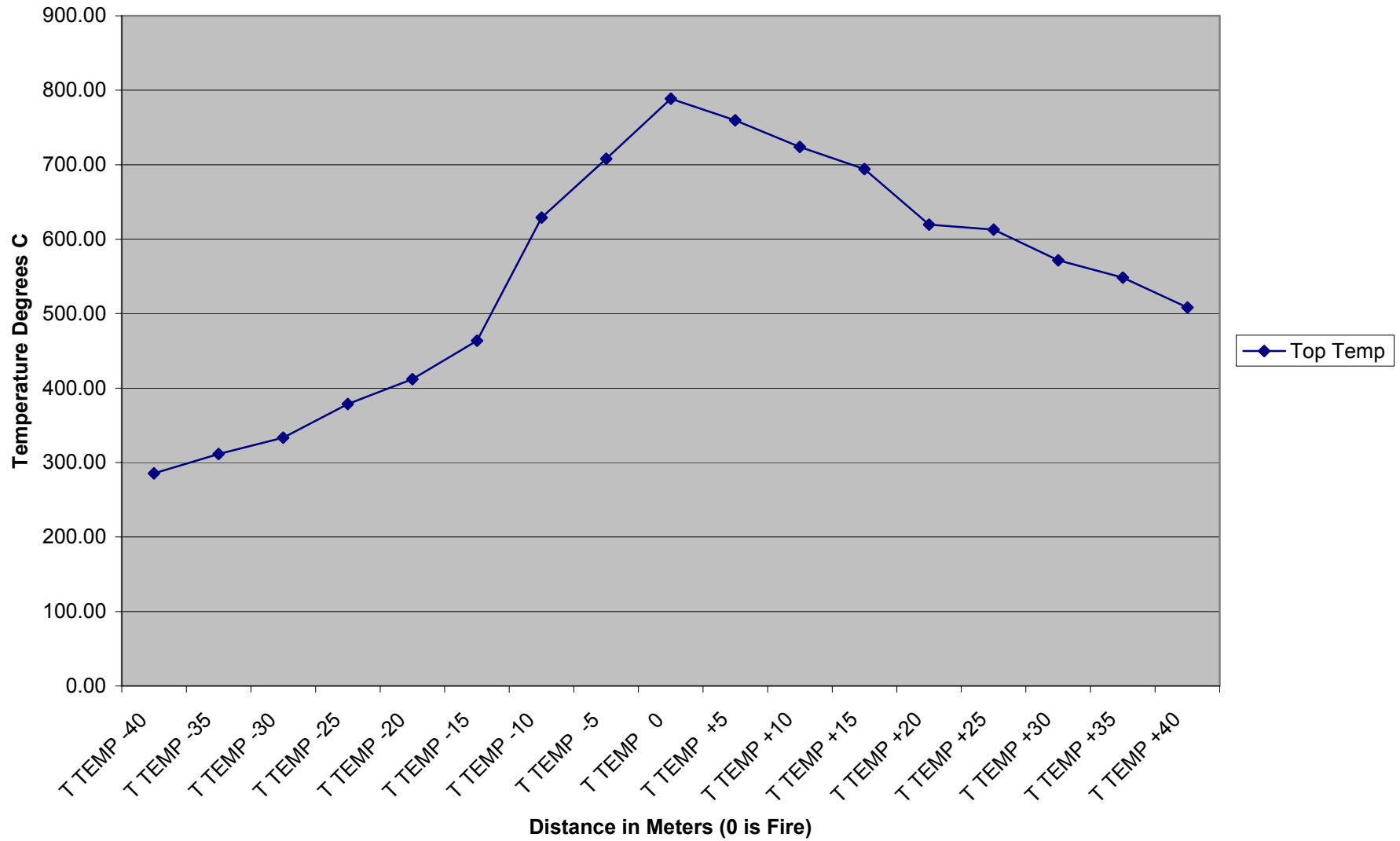
Temps at Top of Railcars
