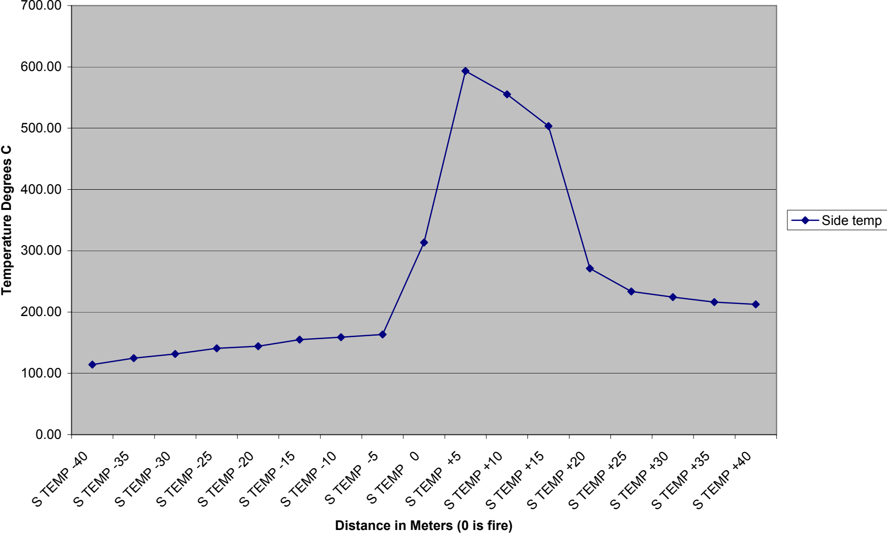
Temperatures at railcar sides
