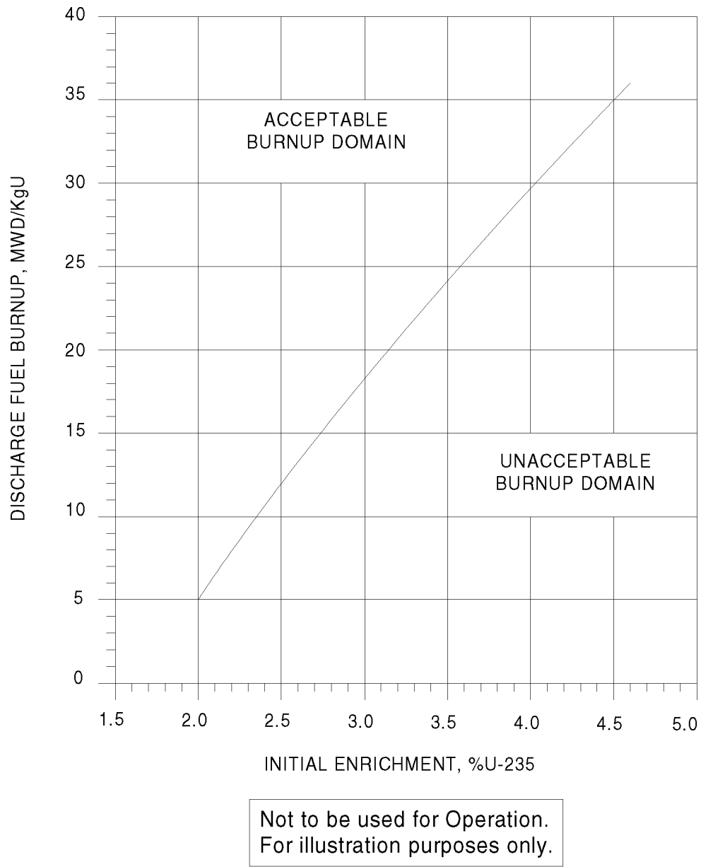
Figure 3.7.17-1 (page 1 of 1) Fuel Assembly Burnup Limits in Region 2
