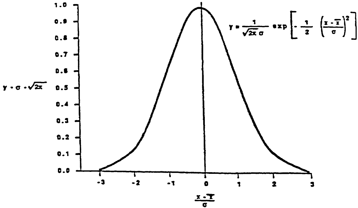
Figure B-2 A Gaussian Curve
