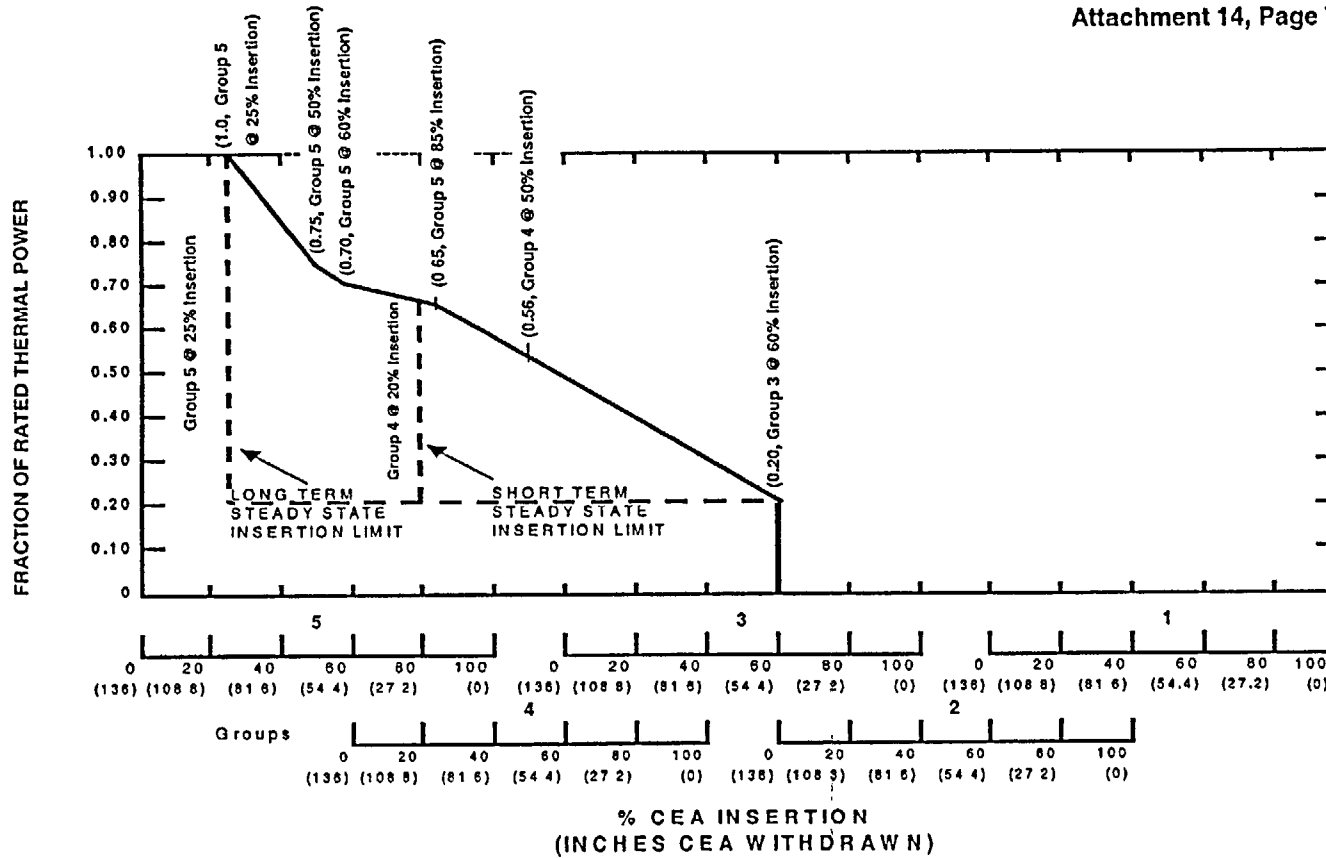
FIGURE 3.1-2 CEA Group Insertion Limits vs. THERMAL POWER
