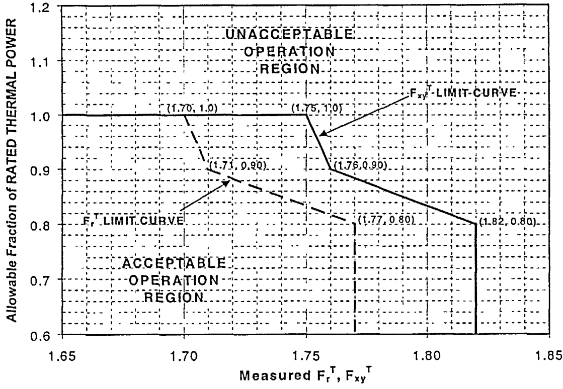
FIGURE 3.2-3 Allowable Combinations of THERMAL POWER and F_r^T, F_{xy}^T
