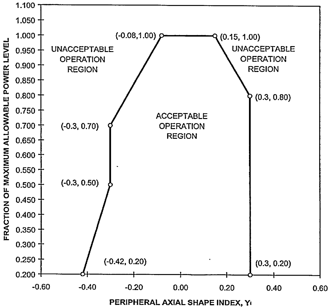
Figure 3.2.5 DNB Axial Flux Offset Control Limits (See NEOP-23 for Administrative Limits)
