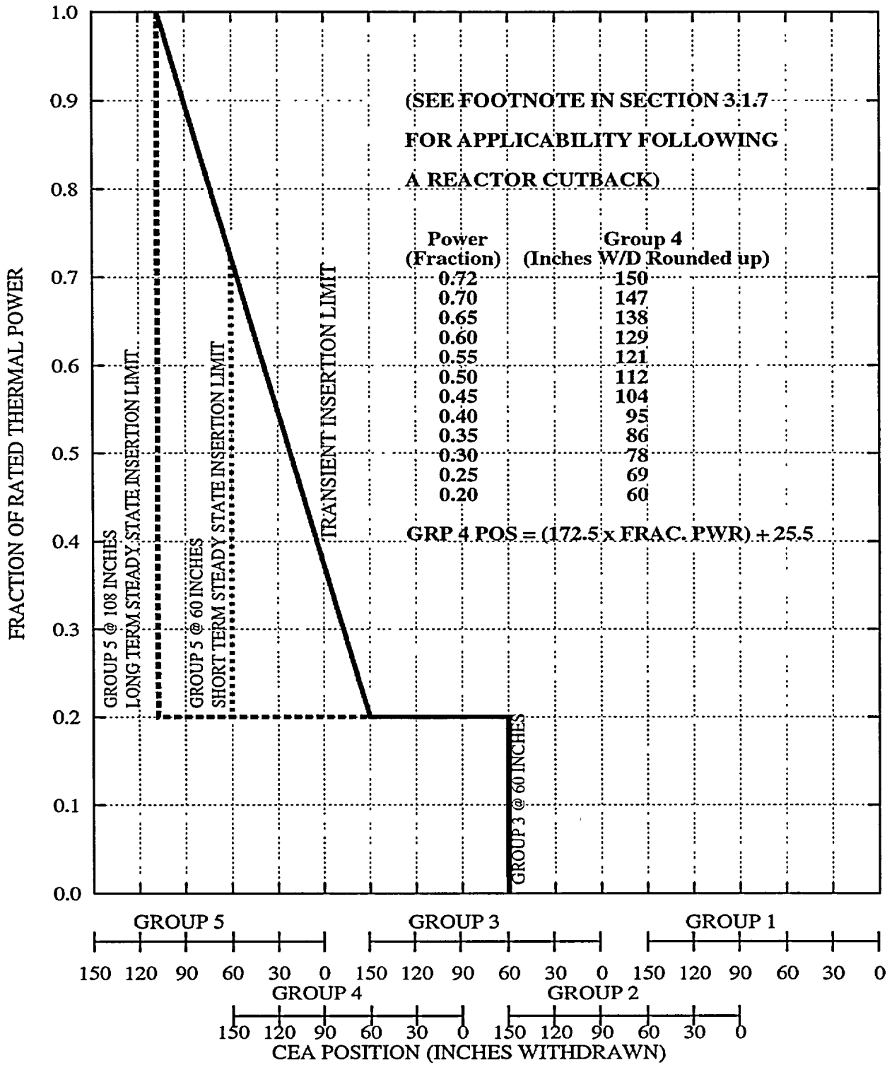
FIGURE 3.1.7-1 CEA INSERTION LIMITS VERSUS THERMAL POWER (COLSS IN SERVICE)
