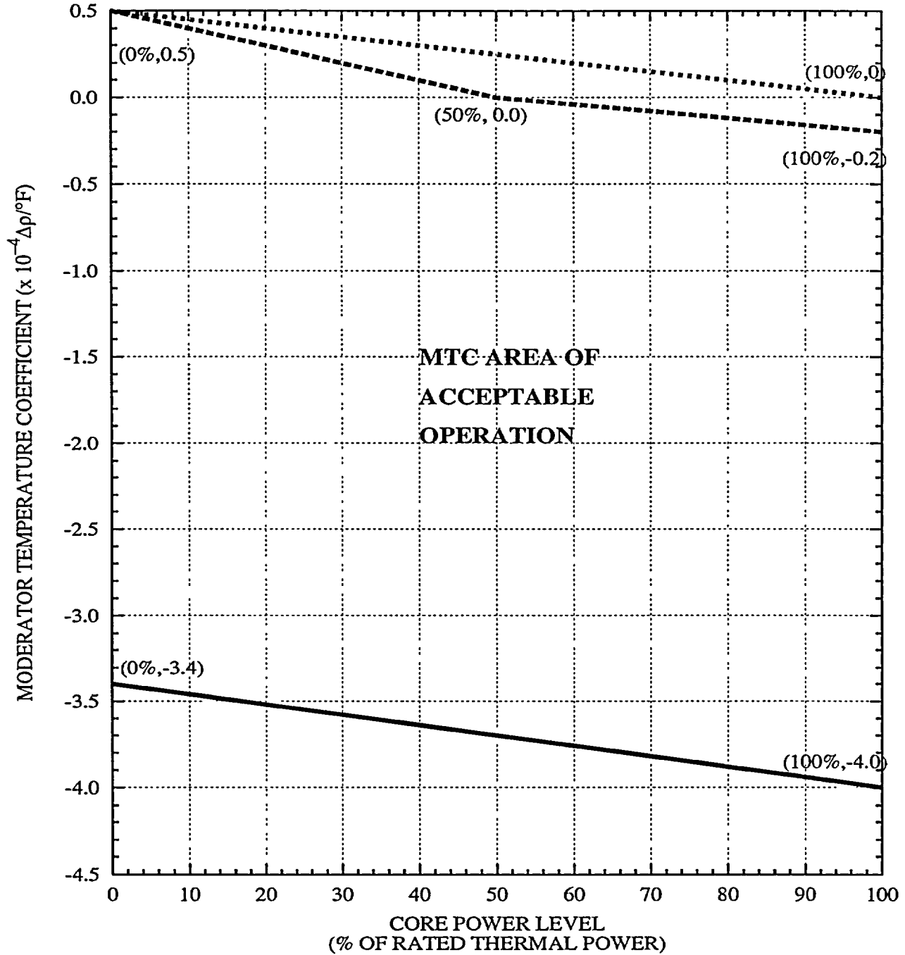
FIGURE 3.1.4-1 MTC ACCEPTABLE OPERATION, MODES 1 AND 2
