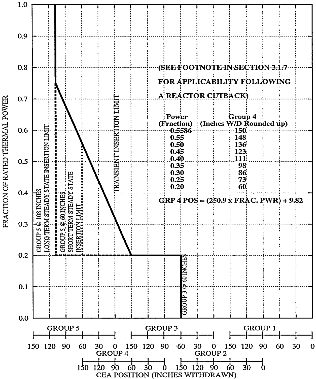
FIGURE 3.1.7-2 CEA INSERTION LIMITS VERSUS THERMAL POWER (COLSS OUT OF SERVICE)
