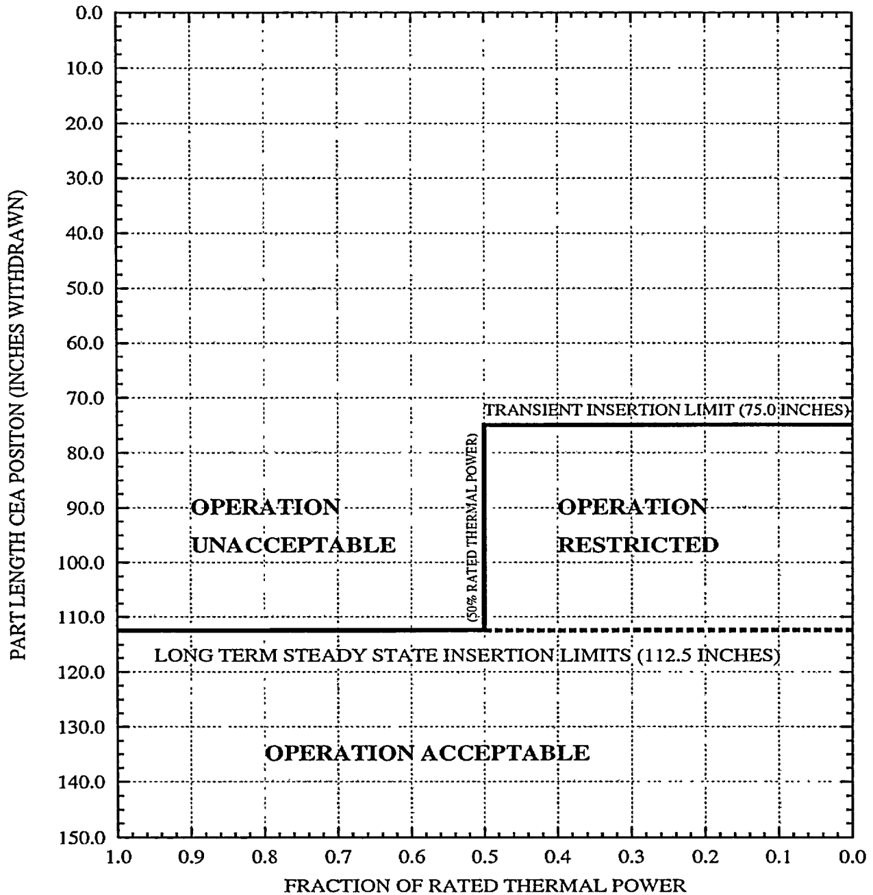
FIGURE 3.1.8-1 PART LENGTH CEA INSERTION LIMITS VERSUS THERMAL POWER
