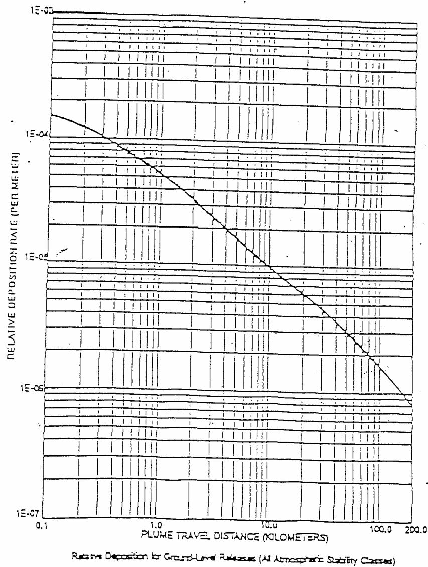
Figure 7.6 RELATIVE DEPOSITION FOR GROUND LEVEL RELEASES (All Stability Classes)
