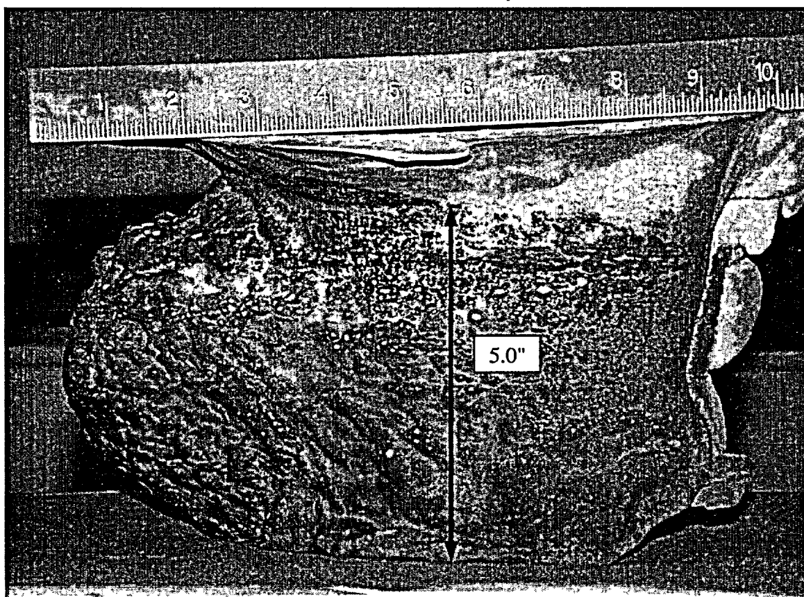
Davis-Besse Cavity Mold at 270° 0.55X
