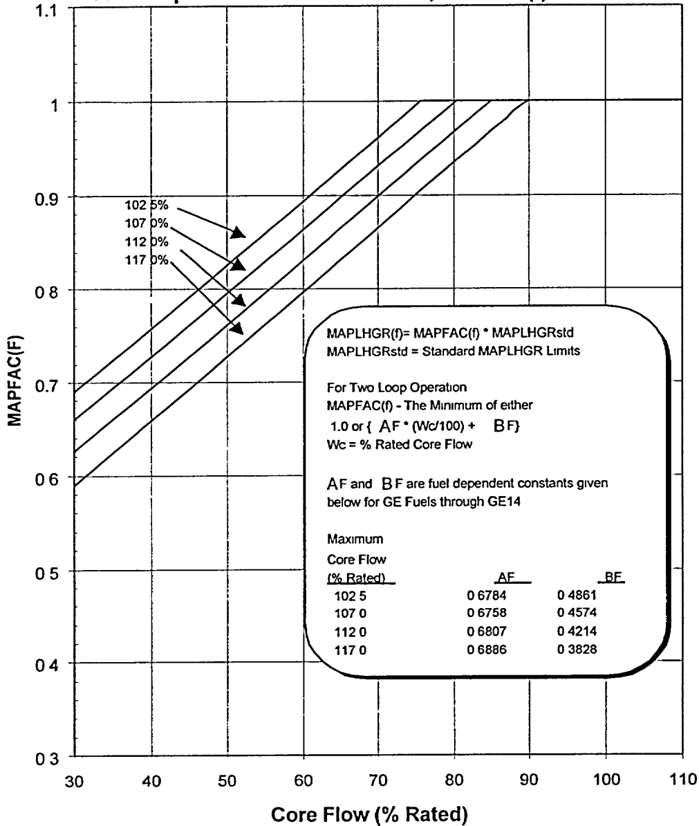
Flow-Dependent MAPLHGR Factor, MAPFAC(f)
