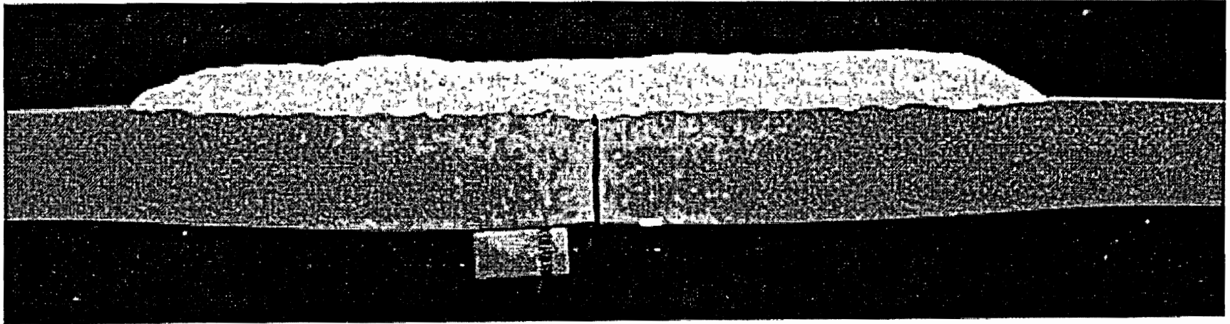
Section through a weld-overlay repair of a through-wall crack in a 6-inch diameter TP304 stainless steel pipe after loading. (Degraded Piping Program, DRB No. 1.2.3.6)
