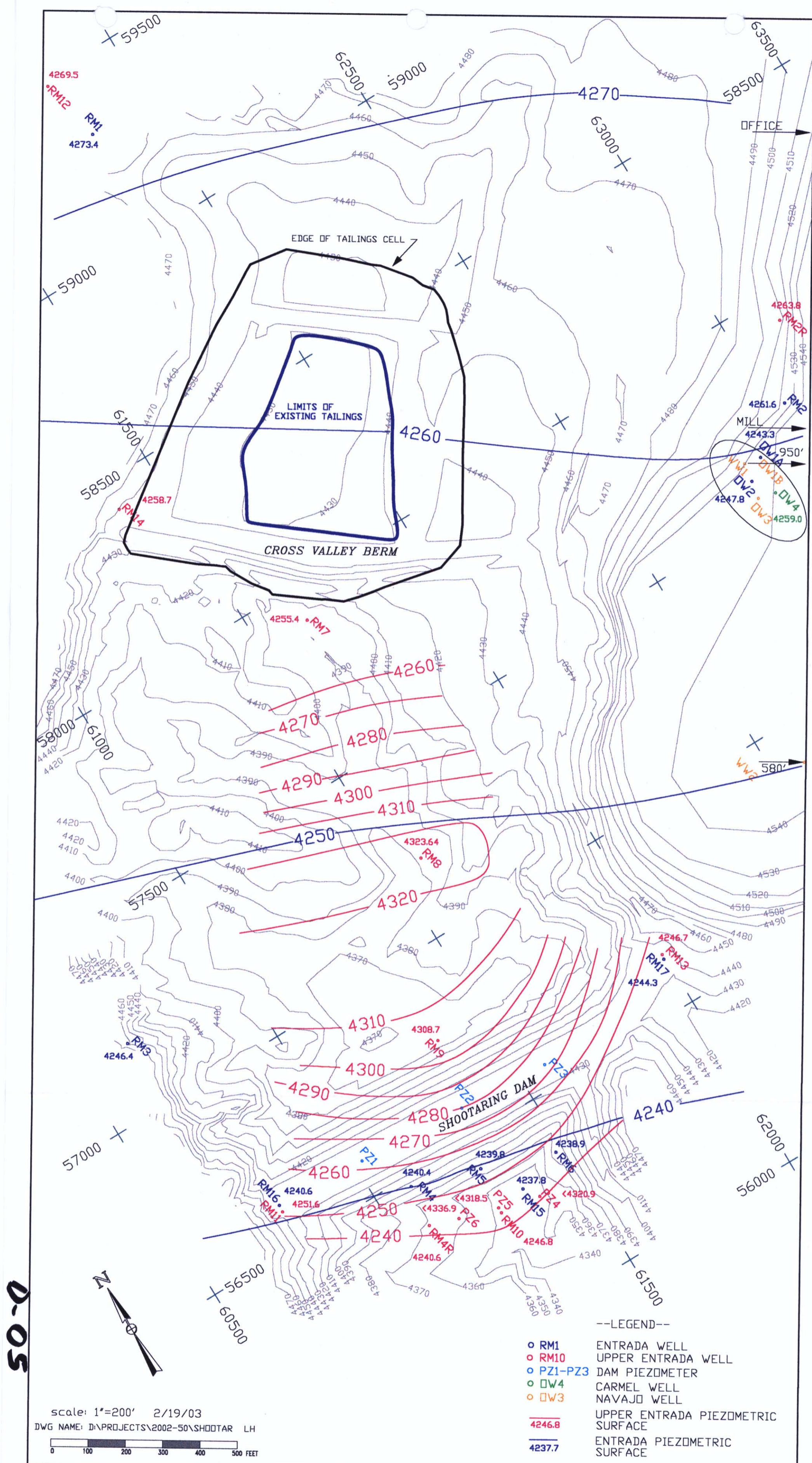
FIGURE 4-1. WATER-LEVEL ELEVATION IN THE UPPER ENTRADA AND ENTRADA AQUIFER, 2002, FT-MSL
