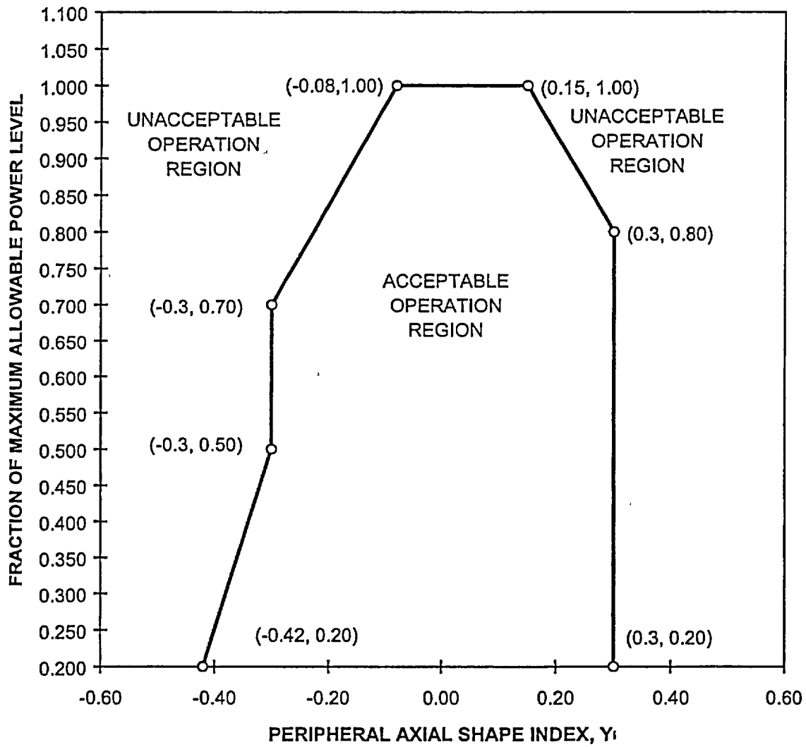
Figure 3.2.5 DNB Axial Flux Offset Control Limits (See NEOP-23 for Administrative Limits)
