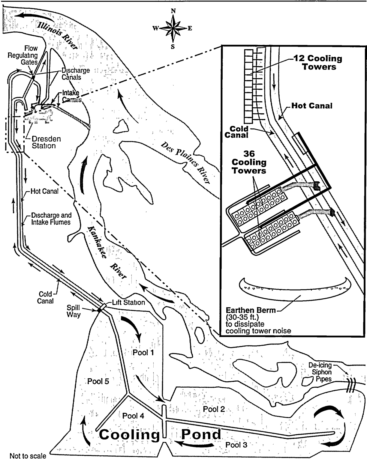
FIGURE 3-2. Cooling Water System Schematic.
