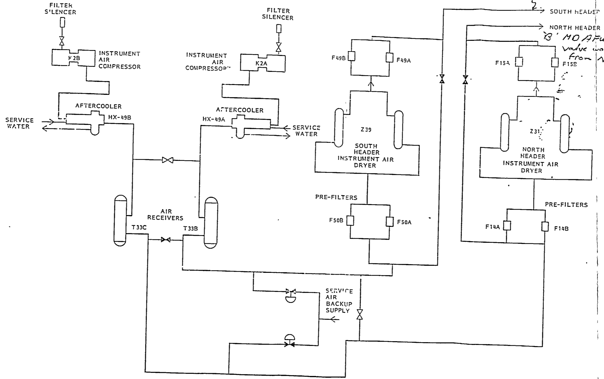
INSTRUMENT AIR SYSTEM SIMPLIFIED DIAGRAM Figure 11.11.1
