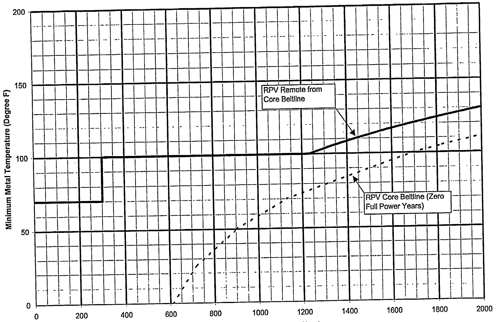
Figure 3.6.2 Minimum Temperature vs. Pressure For Pressure Tests
