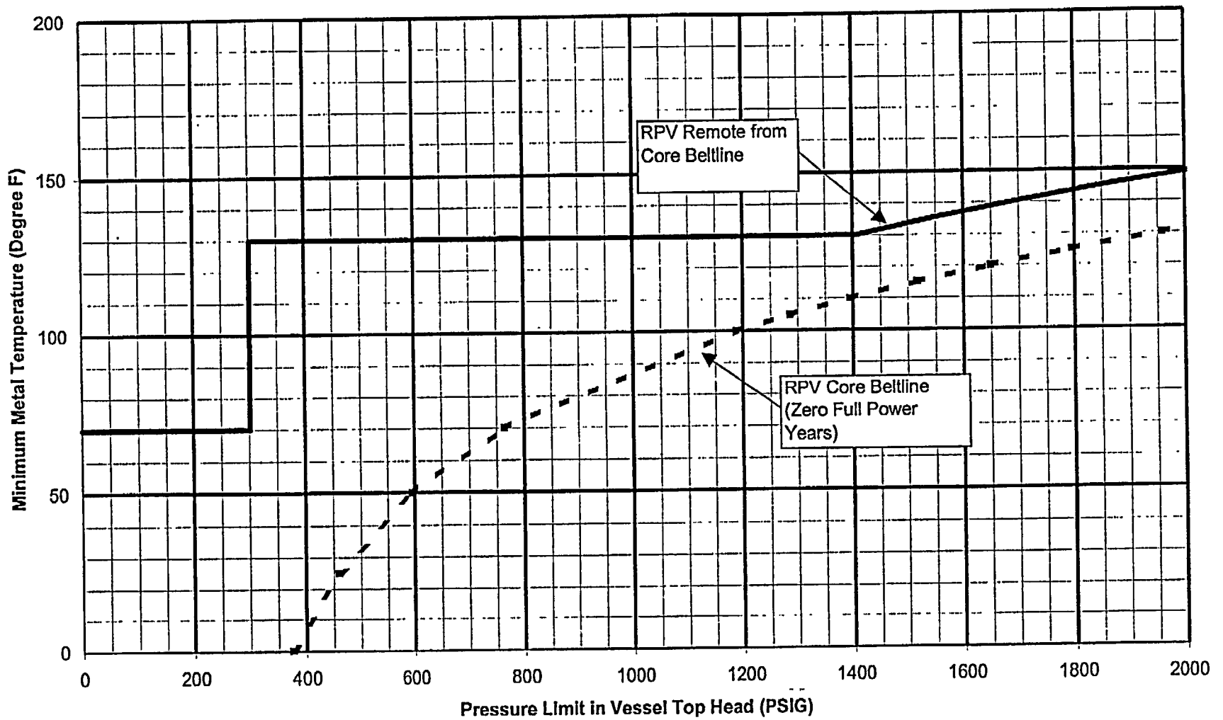
Figure 3.6.3 Minimum Temperature vs. Pressure Mechanical Heatup or Cooldown without the Core Critical
