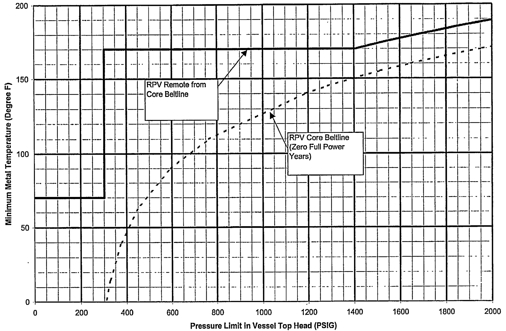
Figure 3.6.4 Minimum Temperature Vs. Pressure for Core Critical Operation
