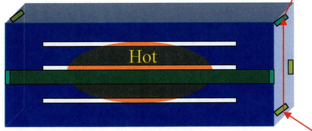
Air Flow within HI-STORM 100 cask
