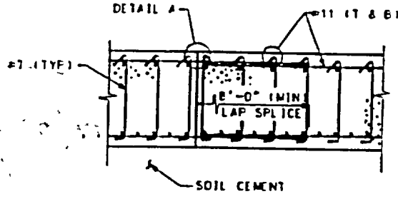
TYP CONSTRUCTION JT CASK STORAGE PAD
