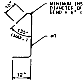
DETAIL C TYPICAL TIE DETAIL
