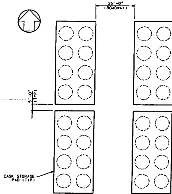
PARTIAL PLAN TYPICAL CASK STORAGE PAD SPACING
