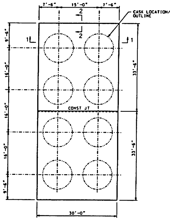
PLAN CASK STORAGE PAD (500 REQD)
