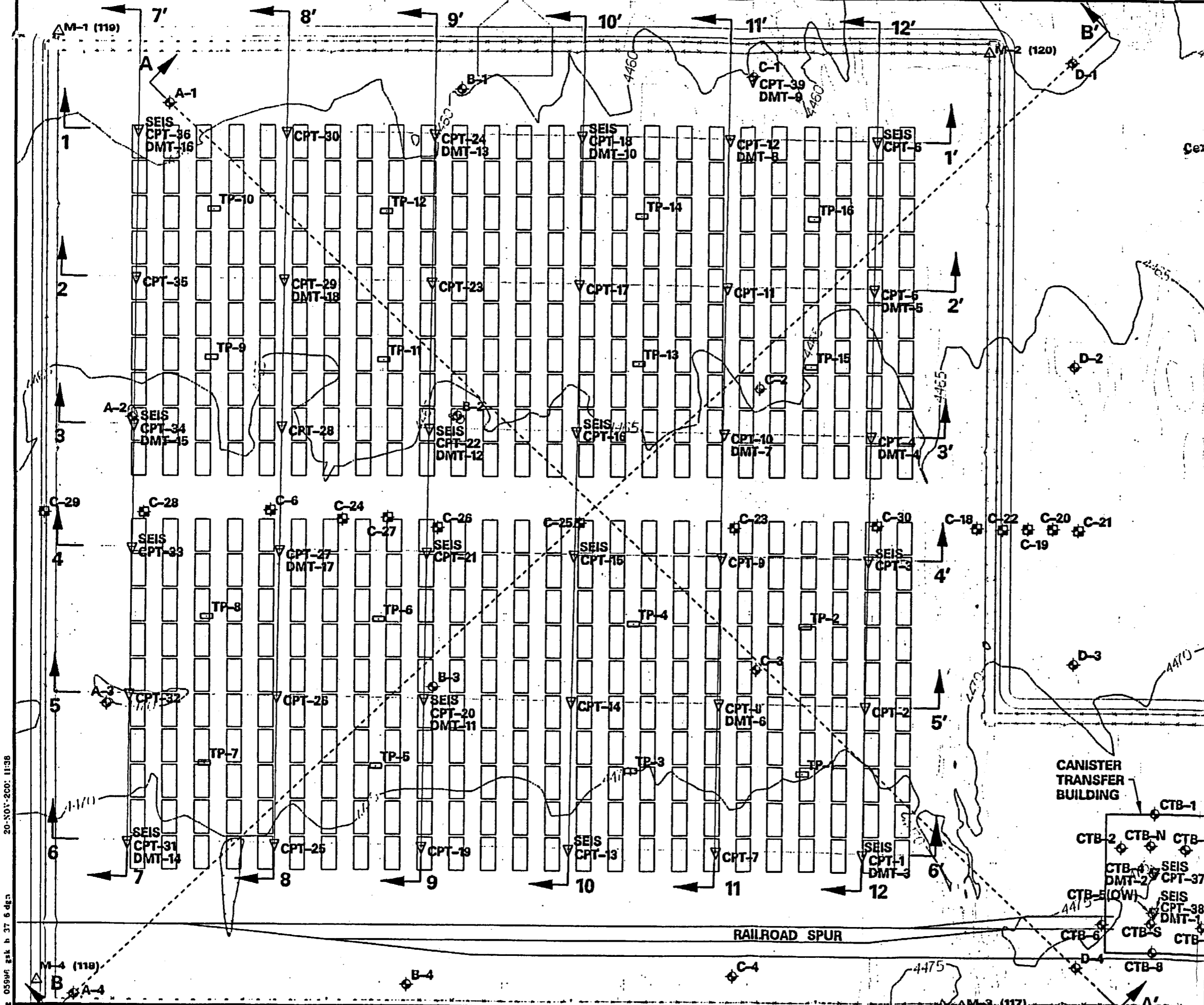
Figure 2.6-19 LOCATIONS OF GEOTECHNICAL INVESTIGATIONS IN PAD EMPLACEMENT AREA PRIVATE FUEL STORAGE FACILITY SAFETY ANALYSIS REPORT
