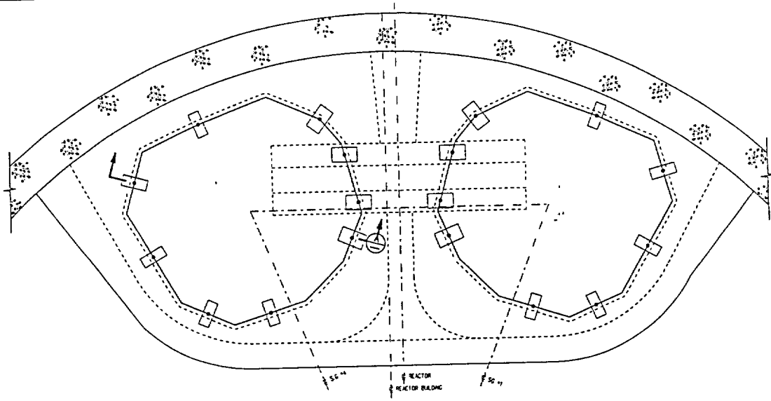
PARTIAL PLANS TOP SLAB STEAM GENERATOR ENCLOSURES 1/2" = 1'-0"
