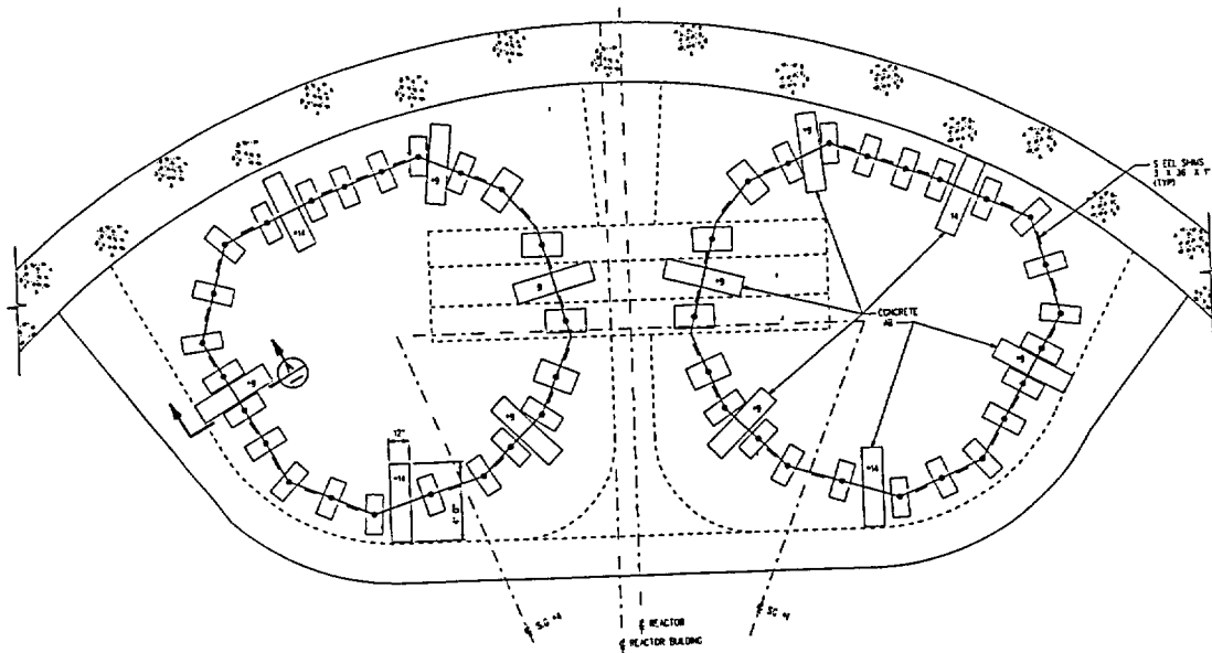
PARTIAL PLANS TOP SLAB STEAM GENERATOR ENCLOSURES A. 178 APPROX 1/4" = 1'-0"
