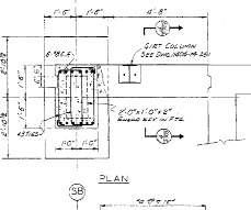
PLAN - SERVICE BUILDING FOOTINGS SCALE 1/4" = 1'-0"
