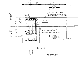
PLAN - SERVICE BUILDING FOOTINGS SCALE 1/4" = 1'-0"
