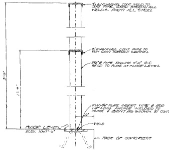
SECTION THRU RAILING SCALE: 1/4" = 1'-0"
