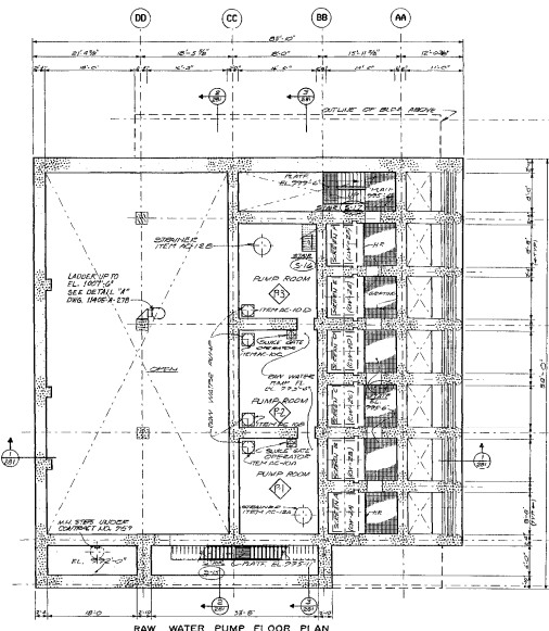
RAW WATER PUMP FLOOR PLAN PLAN AT ELEVATION 993'-6" SCALE: 1/8" = 1'-0"
