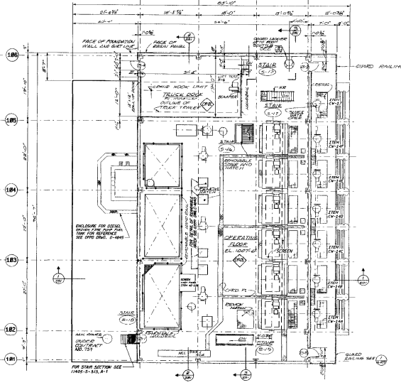
OPERATING FLOOR PLAN PLAN AT ELEVATION 1007'-6" SCALE: 1/8" = 1'-0"
