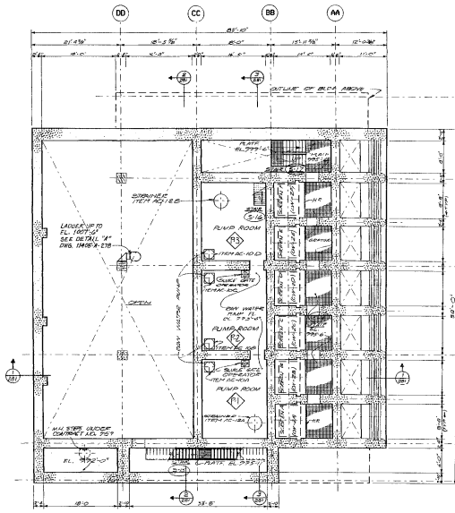
RAW WATER PUMP FLOOR PLAN PLAN AT ELEVATION 993'-6" SCALE: 1/8" = 1'-0"
