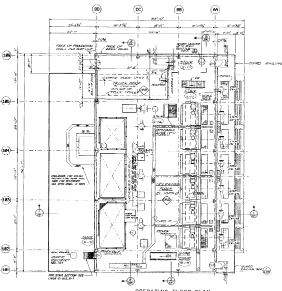
OPERATING FLOOR PLAN PLAN AT ELEVATION 1007'-6" SCALE: 1/8" = 1'-0"
