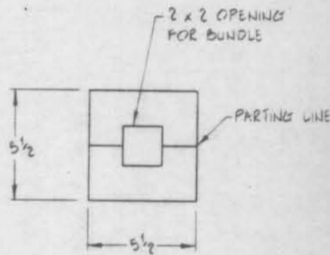
DETAIL II MATERIAL - ETHAFOAM CUSHION 2 LB DENSITY 'DOW CHEMICAL' OR AN APPROVED EQUAL
