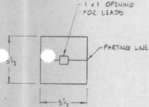
DETAIL III MATERIAL - ETHAFOAM CUSHION 2 LB DENSITY 'DOW CHEMICAL' OR AN APPROVED EQUAL
