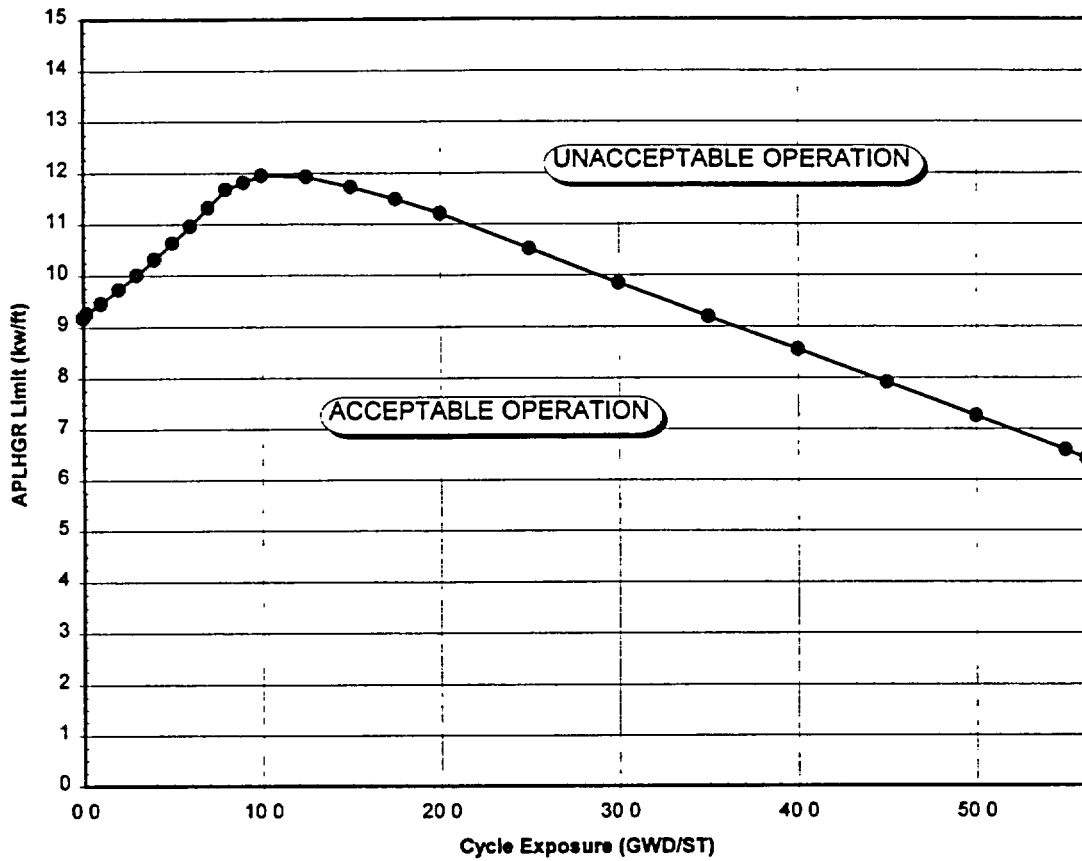
Figure 7 APLHGR Limits for Bundle Type GE11-P9HUB367-14GZ (GE11)
