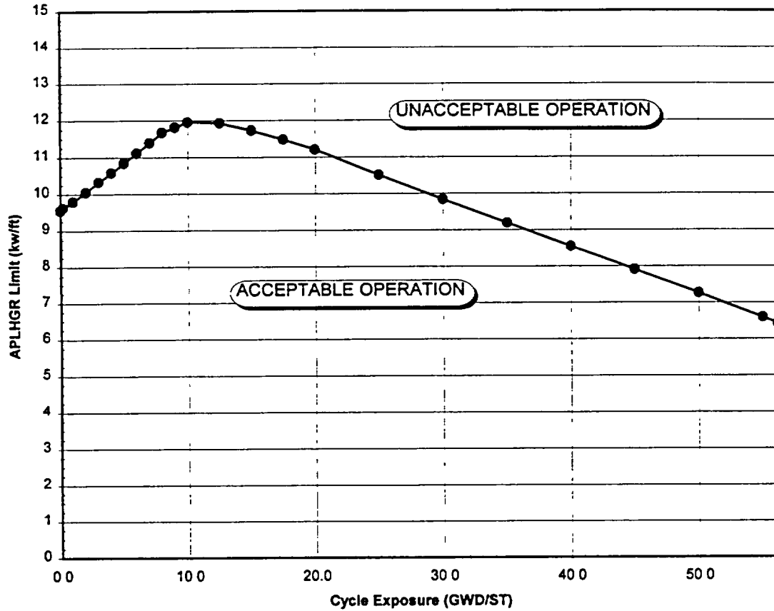
Figure 6 APLHGR Limits for Bundle Type GE11-P9HUB366-12G4.0 (GE11)
