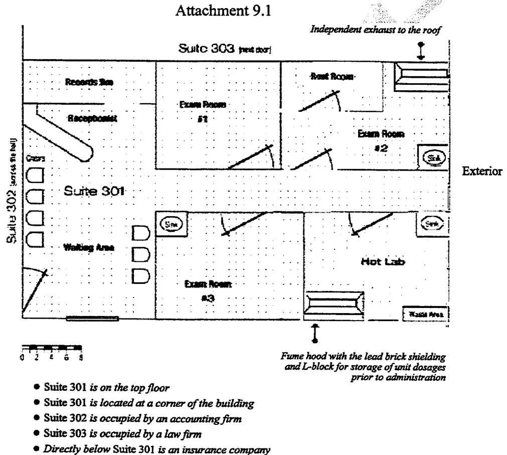
Figure 8.1: Facility Diagram for Nuclear Medicine Suite
