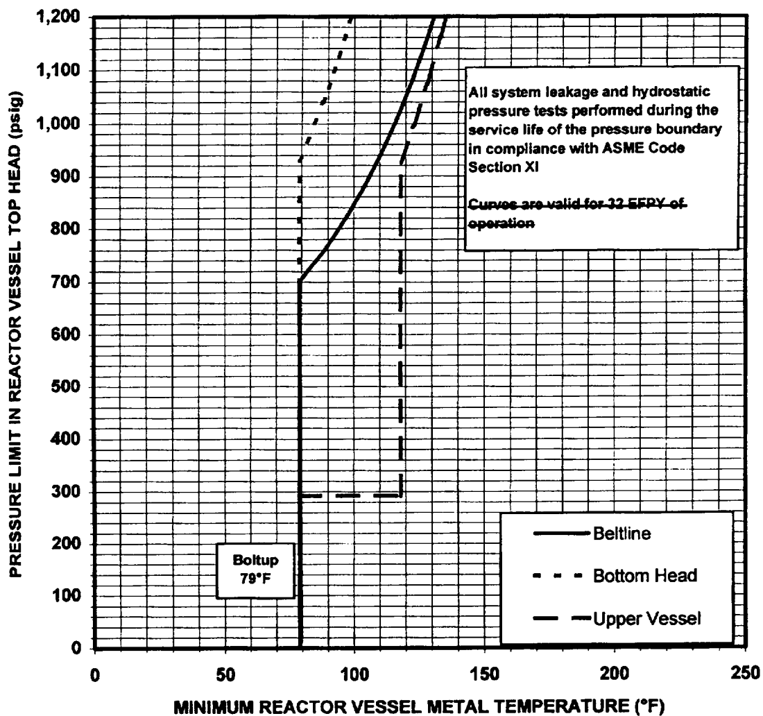
Figure 3.4.6.1-1 Hydrostatic Pressure and Leak Tests Pressure/Temperature Limits - Curve A
