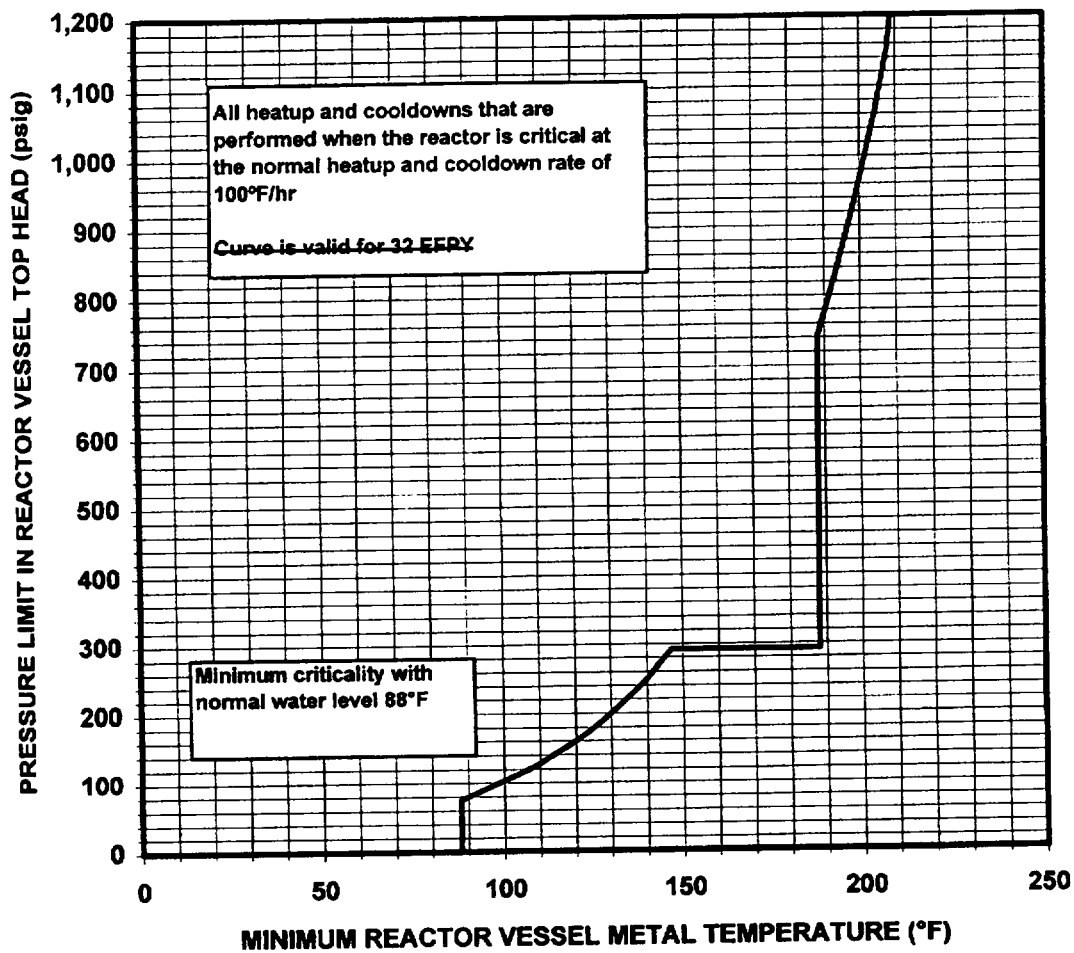
Figure 3.4.6.1-3 Core Critical Heatup and Cooldown Pressure/Temperature Limits - Curve C
