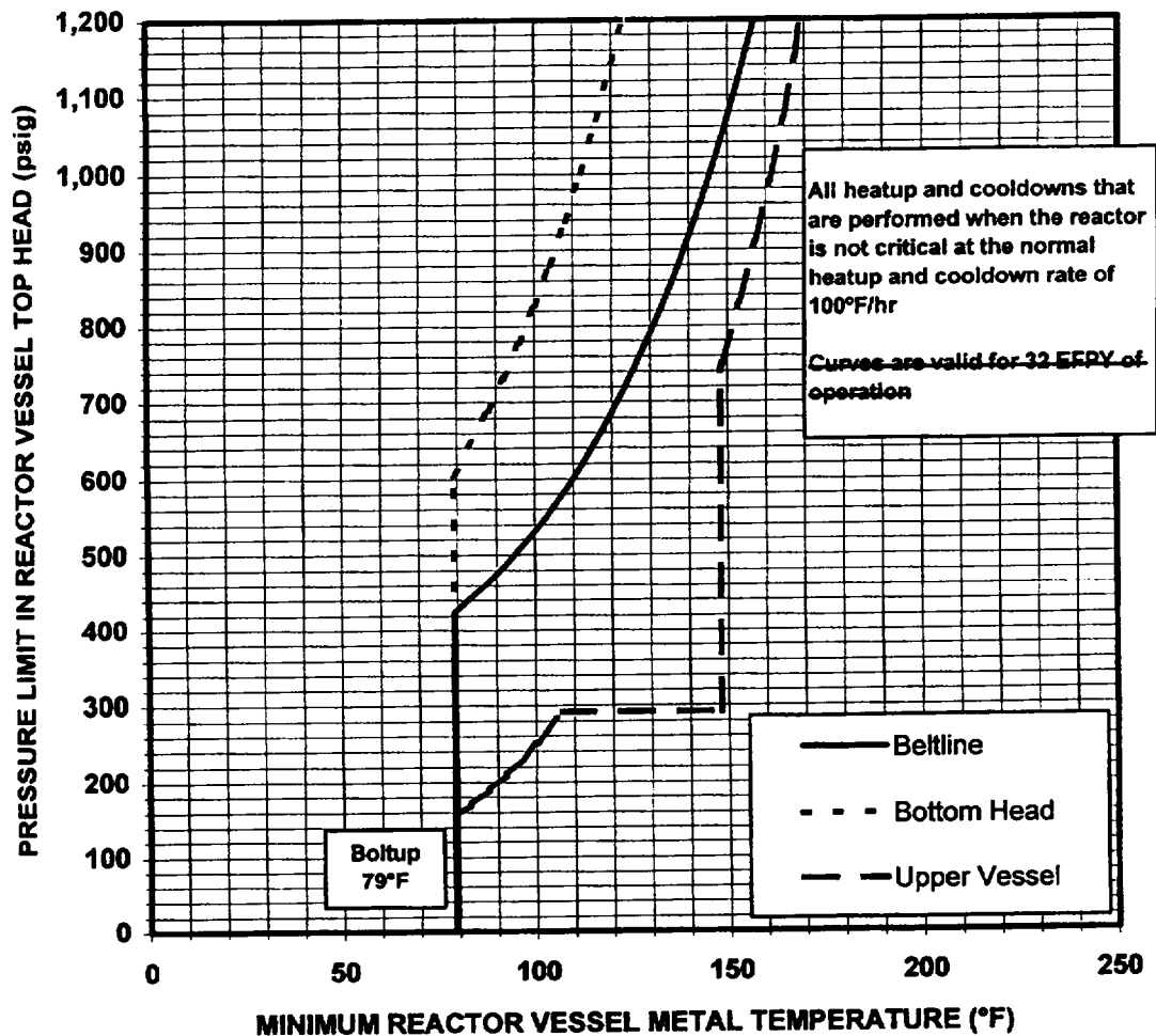
Figure 3.4.6.1-2 Non-Nuclear Heatup and Cooldown Pressure/Temperature Limits - Curve B
