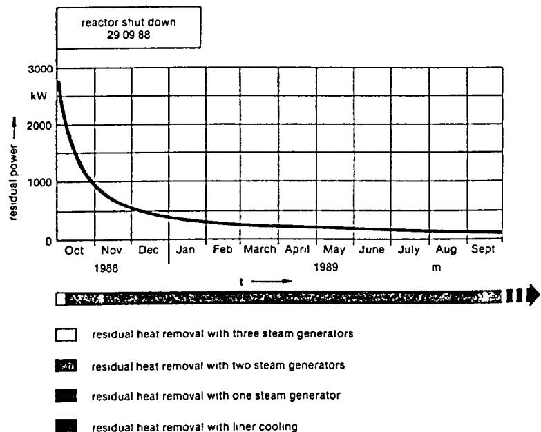
Fig 7 Residual heat removal during the outage phase
