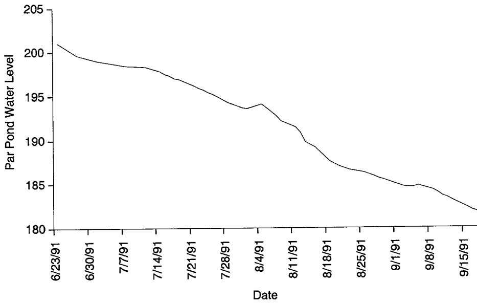
Figure 6-39. Par Pond Water-Level Change during Drawdown
