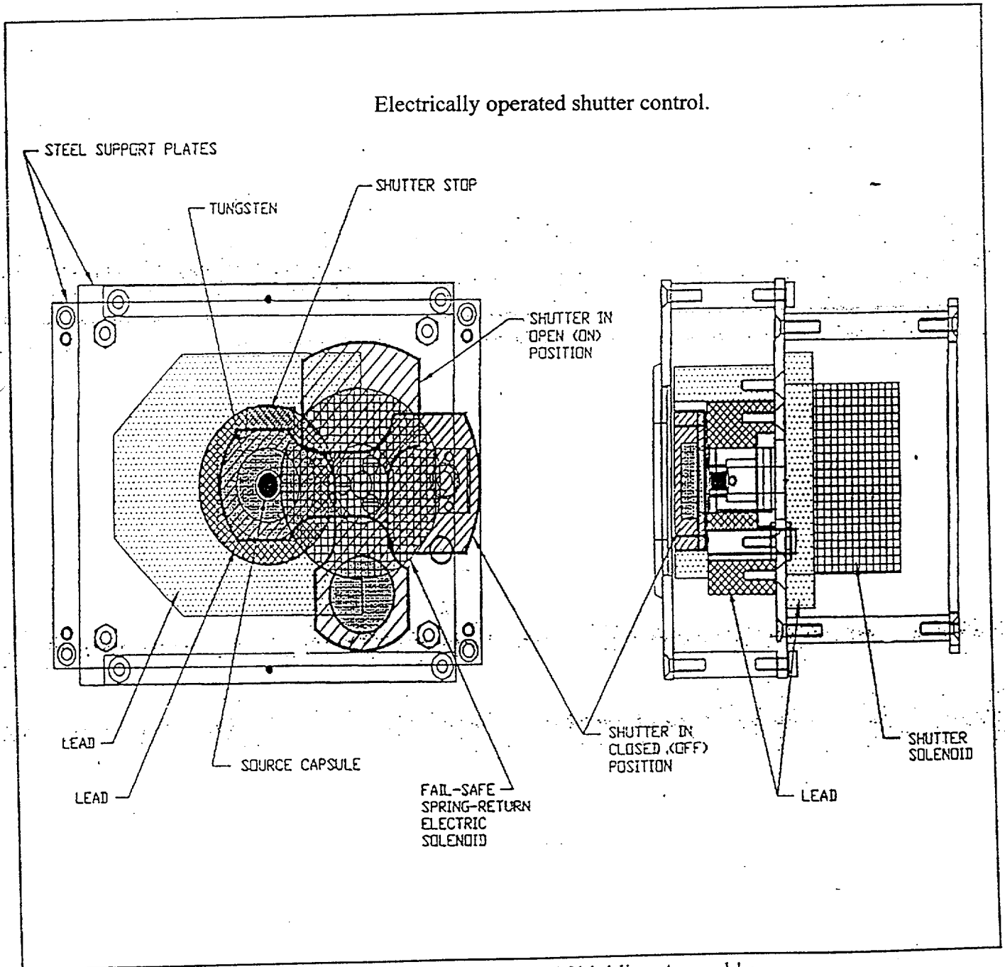
Model 302 Source Holder / Solenoid / Shutter / Shielding Assembly
