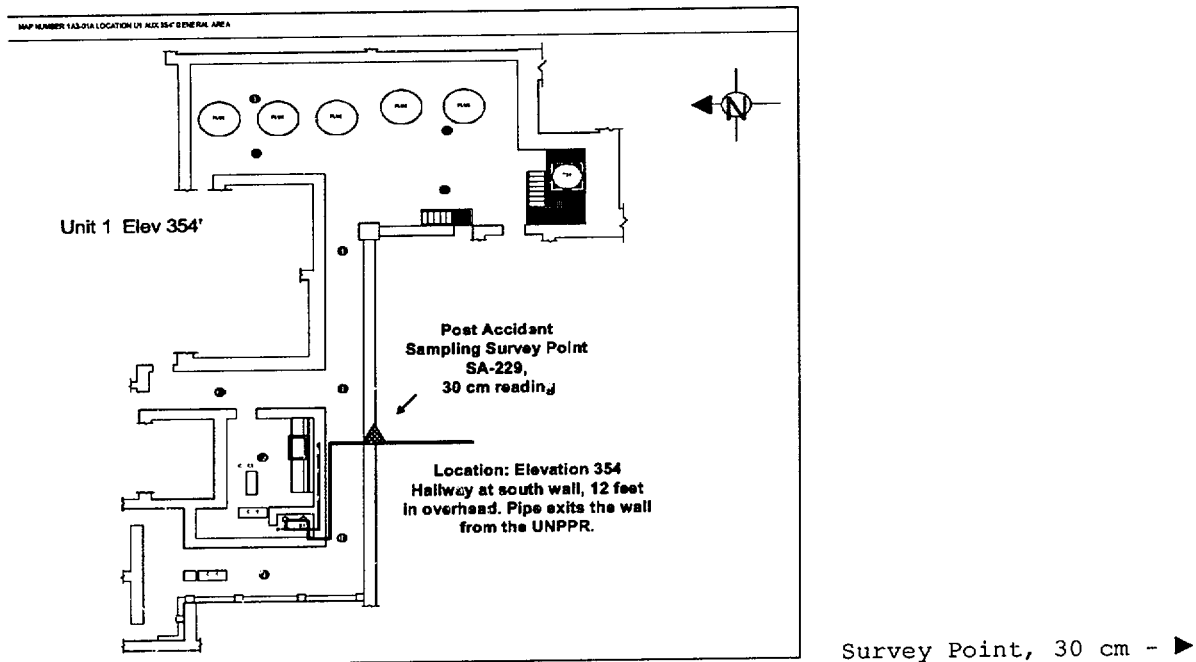
Figure 1 - Unit 1 Elev. 354 Survey Point
