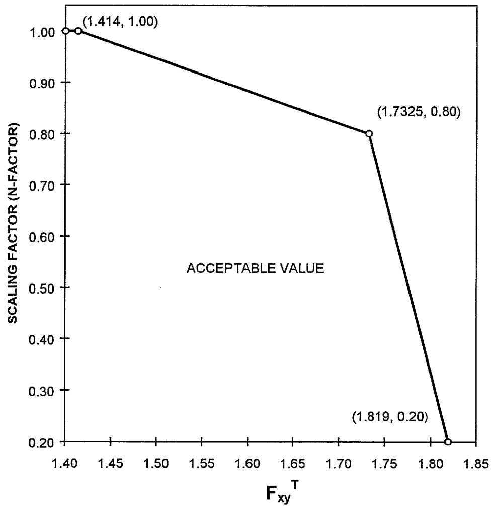
Figure 3.2.1-3 Total Planar Radial Peaking Factor ( F_{xy}^T ) vs. Scaling Factor (N-Factor)
