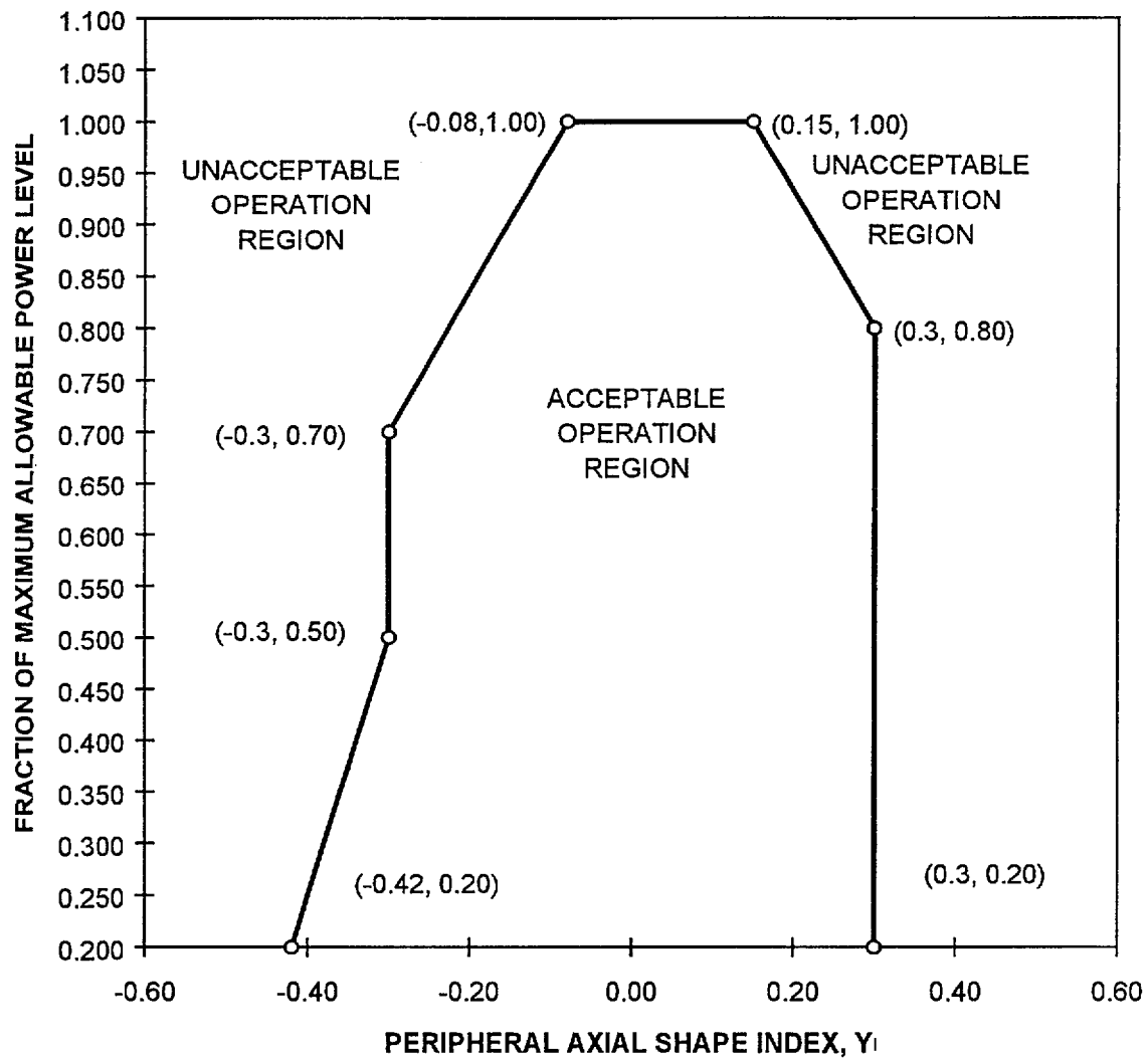
Figure 3.2.5 DNB Axial Flux Offset Control Limits (See NEOP-13 for Administrative Limits)
