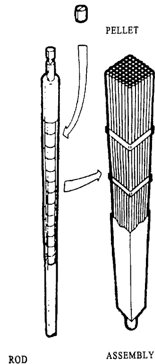
Figure 11: Fuel Pellets, Rods & Assemblies
