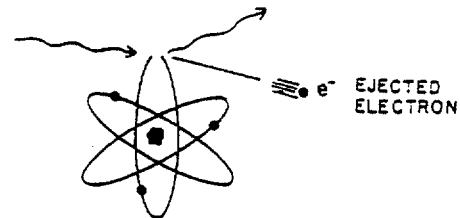
Figure 5: Ionization
