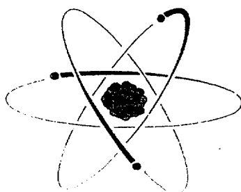
Figure 3: The Atom
