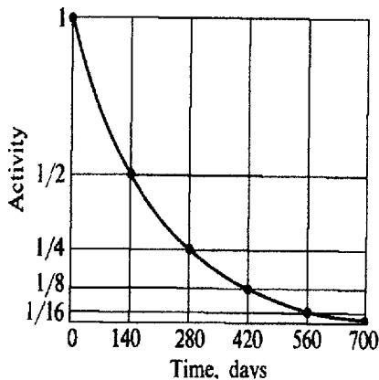
Figure 4: Radioactive Decay
