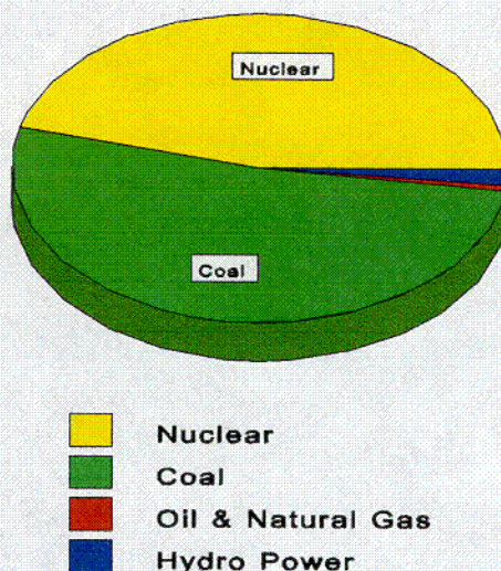
Figure 2: 2001 Energy Sources
