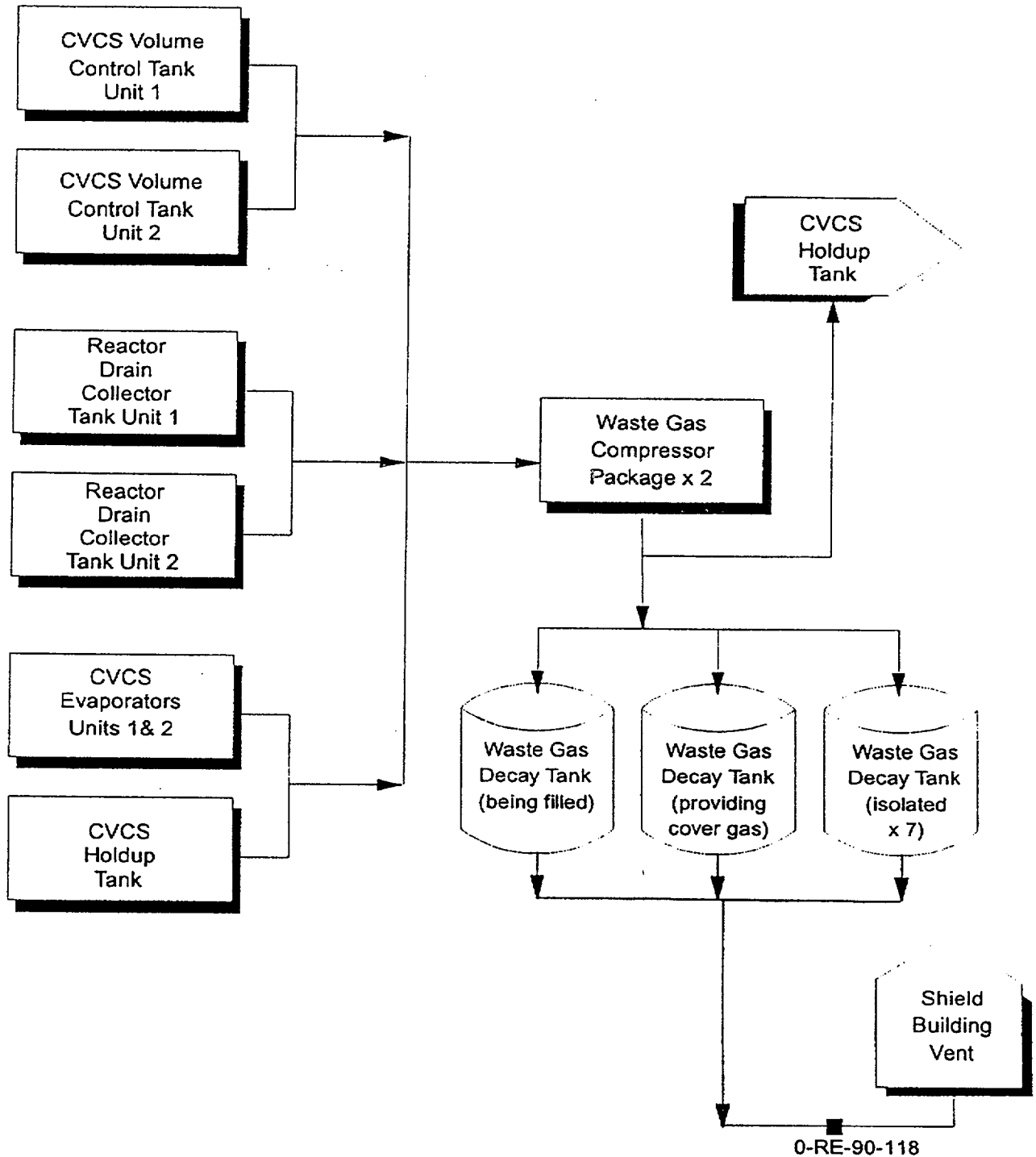
Figure 7.3 - GASEOUS RADWASTE TREATMENT SYSTEM
