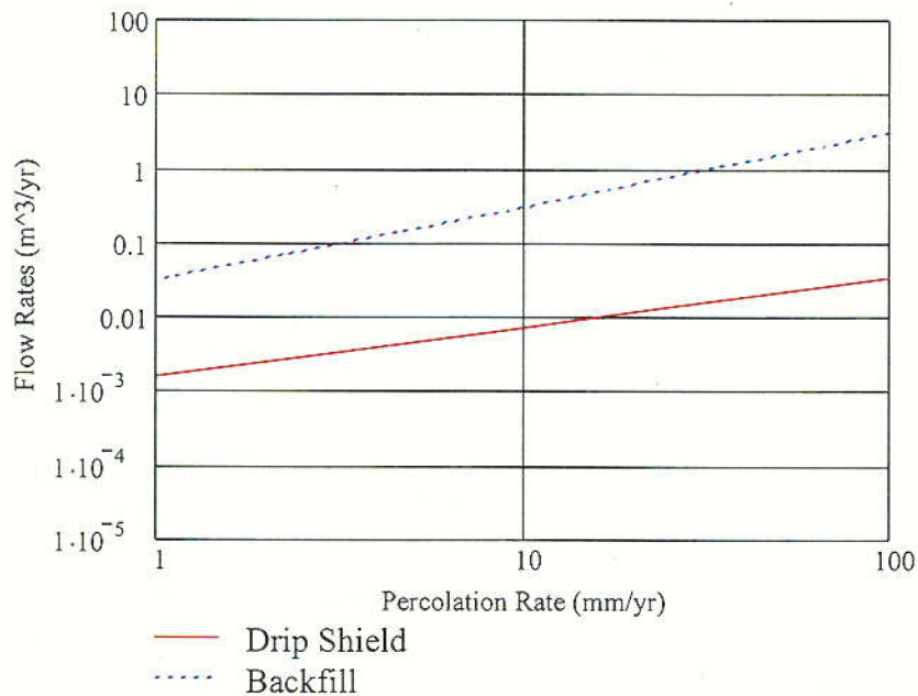
Figure 25. Drip Shield and Backfill Flow Rates as a Function of Percolation Rate
