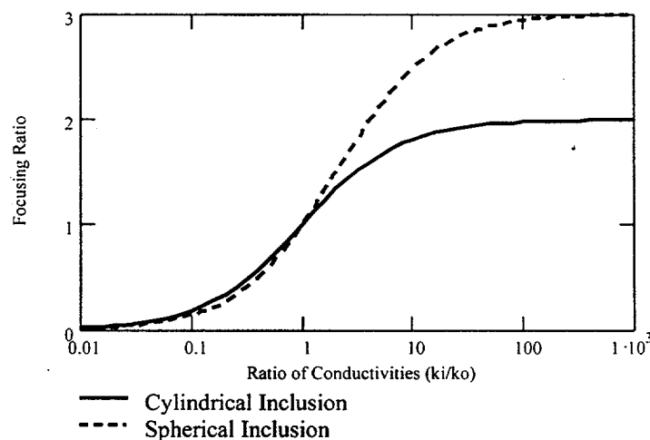
Figure XI-1. The Focusing Ratio or Velocity Ratio for a Sphere of Permeability k_i in a Matrix of Permeability k_o
