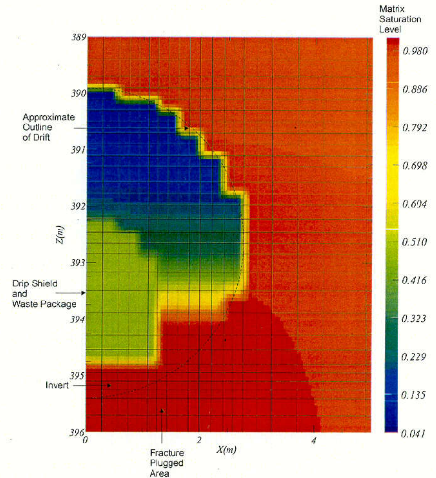
Figure 18. Matrix Saturation Levels for Focused Flow at Steady State at Isothermal Temperature Near the Repository Horizon for Plugged Fractures (Case 5)
