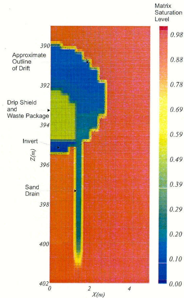
Figure 22. Matrix Saturation Levels for Focused Flow at Steady State at Isothermal Temperature Near the Repository Horizon for Plugged Fractures with a Sand Drain (Case 9)
