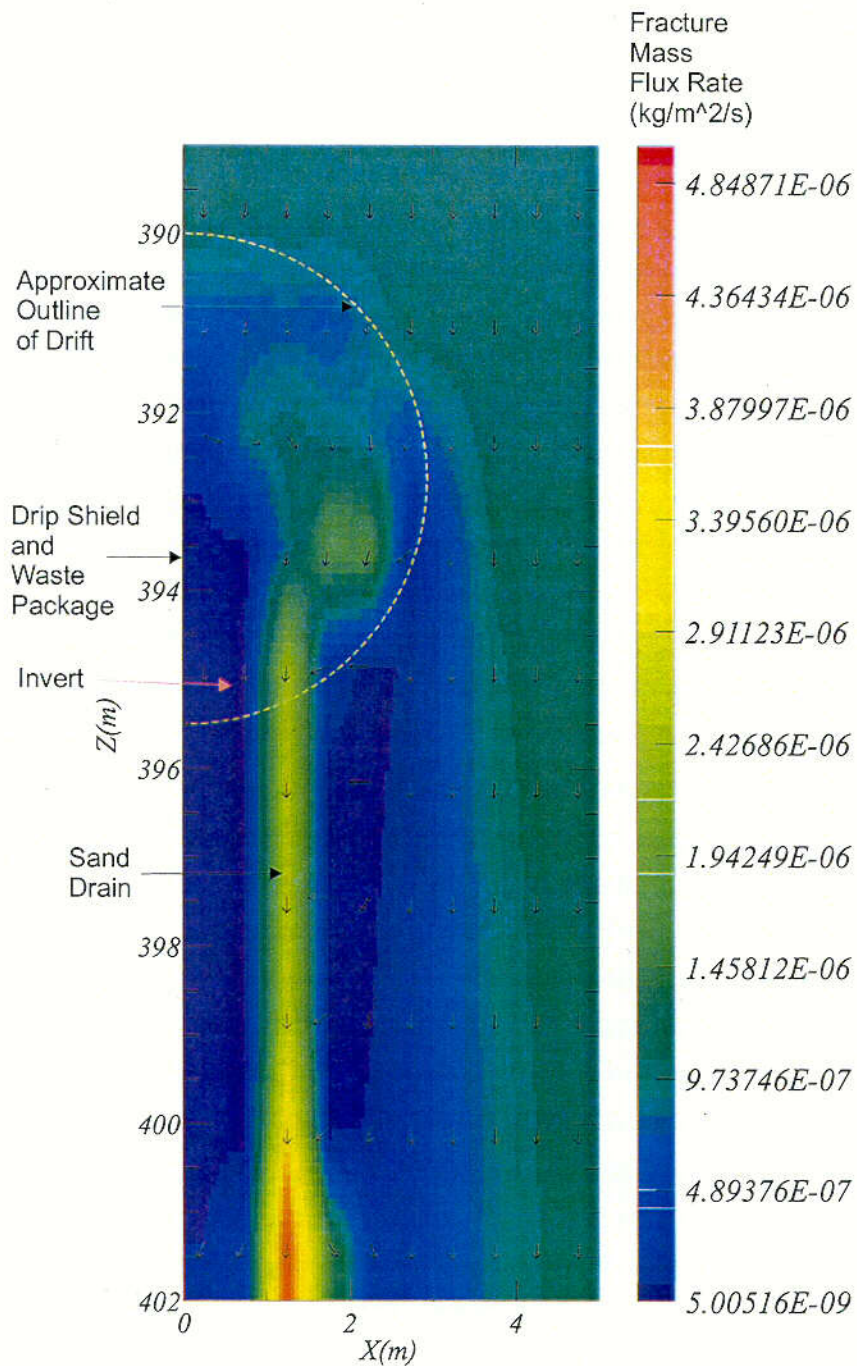
Figure 23. Fracture Mass Flux Rates ( \text{kg/m}^2/\text{s} ) and Direction of Flow for Focused Flow at Steady State at Isothermal Temperature Near the Repository Horizon for Plugged Fractures with a Sand Drain (Case 9)
