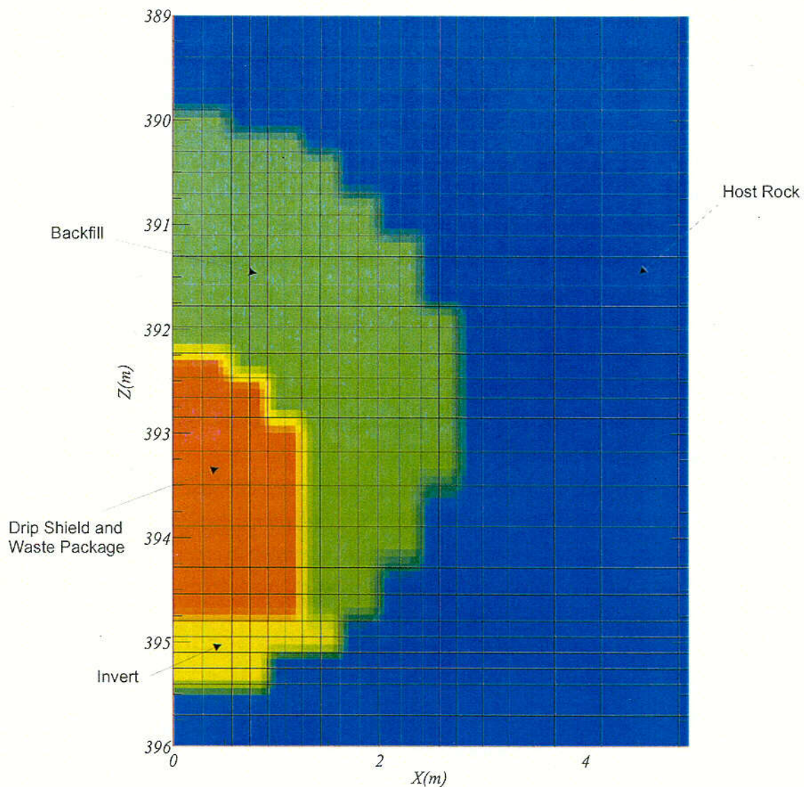
Figure 5. Engineered Barrier Segment Block Model
