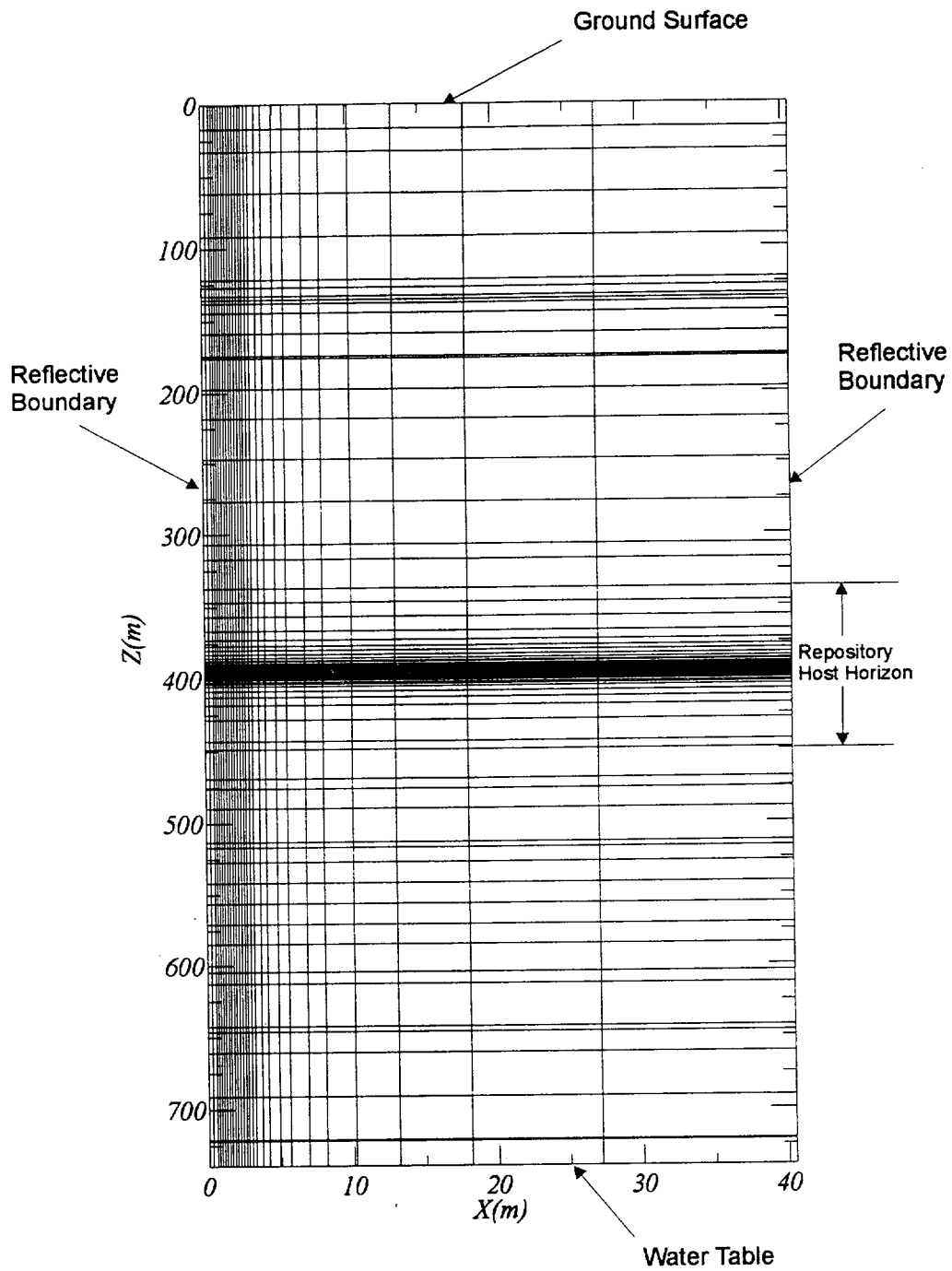
Figure 4. Model Domain and Boundary Conditions
