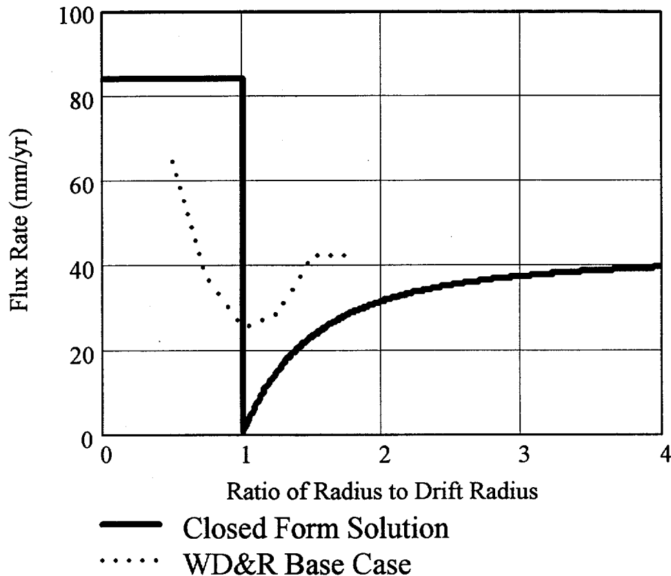
Figure IX-3. Comparison of the NUFT WD&R Model Calculations to the Closed Form Solution
