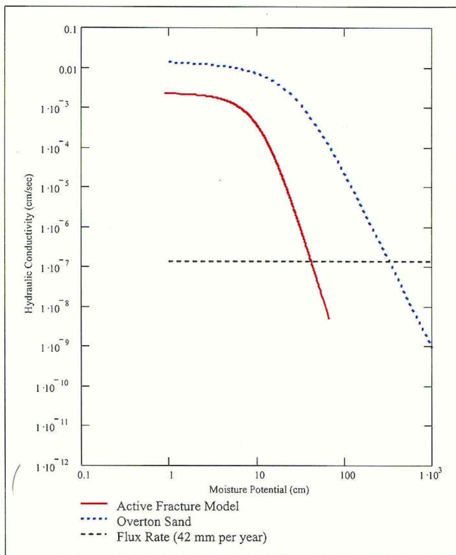
Figure IX-2. Constitutive Properties for the Active Fracture Model, and the Overton Sand
