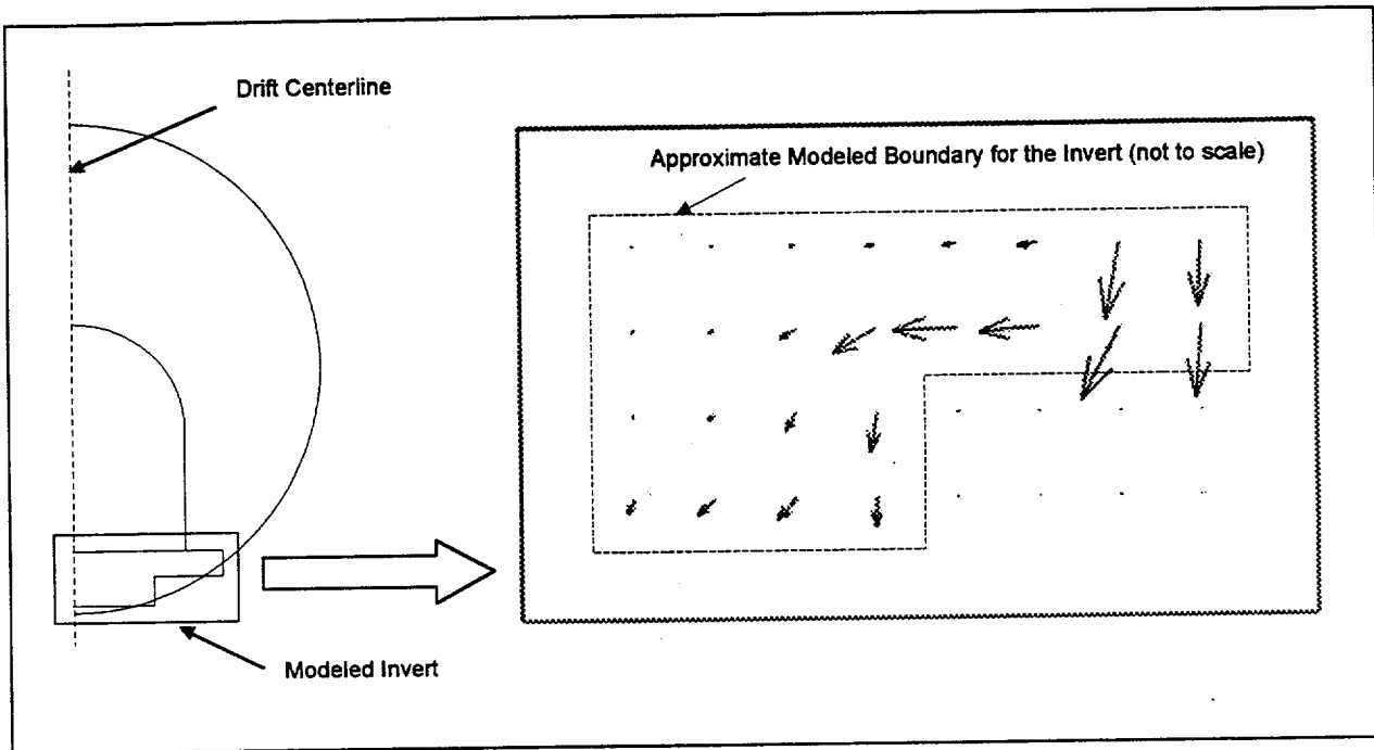
Figure 26. Fracture Pore Water Velocity Vectors in the Invert for the Base Case
