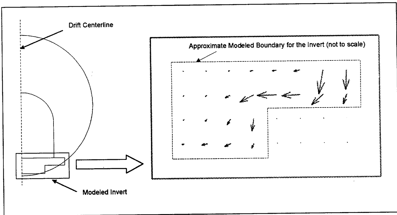
Figure 27. Matrix Pore Water Velocity Vectors in the Invert for the Base Case
