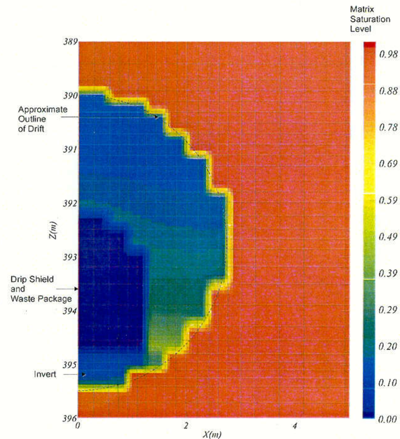
Figure 10. Matrix Saturation Levels for Focused Flow at Steady State at Isothermal Temperature Near the Repository Horizon (Case 1)
