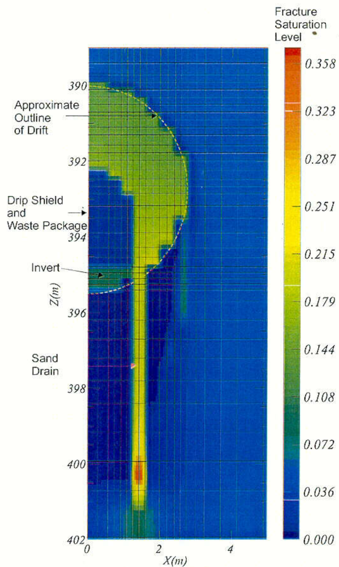
Figure 21. Fracture Saturation Levels for Focused Flow at Steady State at Isothermal Temperature Near the Repository Horizon for Plugged Fractures with a Sand Drain (Case 9)
