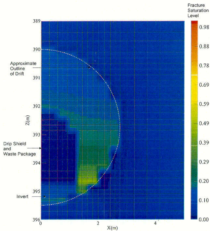
Figure 9. Fracture Saturation Levels for Focused Flow at Steady State at Isothermal Temperature Near the Repository Horizon (Case 1)
