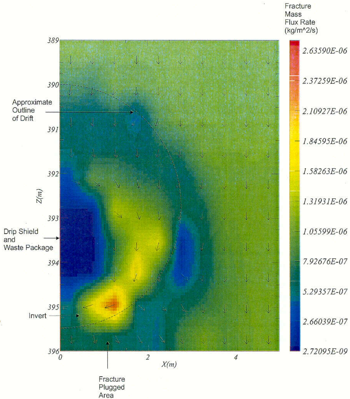
Figure 19. Fracture Mass Flux Rates ( \text{kg/m}^2/\text{s} ) and Direction of Flow for Focused Flow at Steady State at Isothermal Temperature Near the Repository Horizon for Plugged Fractures (Case 5)
