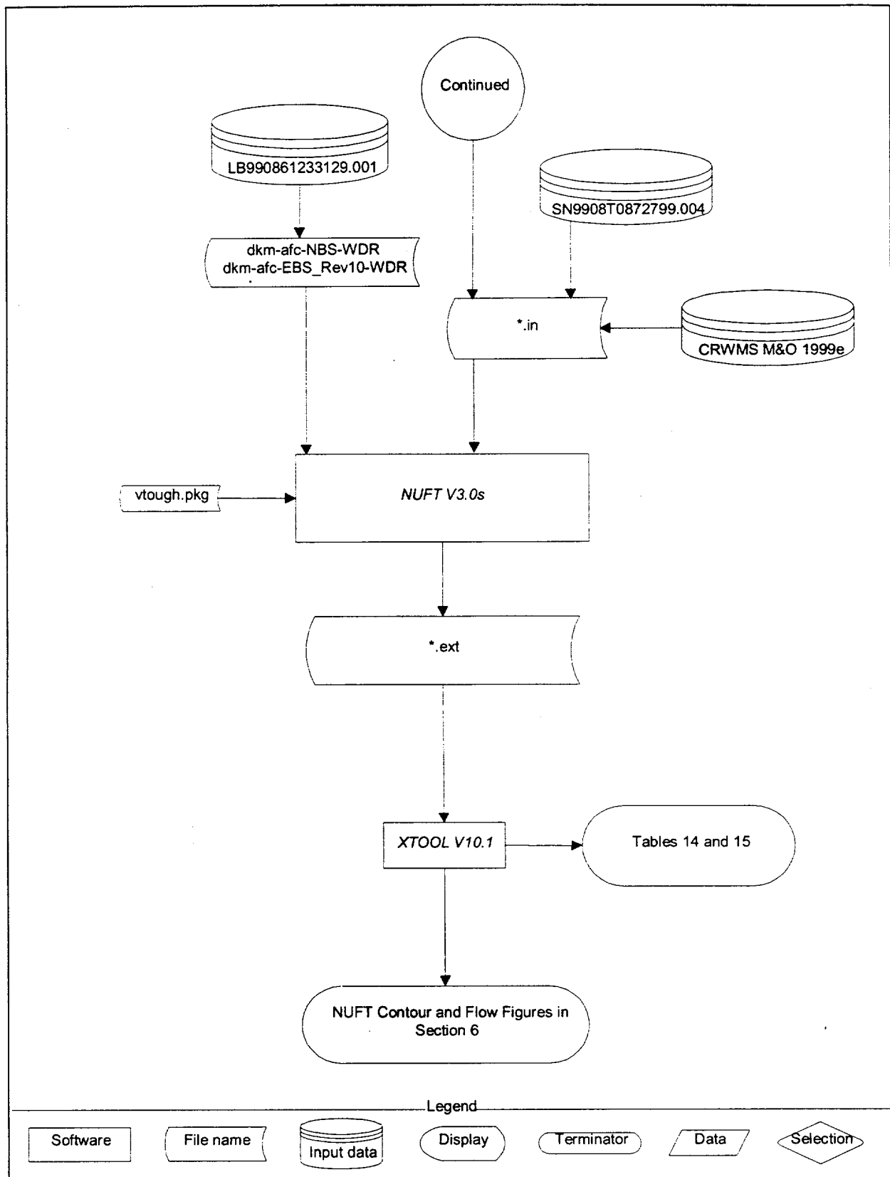
Figure 1. Input Data Manipulation Flowchart (Continued)
