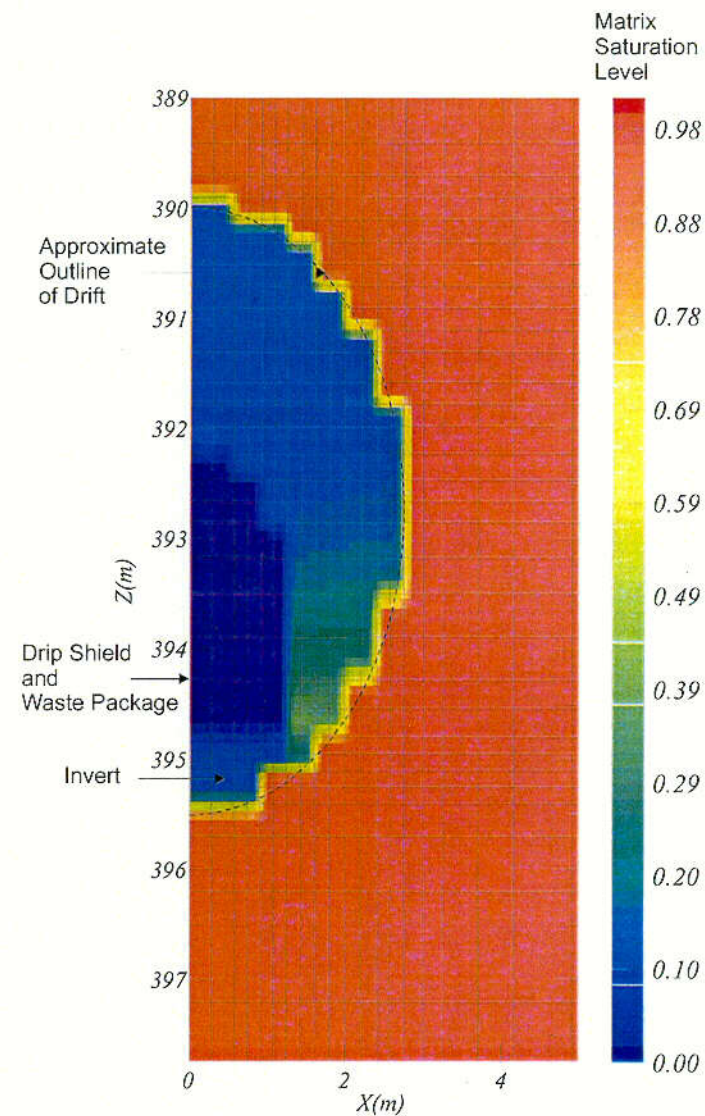
Figure 14. Matrix Saturation Levels for Focused Flow for Repository Heating Near the Repository Horizon After 1,000 Years (Case 3)
