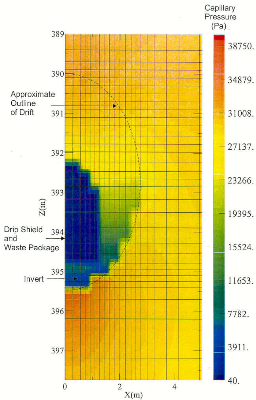
Figure 12. Absolute Matrix Capillary Pressure for Focused Flow for Repository Heating Near the Repository Horizon After 1,000 Years (Case 3)
