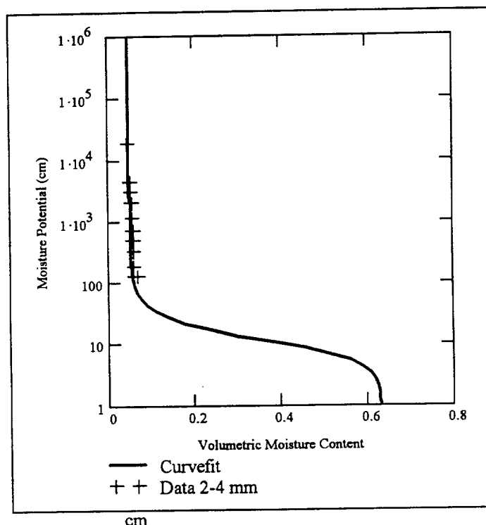
Figure 3. Moisture Retention Relationship for the Invert
