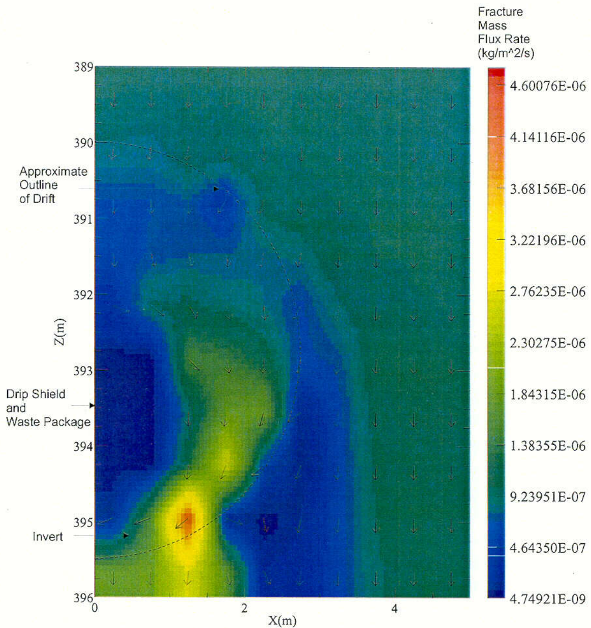
Figure 11. Fracture Mass Flux Rates (kg/m 2 -s) and Direction of Flow for Focused Flow at Steady State at Isothermal Temperature Near the Repository Horizon (Case 1)
