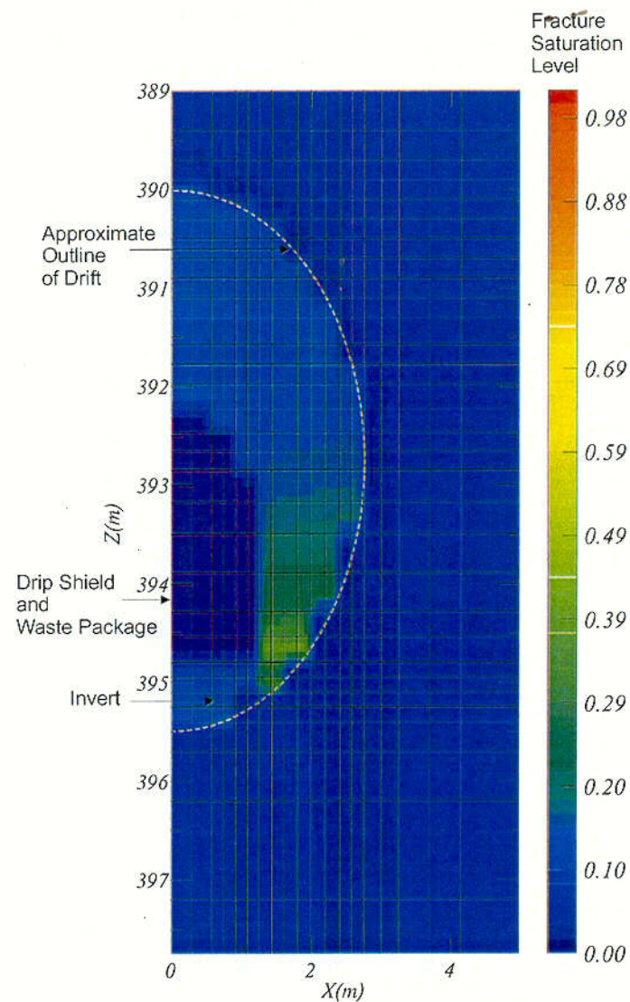
Figure 13. Fracture Saturation Levels for Focused Flow for Repository Heating Near the Repository Horizon After 1,000 Years (Case 3)
