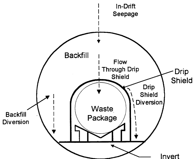
Figure 2. Conceptual Model for Diversion of Water Flow
