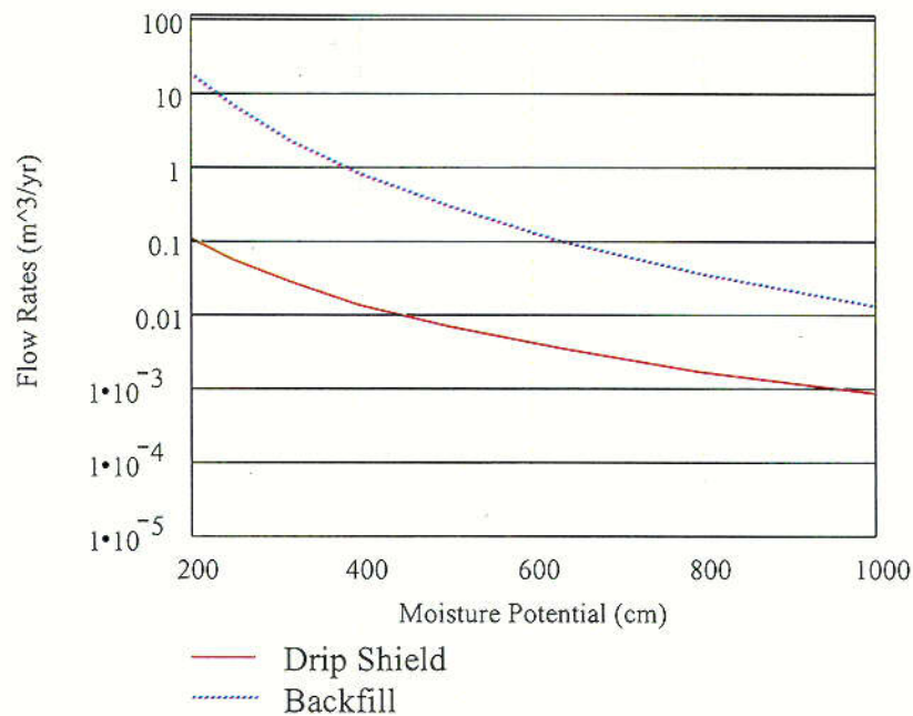
Figure 24. Drip Shield and Backfill Flow Rates as a Function of Moisture Potential
