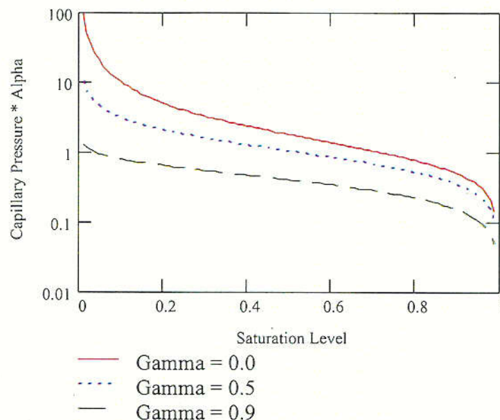
Figure 6. Influence of the Parameter Gamma on Retention
