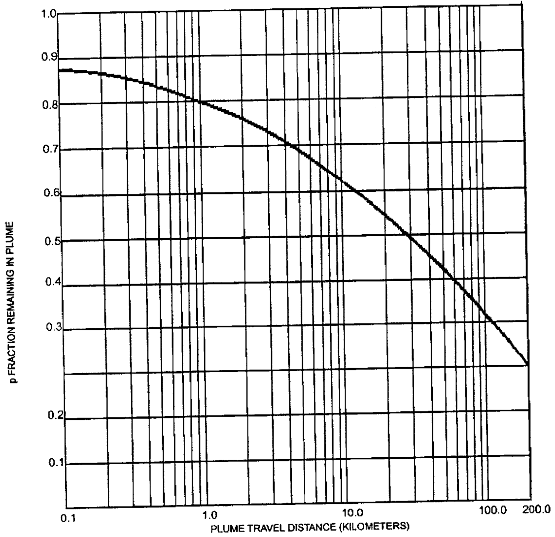
Plume Depletion Effect for Ground-Level Releases (All Stability Classes)
