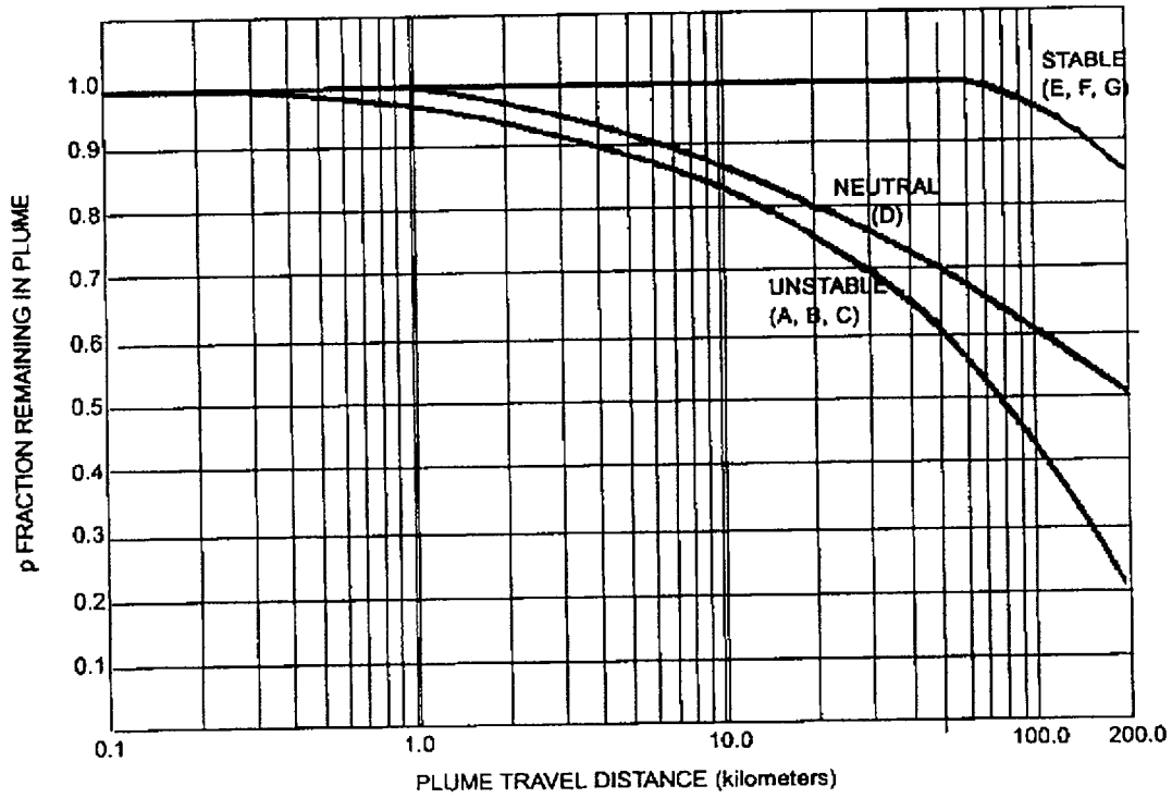
Plume Depletion Effect for 60 meter Releases (Letters denote Pasquill Stability Class)
